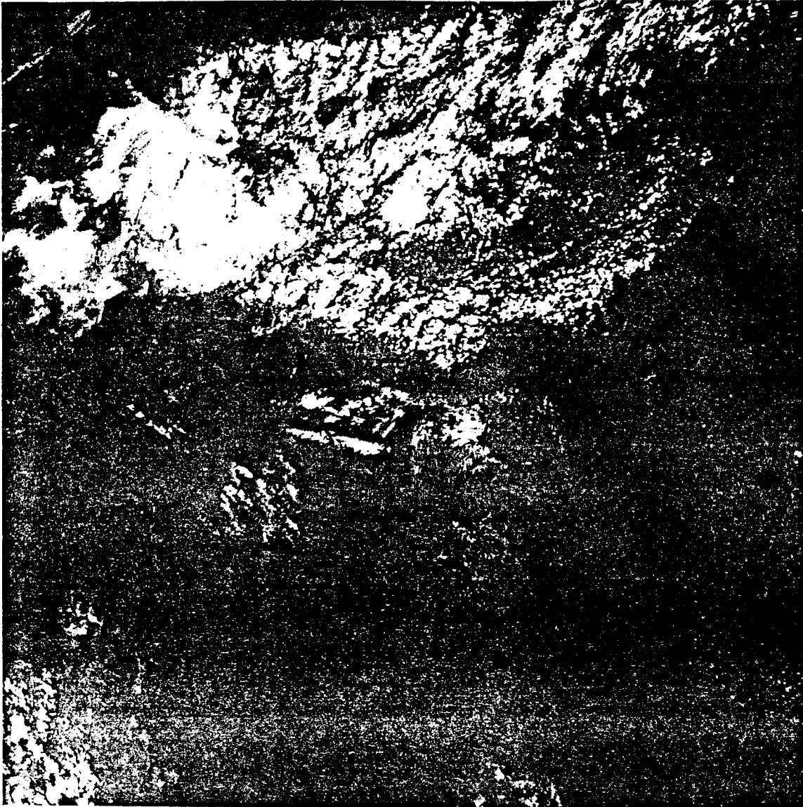
(d) Western half of Taiwan (Formosa) and Pescadores Islands, looking east. China coast and Haitan Tao Island are at lower left.
