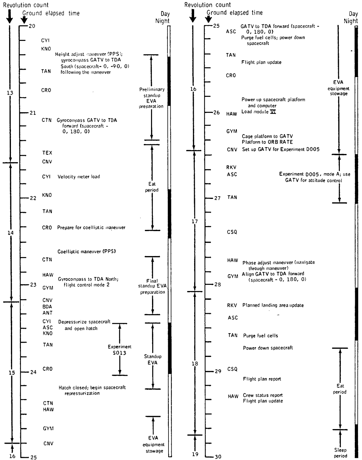
(c) 20 to 30 hours g.e.t.
