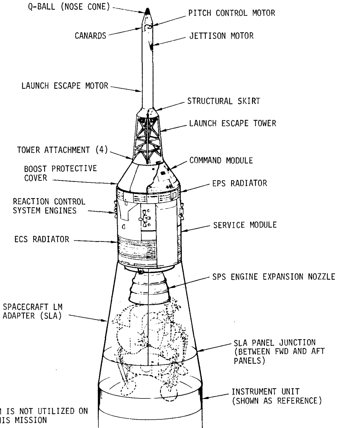
SPACECRAFT CONFIGURATION
