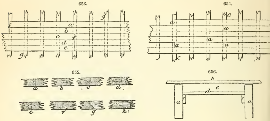
Fig. 655 shows the various ways of joining floor-boards : a , plain joint; b , ploughed and tongued; c , rebated; d , e , with a tongue of wood or iron inserted; f , with the tongue resting on the joist; g , h , splayed.
