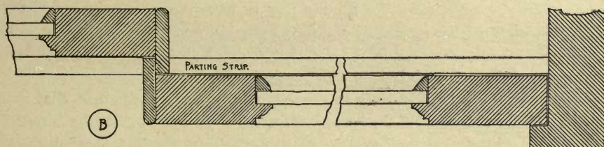
MEETING STILES OF SLIDING DOORS.
