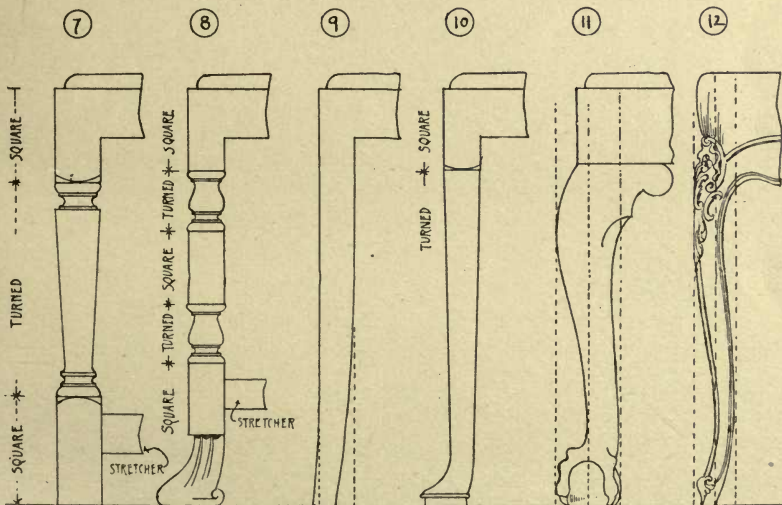
ELEVATIONS
