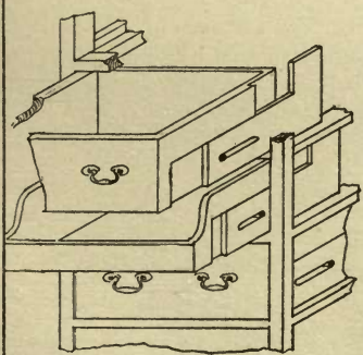
SECTION THROUGH FRONT.
