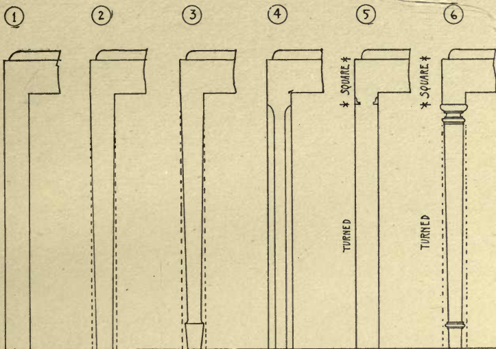
ELEVATIONS
