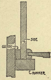
SECTION THROUGH BACK AND SIDE.
