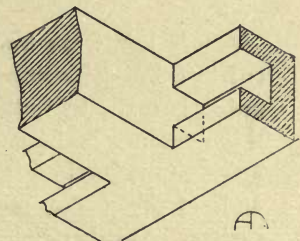
STUB TENON
