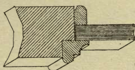
GLASS FULL SIZE AS A PANEL
