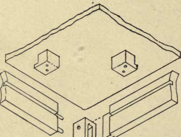
FRAME DOWELED TO THE LEG
