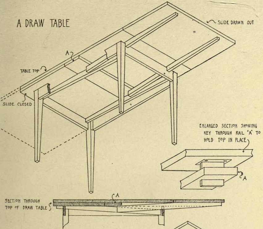
COMMON FORM OF EXTENSION TABLE
