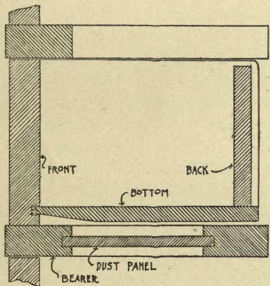
SECTION THROUGH FRONT.
