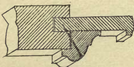
JOINERS METHOD.
