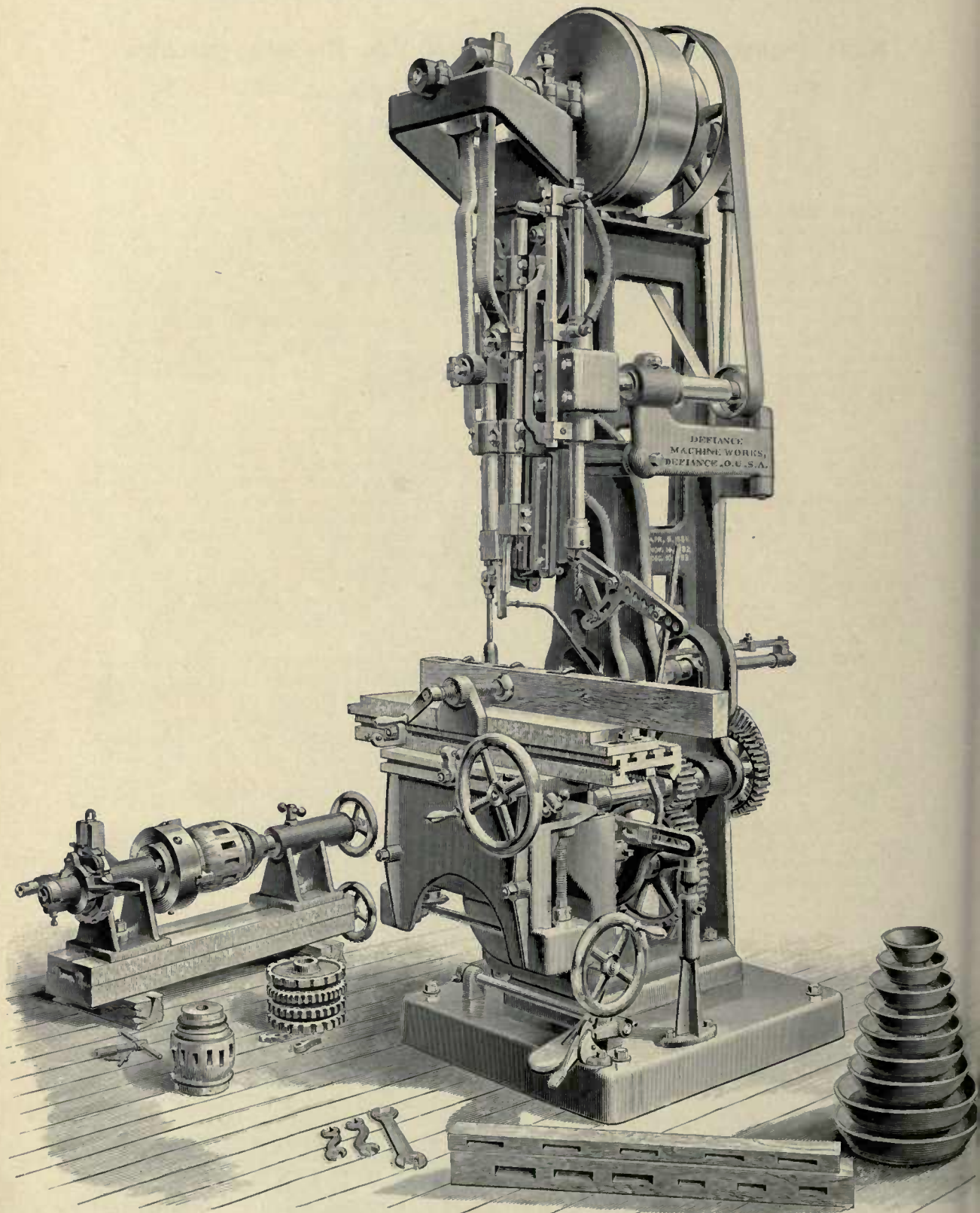
No. 1 \frac{1}{2} Patent Double Chisel Combined Hub and Plain Mortising Machine.
