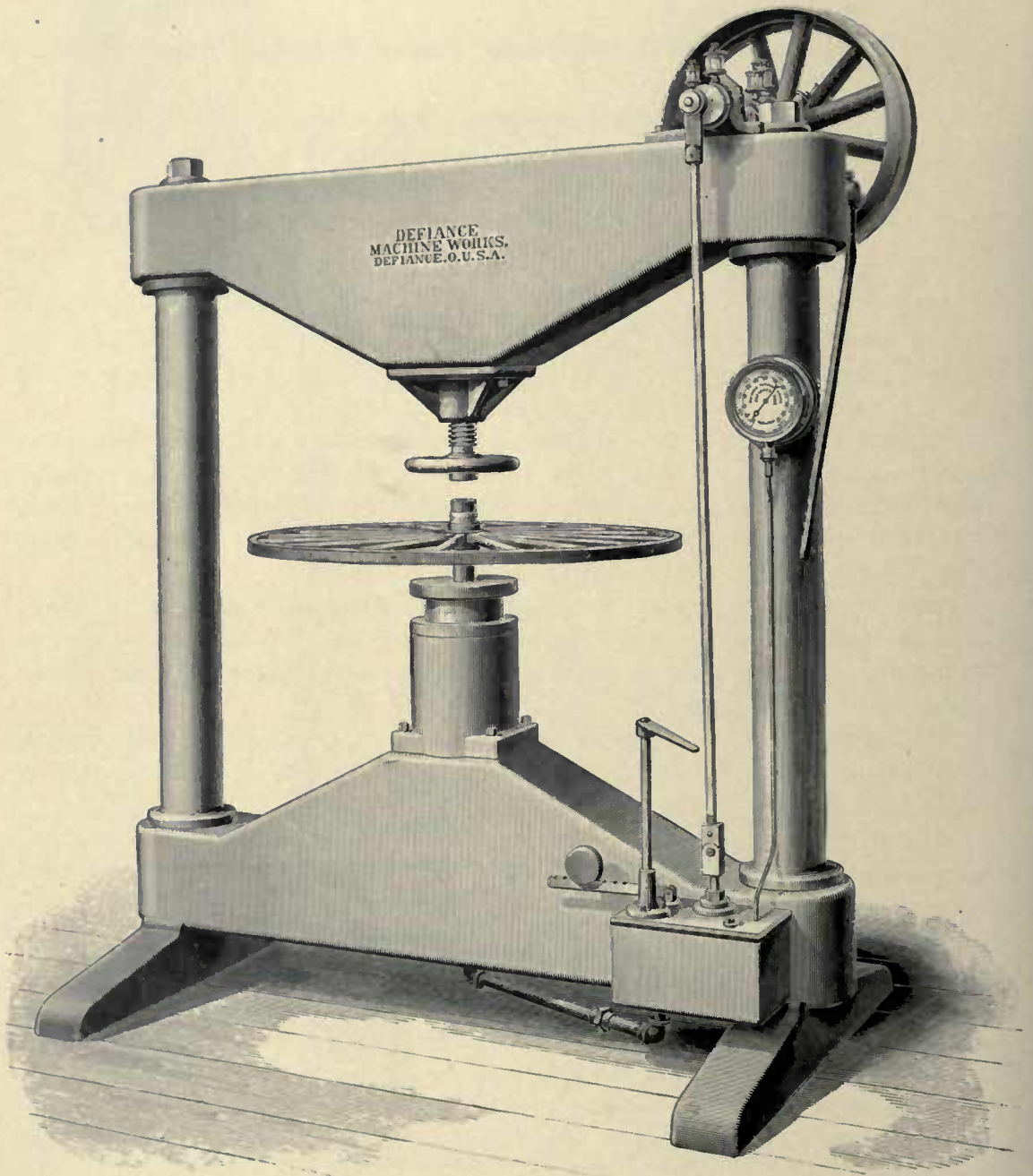
No. 2 Patent 60-Ton, Iron Frame, Hydraulic Wheel Press.
