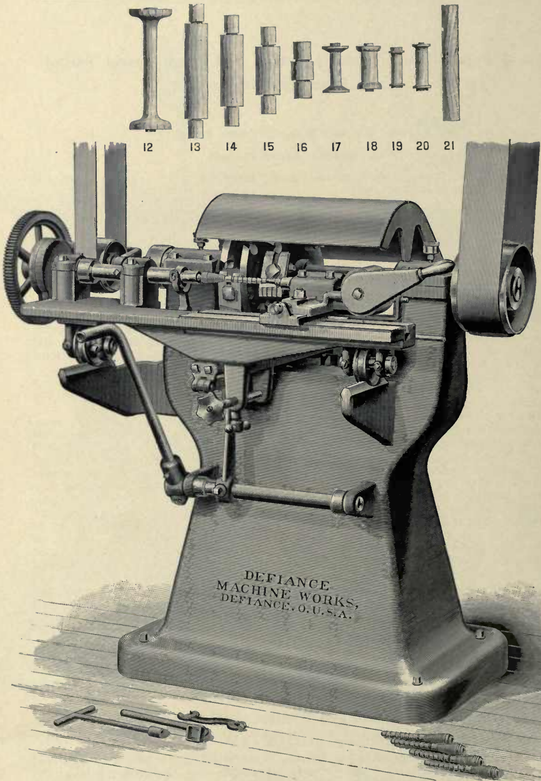
No. 3 Patent Bobbin and Spool-Barrel Turning Lathe. Export Shipping Weight, 2,000 Pounds. Net Weight, 1,600 Pounds. Cubic Measurement, 66 Feet. Cable Word, LONESTAR.
