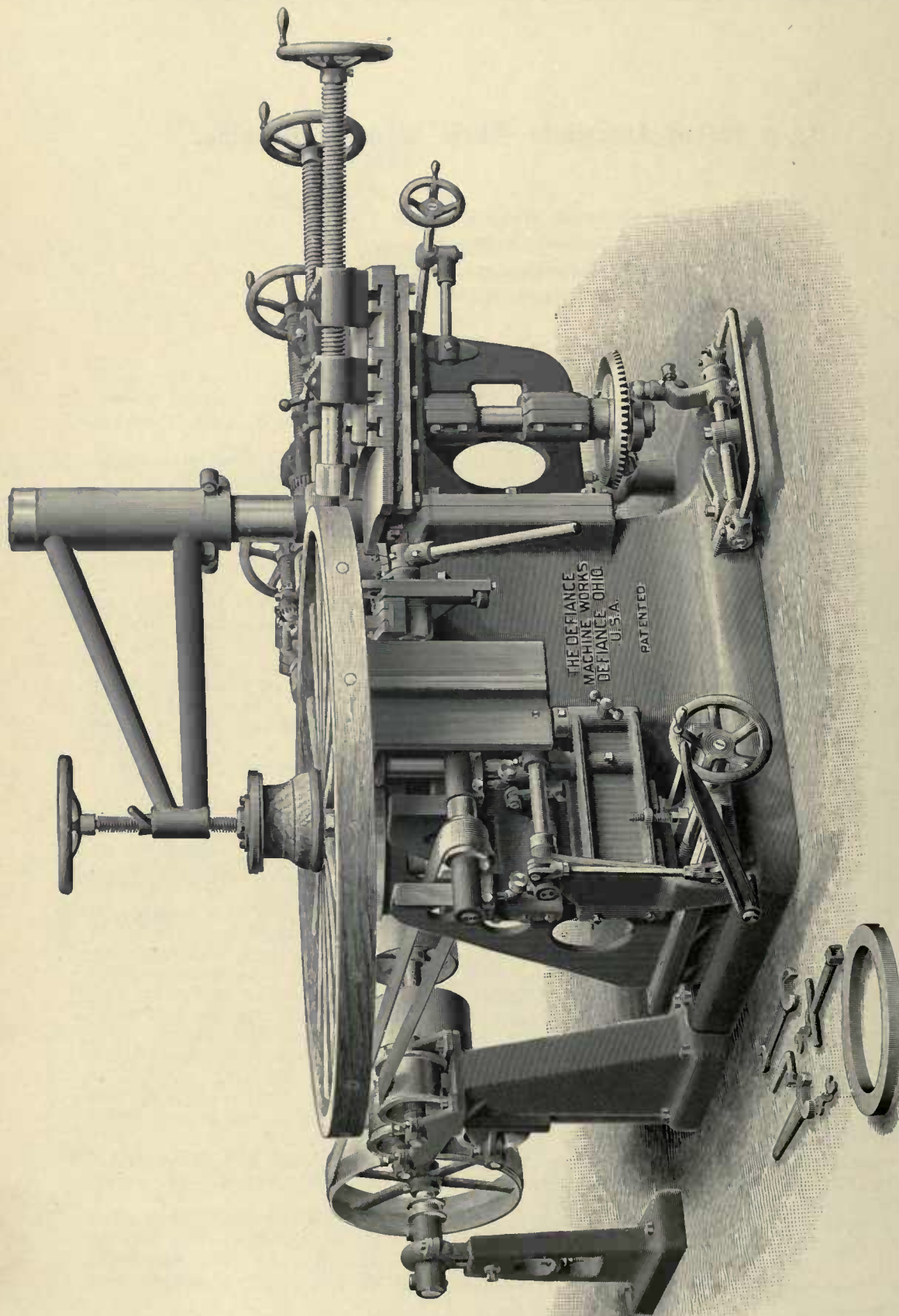
No. 4 Patent Automatic Wheel Rimming Machine.
