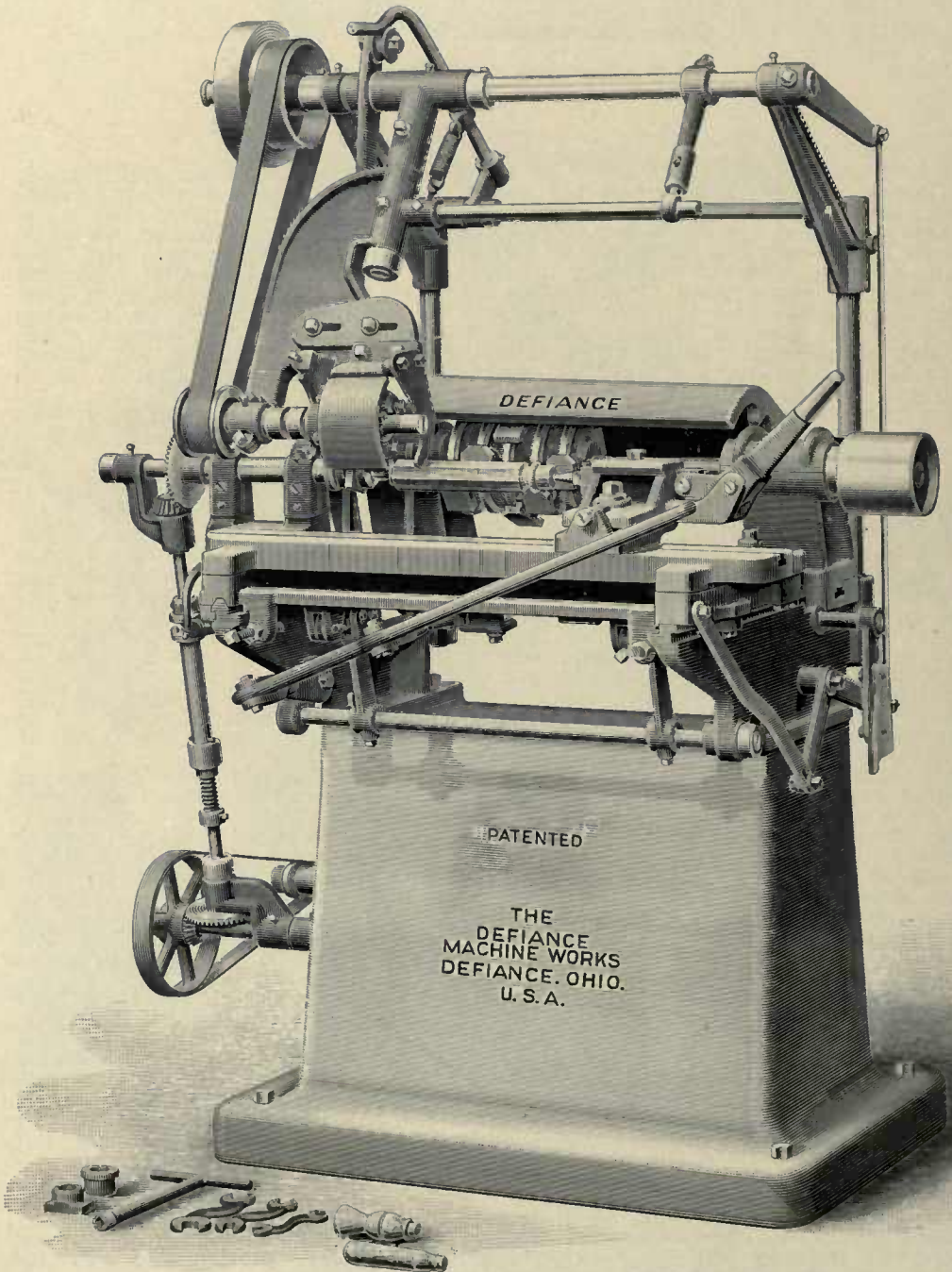
No. 444 Patent Automatic Turning Lathe. Export Shipping Weight, 1,900 Pounds. Net Weight, 1,400 Pounds. Cubic Measurement, 74 Feet. Cable Word, LEBIR.
