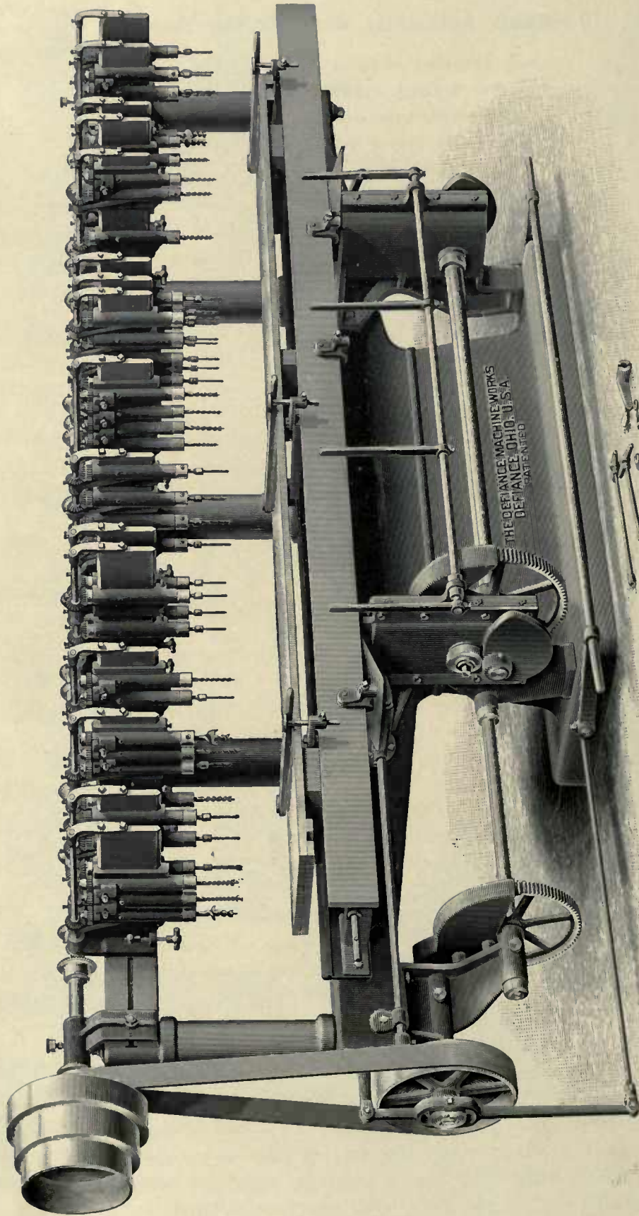
No. 12 Patent Automatic Wagon-Box Boring Machine.
