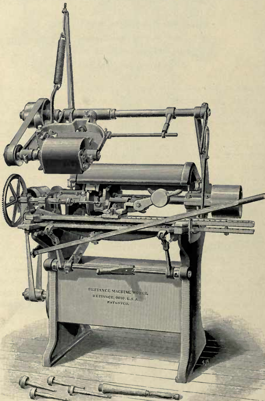
24" Patent Automatic Handle Lathe.
