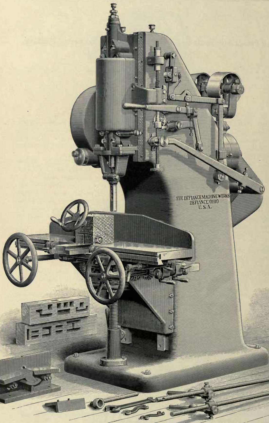
No. 1 Patent Automatic Vertical Hollow Chisel Mortising Machine.
