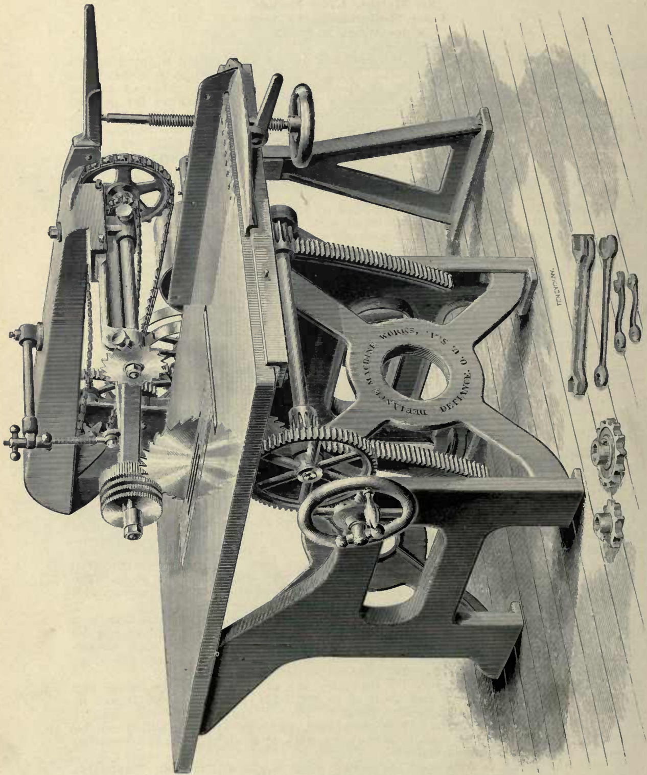
No. 2 Patent Heavy Power Feed Rinning Saw
