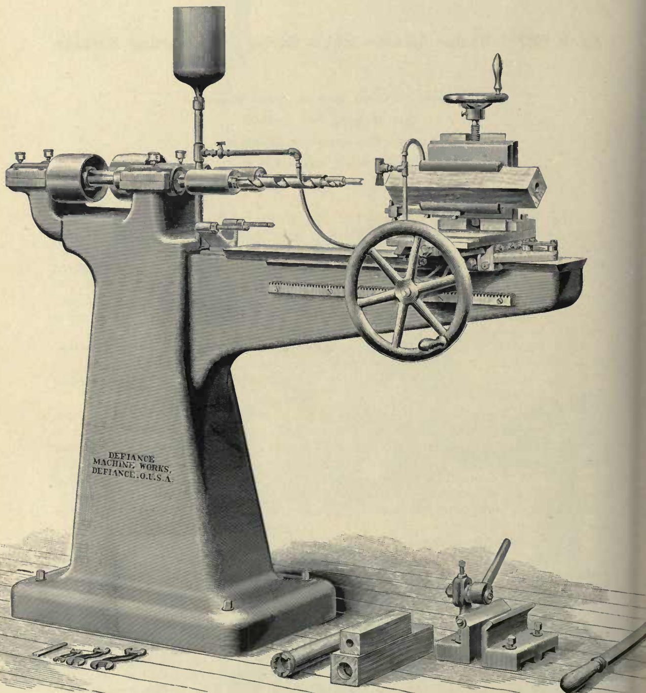
No. 4 Patent Double Spindle Bobbin and Spool Barrel Boring and Reaming Machine.
