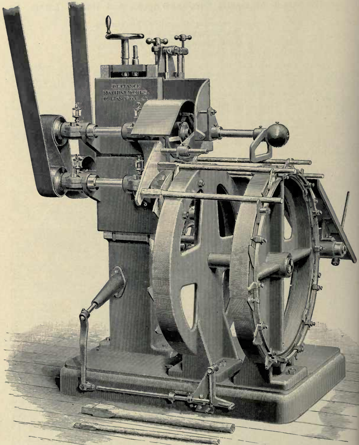
No. 1 Patent Automatic Double Spoke Tenoning, Mitering, and Pointing Machine.
