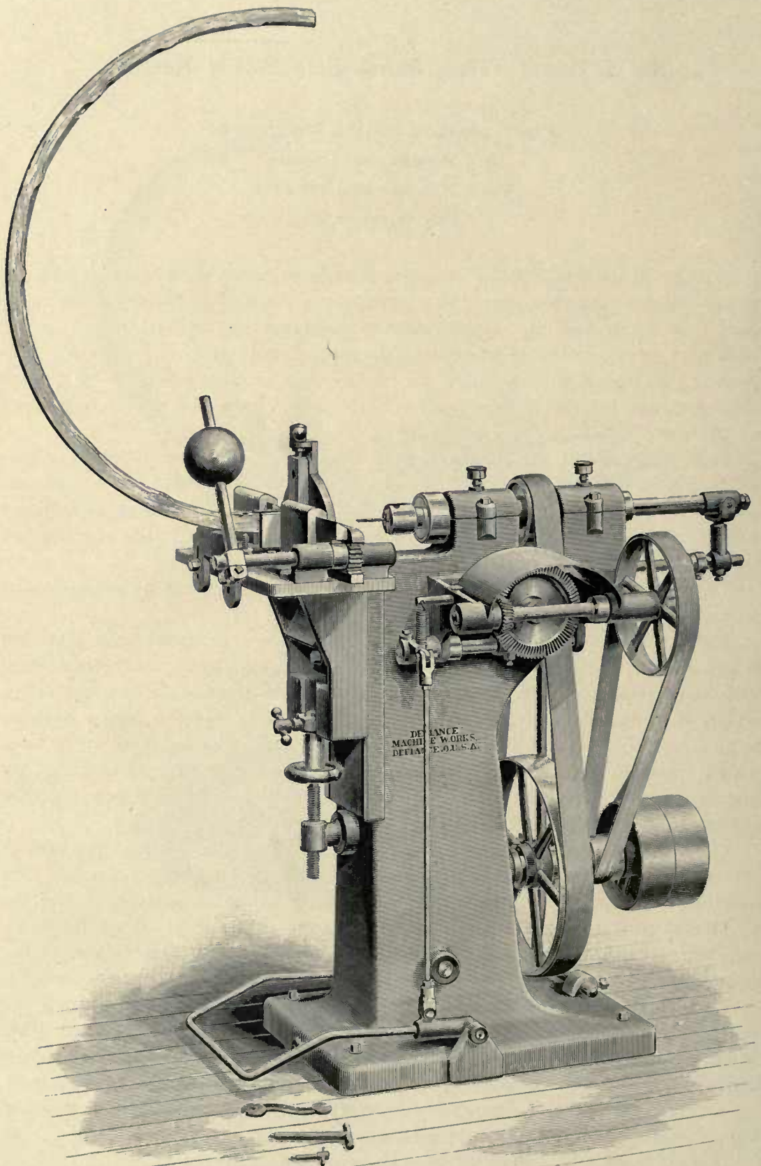
No. 2 Patent Automatic Felloe Dowel Hole Boring Machine. Export Shipping Weight, 1,100 Pounds. Net Weight, 900 Pounds. Cubic Measurement, 38 Feet. Cable Word, BEBE.
