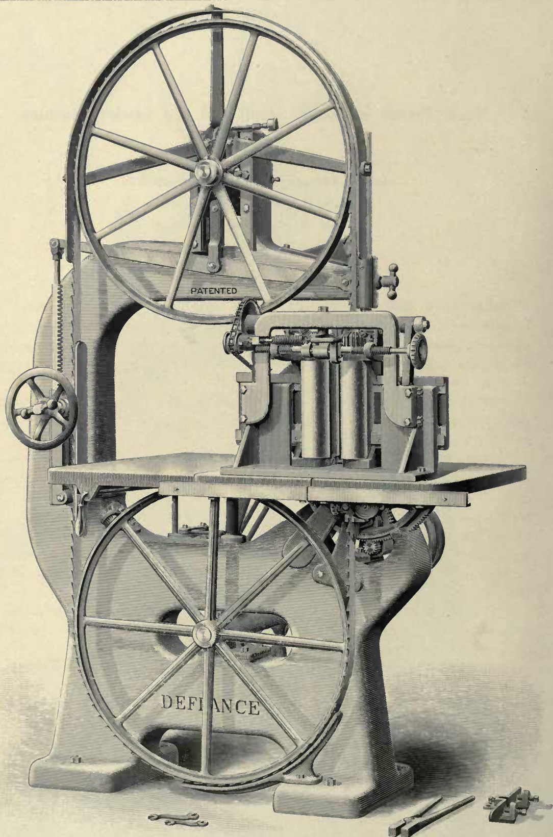
No. 9 Patent Heavy Band, Scroll, Rip and Re-sawing Machine.
