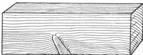
FIG. 49.--Showing risk of knots on underside of loaded beams.
