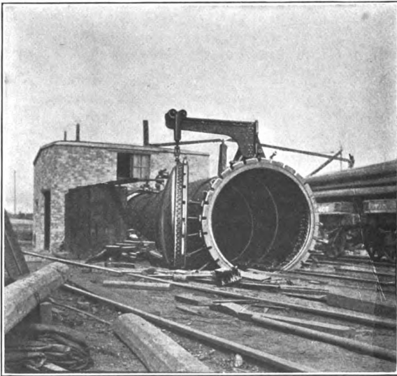
FIG. 40.—Creosoting Tank empty.
