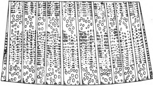
FIG. 10.—Cross section of Oak, magnified about five times. (After Roth.)
