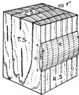
FIG. 3.—Block of Oak. C. S., cross section; R. S., radial section; T. S., tangential section; m. r. , medullary rays; a , height; b , width; e , length of med. ray. (After Roth.)
