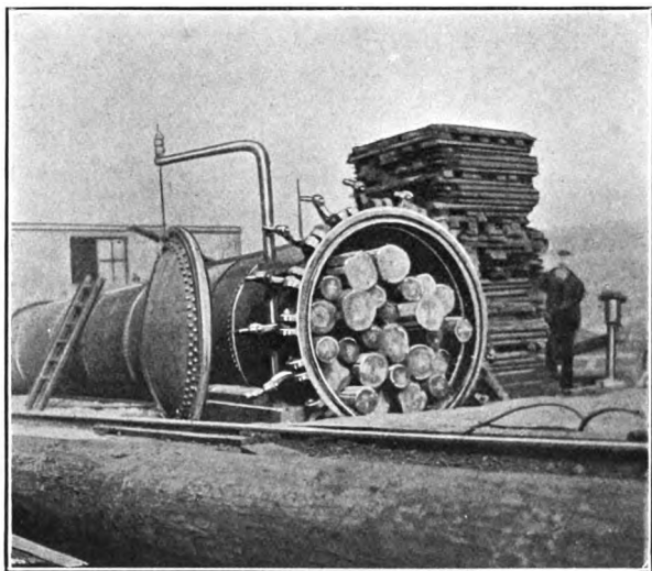
FIG. 41.—Creosoting Tank filled with Poles.
