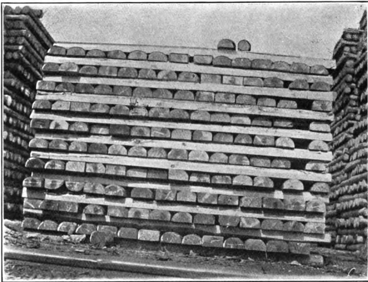
FIG. 38.—Showing Method of Stacking Sleepers for Seasoning.
