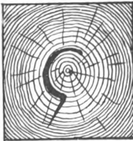
FIG. 47.—Cupshake often found in pitch pine.
