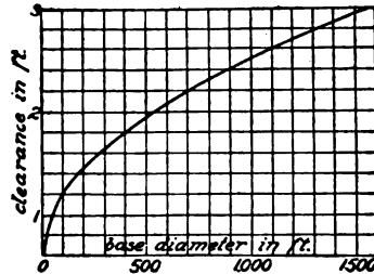
Fig. 30. Reservoir Clearance.
