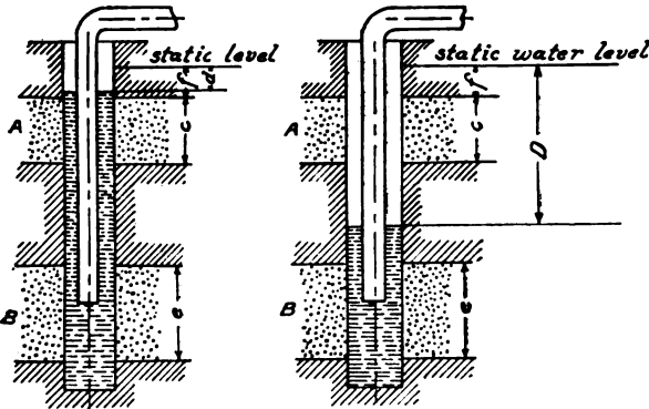
Fig. 20. Water at A and B. Fig. 21. Water between A and B.
