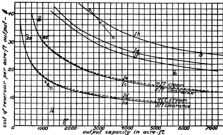
Fig. 49. First Costs of Artificial and Natural Reservoirs.
