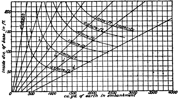
Fig. 38. Capacities and Volumes of Embankment. Case 2.
