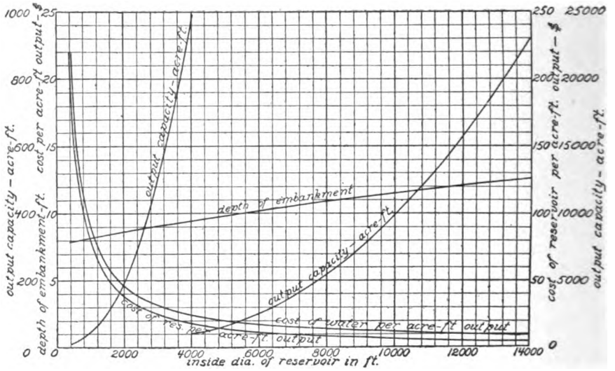
Fig. 45. Economic Reservoir Dimensions and Costs. Case 1a.
