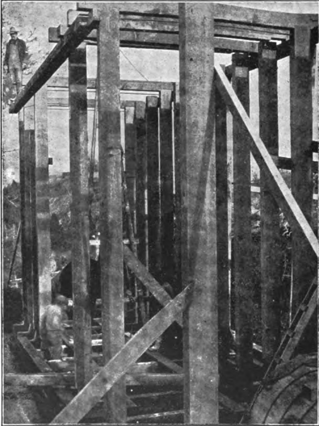
Fig. 7. Laying Wooden Pipe.
