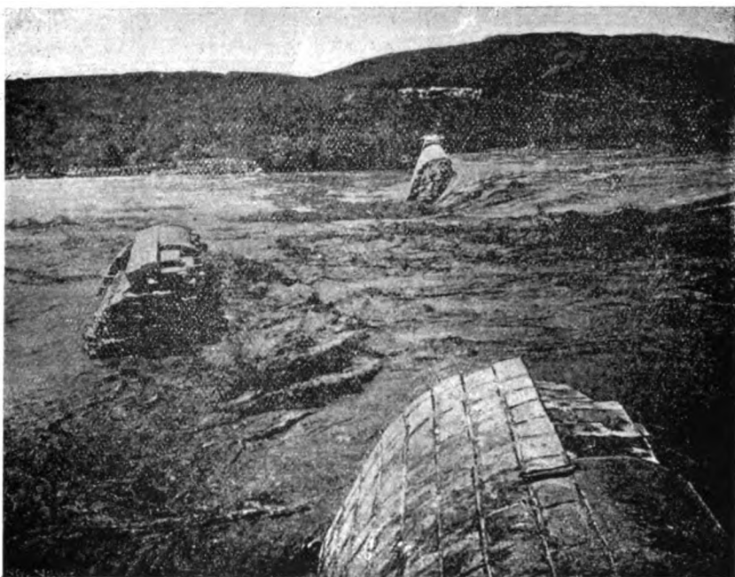
Plate II (a). Austin Dam, Texas. View taken during flood a few minutes after the break.
