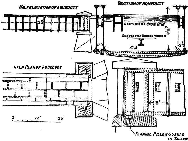
Fig. 74. Manjanar Aqueduct.
