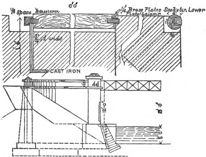
Fig. 91. Towpath Roller.
