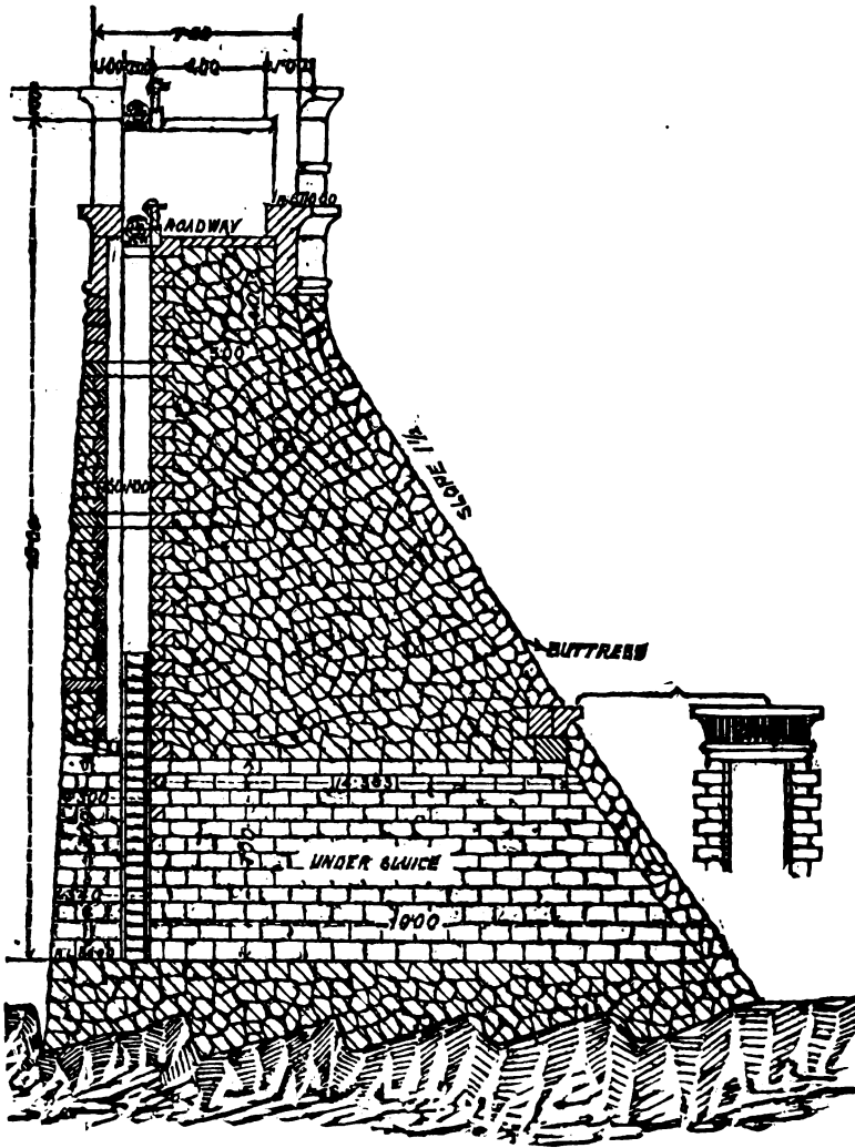
Fig. 127. The Nile Dam at Assuán.
