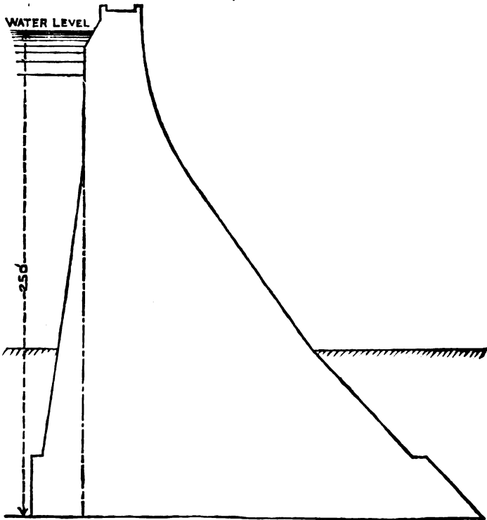
Fig. 116. Quaker Bridge Dam.
