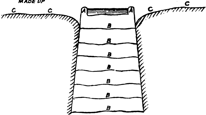
Fig. 96. Puddle wall.
