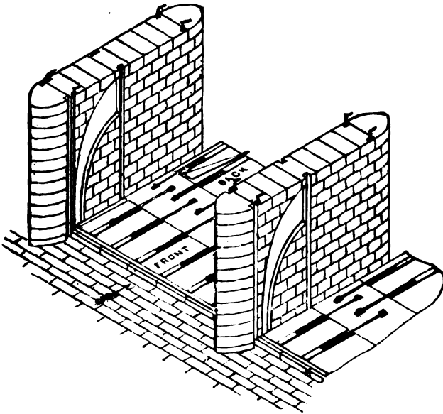
Fig. 39. Fouracres' Shutter Open.
