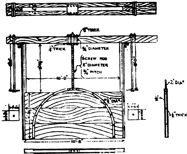
Fig. 55. Details of Shutter.
