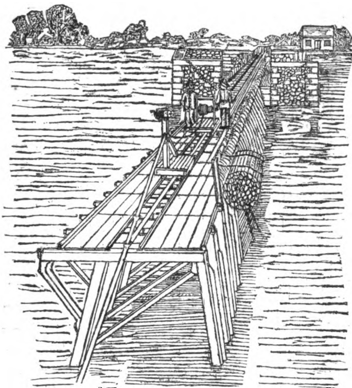
Fig. 33. Moveable Weir.
