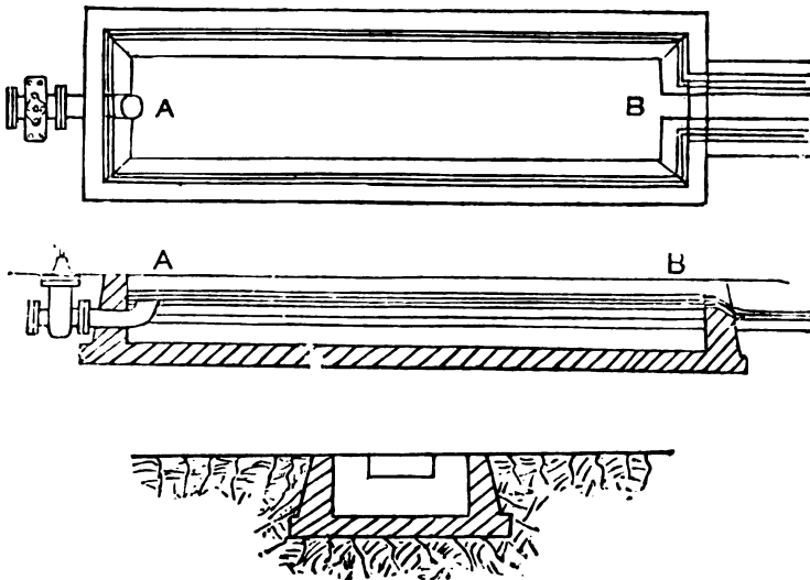
Fig. 149. "Canal" sand washer in plan and sections.
