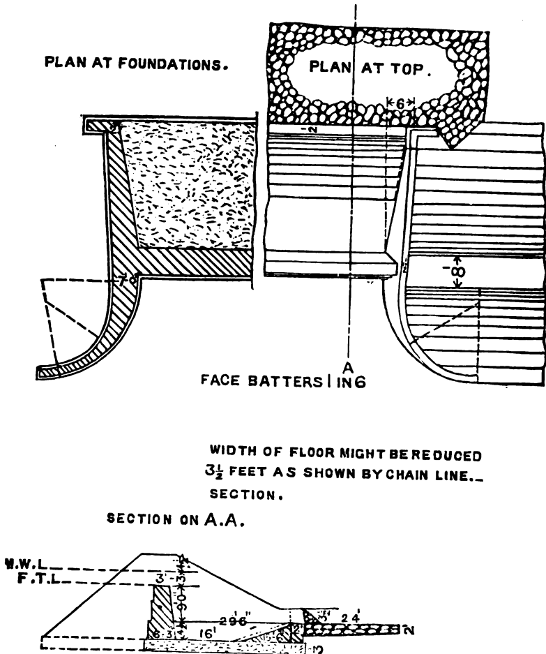
Fig. 110. Surplus Weir with Water Cushion.
