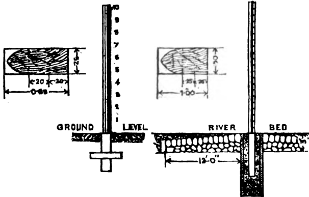
Fig. 2. River Gauge.
