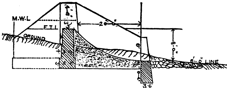
Fig. 111. Weir with curved apron.
