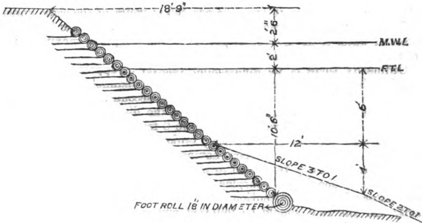
Fig. 106. Nanel or Durbah Revetment.
