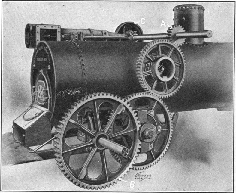
FIG. 172.—Traction-engine gearing.
