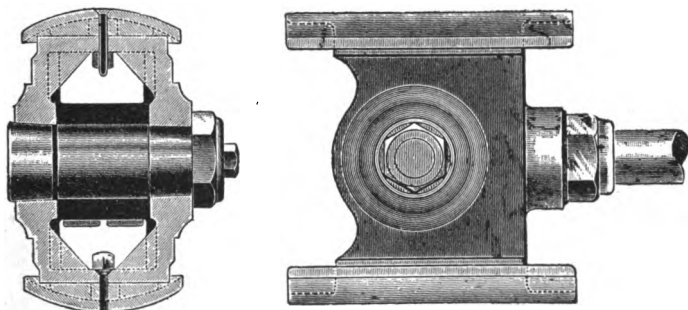
FIG. 49.—Cross-head.
