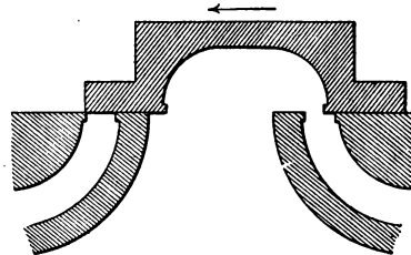
FIG. 38.—Cut-off.
