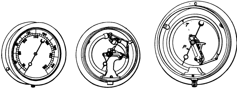
FIG. 26.—Steam gages.
