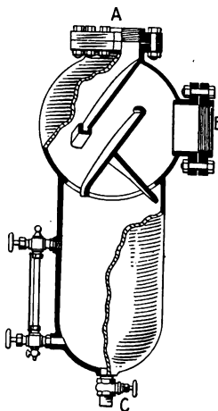
FIG. 59.—Steam separator.
