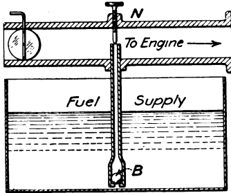
FIG. 77.—Suction-feed carburetor.
