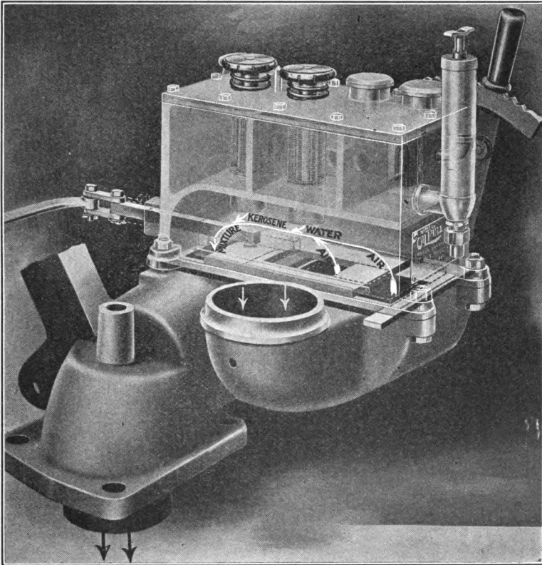
FIG. 186:—Kerosene carburetor.
