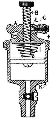
FIG. 54.—Automatic grease cup.
