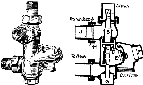
FIG. 31.—Injector.
