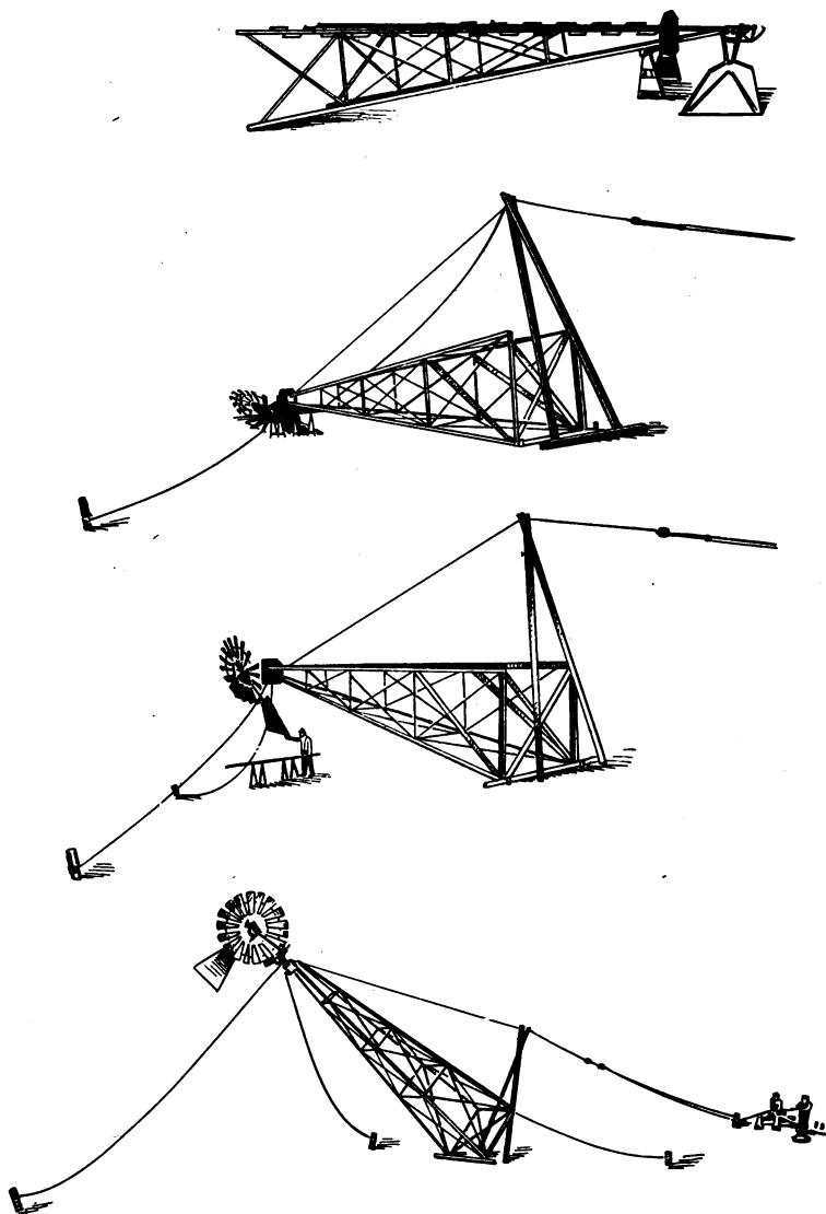
FIG. 232.—Method of raising windmill from the ground.
