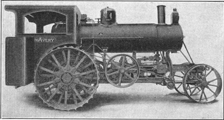
FIG. 162.—Undermounted traction engine.
