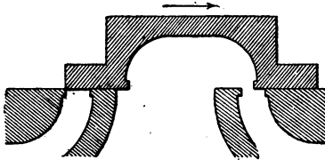
FIG. 37.—Admission.
