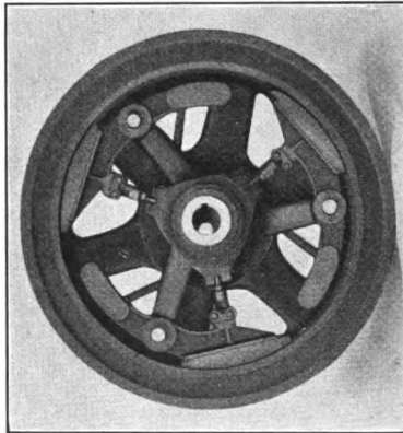
FIG. 188.—Clutch.
