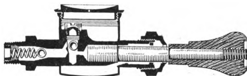
FIG. 58.—Hand oil pump.
