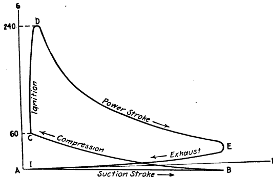
FIG. 68.—Gas-engine indicator card.
