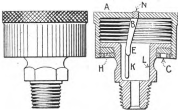
FIG. 53.—Grease cups.
