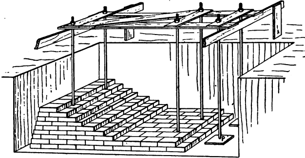
FIG. 62.—Foundation in the process of construction.
