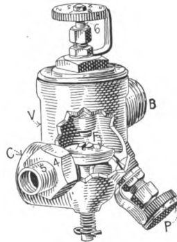
FIG. 76.—Gravity carburetor.
