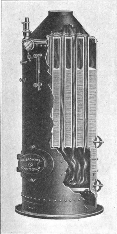
FIG. 7.—Vertical boiler. Exposed tube type.
