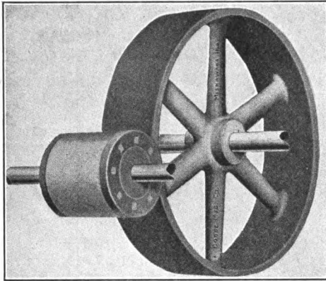
FIG. 283.—Friction gears.
