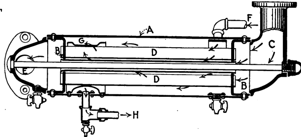
FIG. 165.—Feed-water heater.
