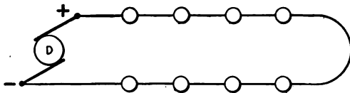
FIG. 252.—Series system of distribution.
