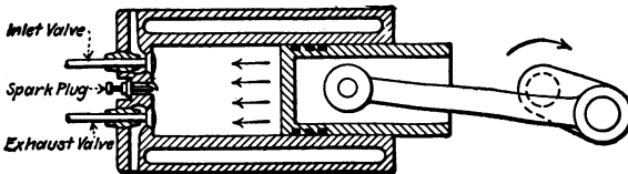
FIG. 64.—Compression.
