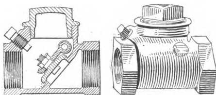
FIG. 23.—Check valve.
