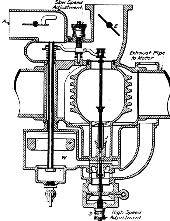
FIG. 82.—Kerosene carburetor.
