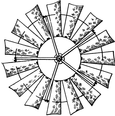
FIG. 220.—Samson wheel.
