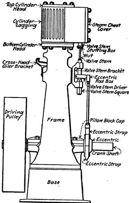
FIG. 35.—Vertical steam engine.
