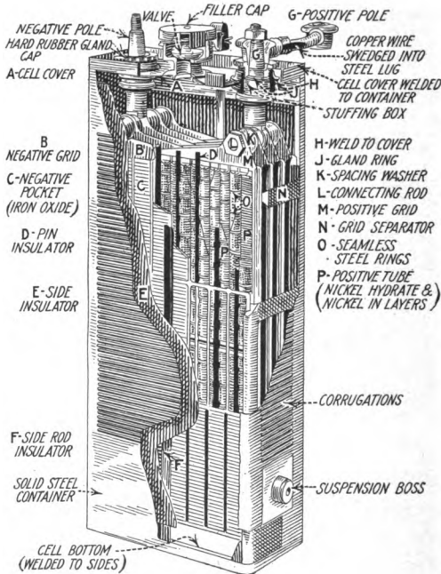
FIG. 238.—Edison storage battery.
