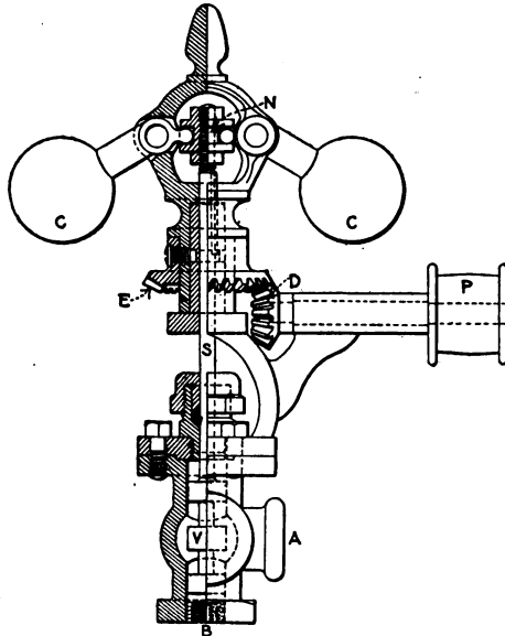
FIG. 47.—Steam-engine governor.
