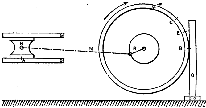
FIG. 43.—Valve setting.
