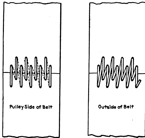
FIG. 273.—Belt lacing.
