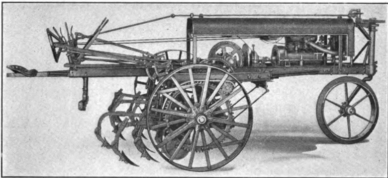
FIG. 201.—Tractor cultivator.
