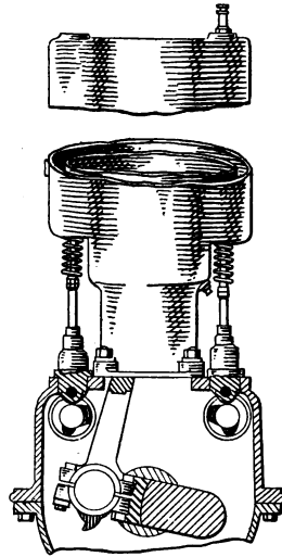
FIG. 130.—Tee-head cylinder.
