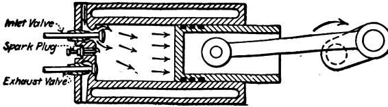
FIG. 63.—Suction.
