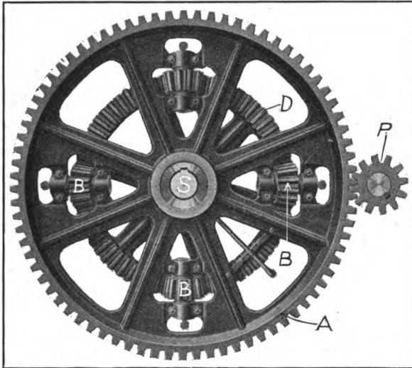
FIG. 174.—Differential.
