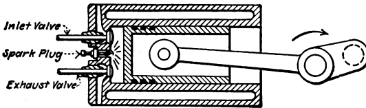
FIG. 65.—Ignition.
