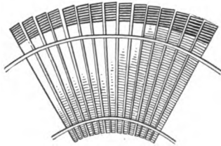
FIG. 221.—Section of wooden wind wheel.
