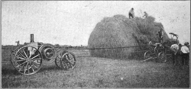
FIG. 202.—Hay-baling machine driven by traction engine.
