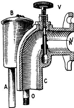
FIG. 74.—Pump-feed carburetor.
