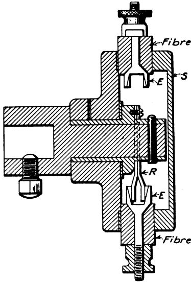
FIG. 103.—Timer.
