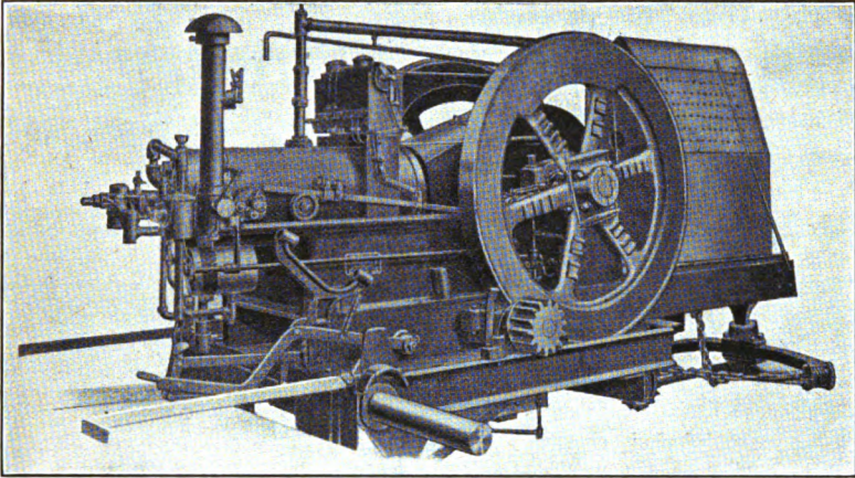
FIG. 176.—Single-cylinder motor.
