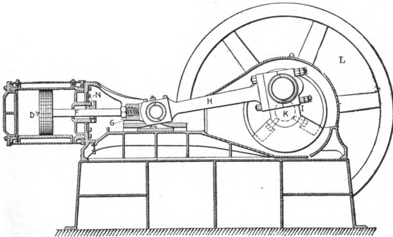
FIG. 34.—Steam engine.
