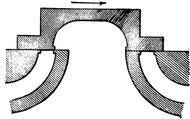
FIG. 40.—Compression.
