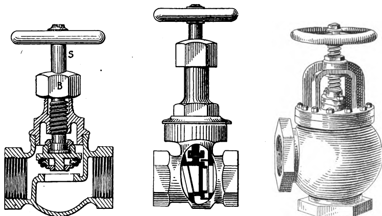
FIG. 20.—Globe valve. FIG. 21.—Gate valve. FIG. 22.—Angle valve
