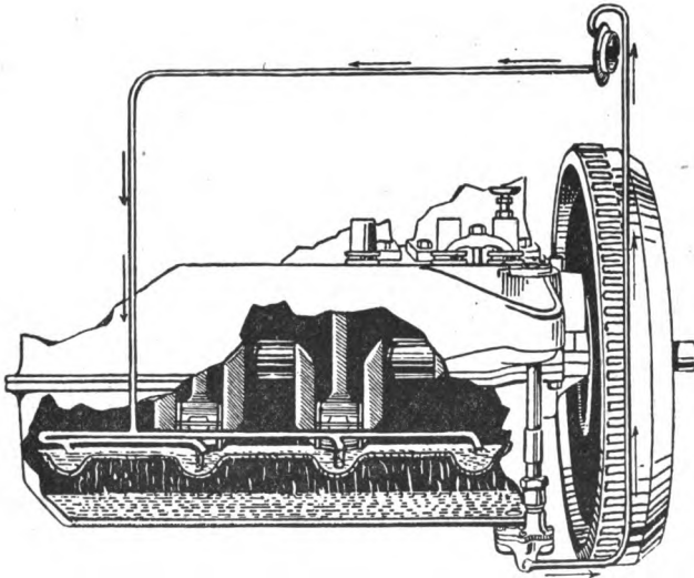
FIG. 109.—Forced-flooded lubrication system.
