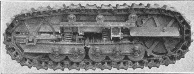
FIG. 196.—Track of crawler type tractor.
