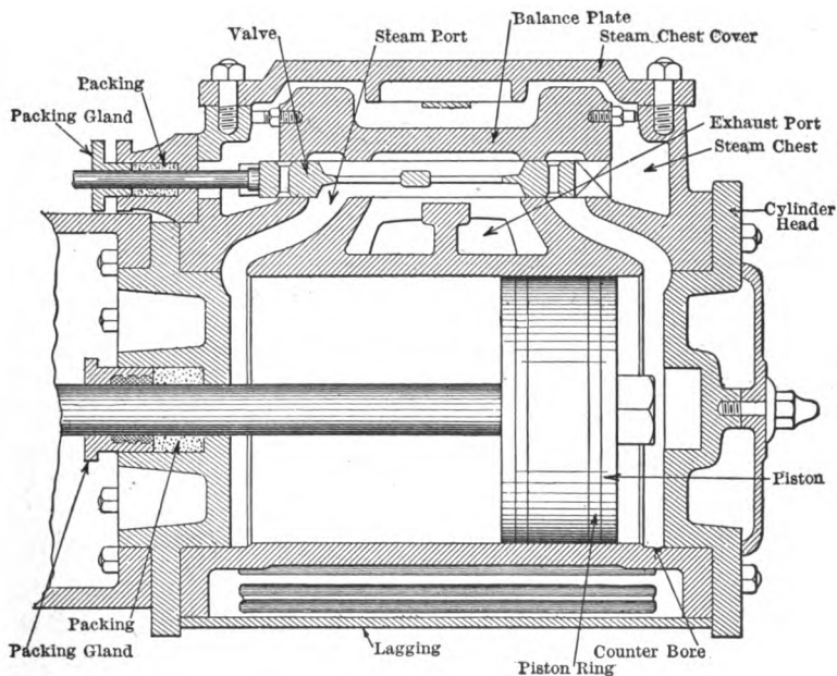
FIG. 42.—Balanced valve.
