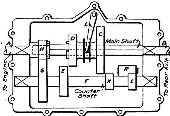
FIG. 135.—The progressive sliding-gear transmission system.
