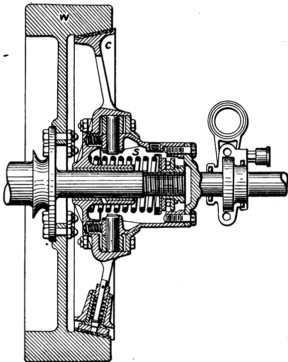
FIG. 133.—Cone clutch.
