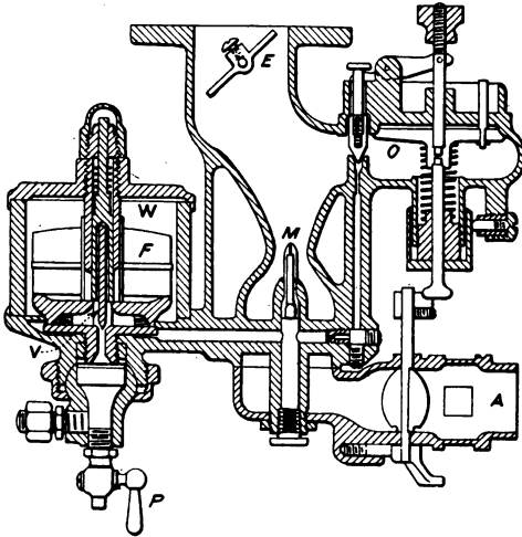
FIG. 79.—Stromberg carburetor.
