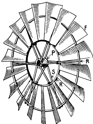
FIG. 217.—Wind wheel.
