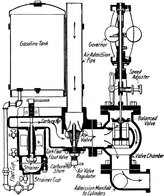
FIG. 185.—Traction-engine carburetor and governor.
