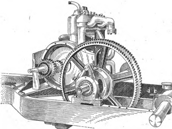
FIG. 190.—Traction-engine transmission.
