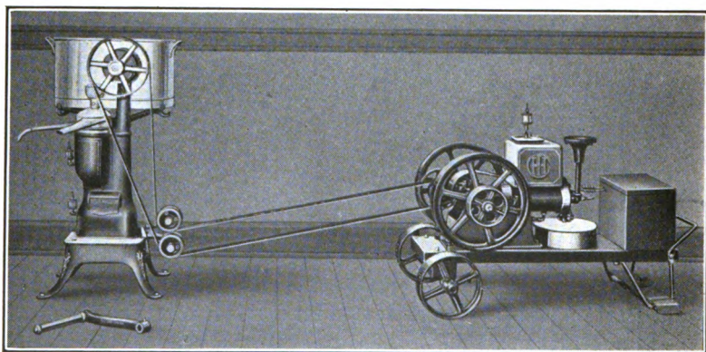
FIG. 116.—Driving cream separator.
