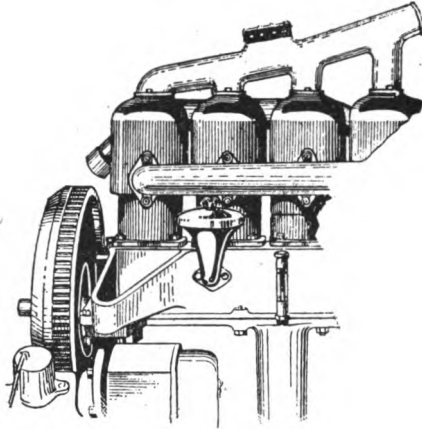
FIG. 122.—Automobile motor, cylinders cast singly.
