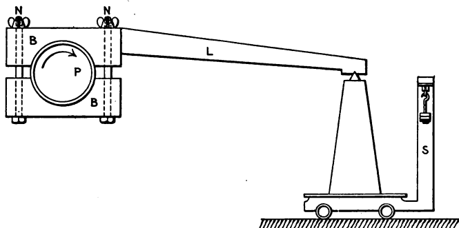
FIG. 2.—Prony brake.
