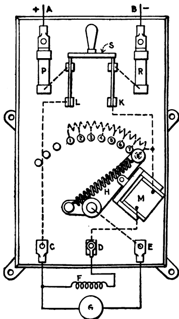
FIG. 266.—Method of connecting motors.
