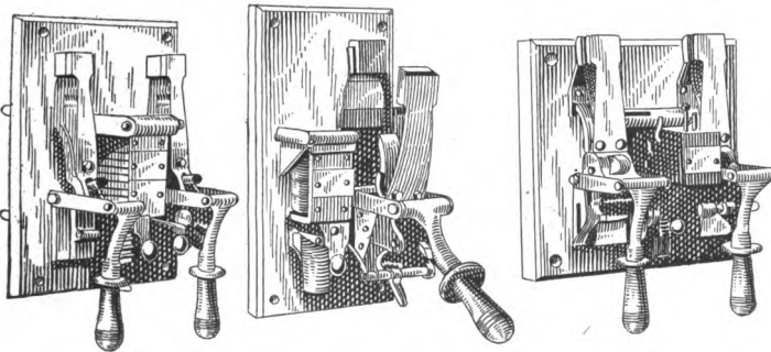
FIG. 262.—Circuit breakers.
