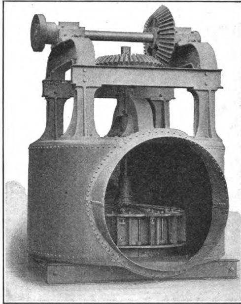
FIG. 212.—Water turbine.
