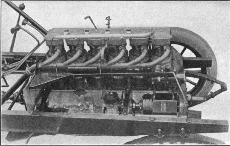
FIG. 126.—Air-cooled automobile motor.
