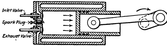
FIG. 66.—Expansion.
