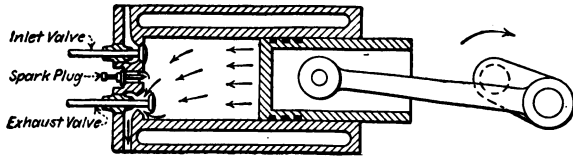
FIG. 67.—Exhaust.
