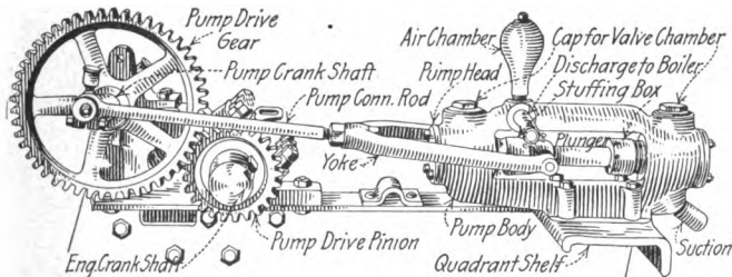
FIG. 164.—Gear-driven pump.
