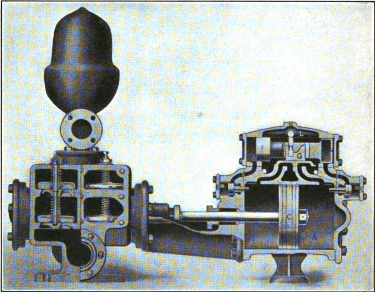
FIG. 30.—Boiler feed pump.
