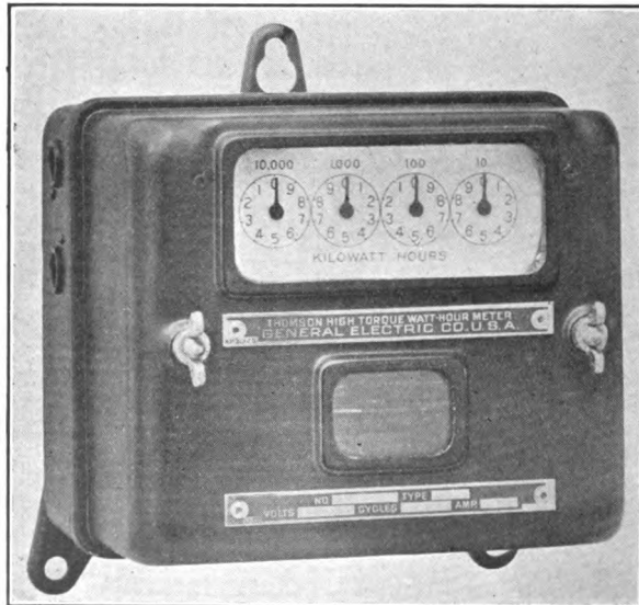
FIG. 258.—Alternating-current wattmeter.
