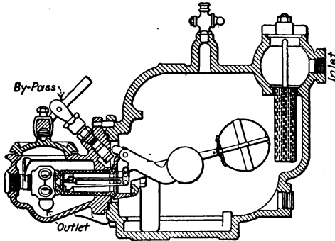
FIG. 28.—Steam trap.
