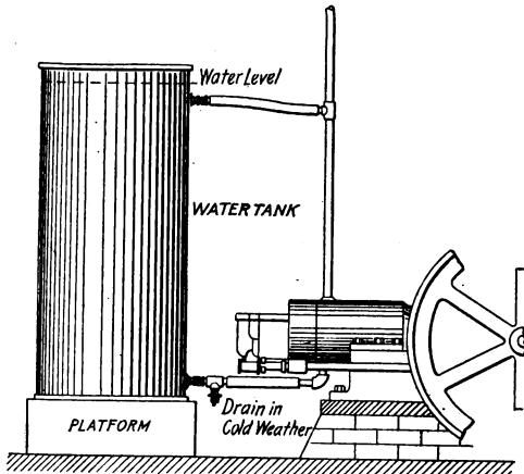
FIG. 85.—Gas-engine water-cooling system.
