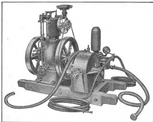
FIG. 114.—Spraying outfit.
