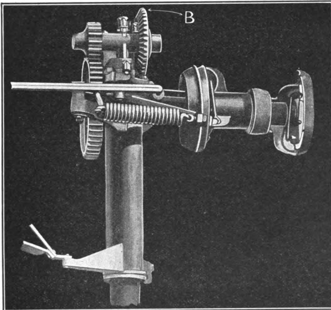
FIG. 226.—Power windmill.
