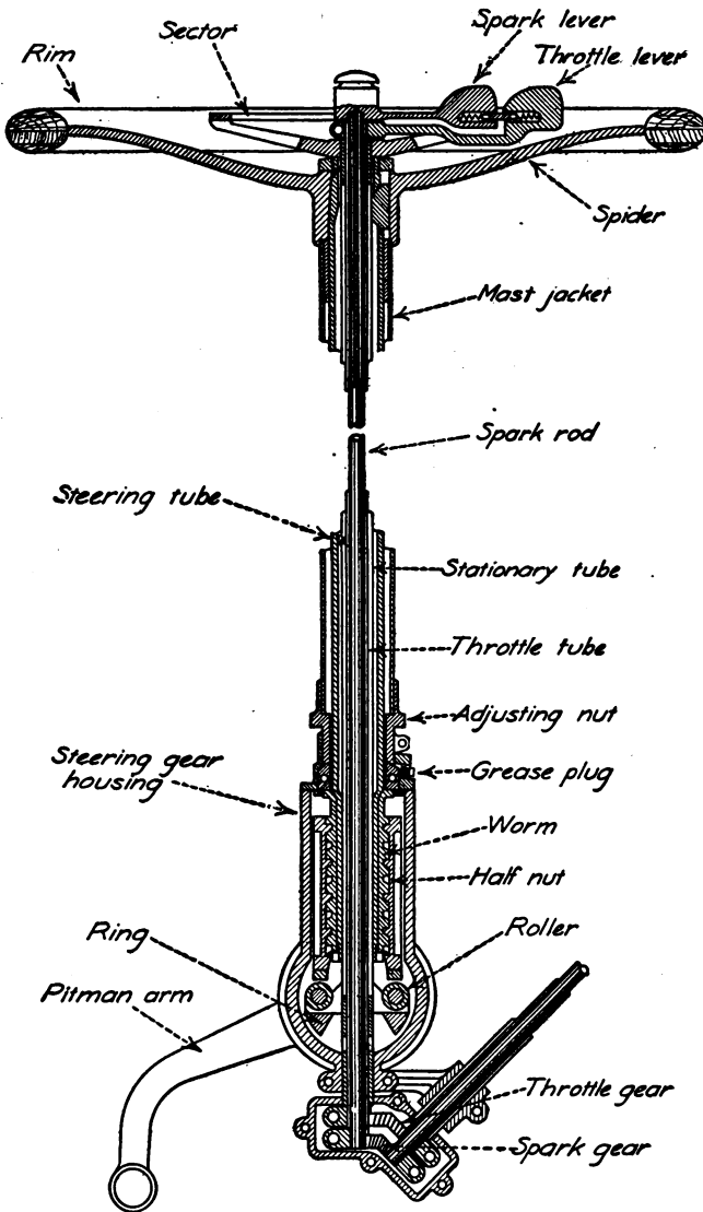
FIG. 145.—Steering gear.
