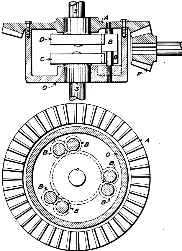
FIG. 142.—Spur-gear differential.
