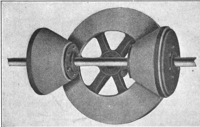
FIG. 284.—Friction gears.
