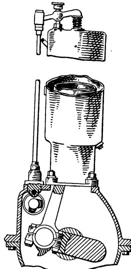
FIG. 132.—Valves-in-the-head cylinder.
