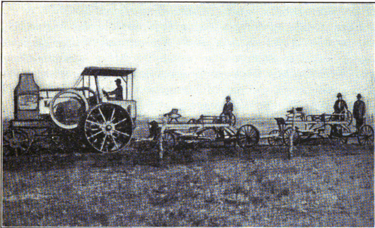
FIG. 203.—Tractor used for pulling graders.
