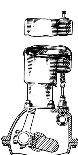
FIG. 131.—Ell-head cylinder.
