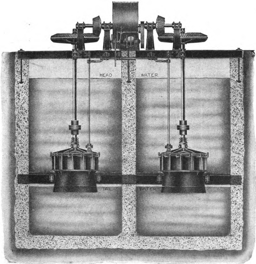
FIG. 213.—Water-power installation.
