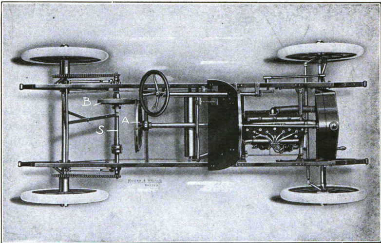
FIG. 140.—Chassis of automobile with friction drive.
