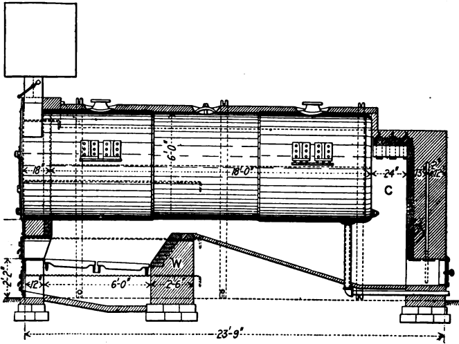
FIG. 5.—Details of boiler setting.
