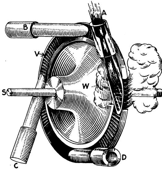
FIG. 61.—Steam turbine.
