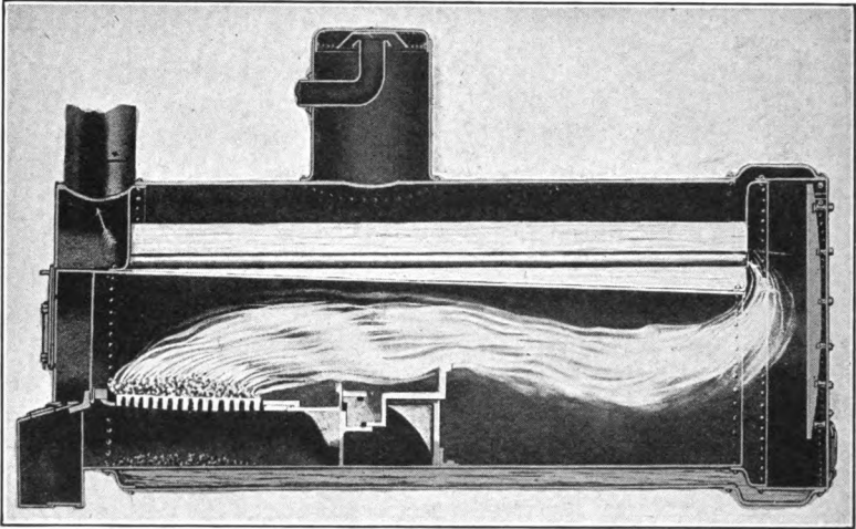
FIG. 158.—Flue-type boiler.
