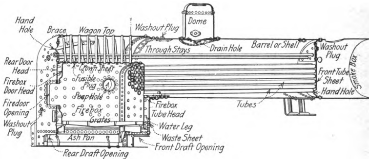
FIG. 159.—Locomotive-type boiler.
