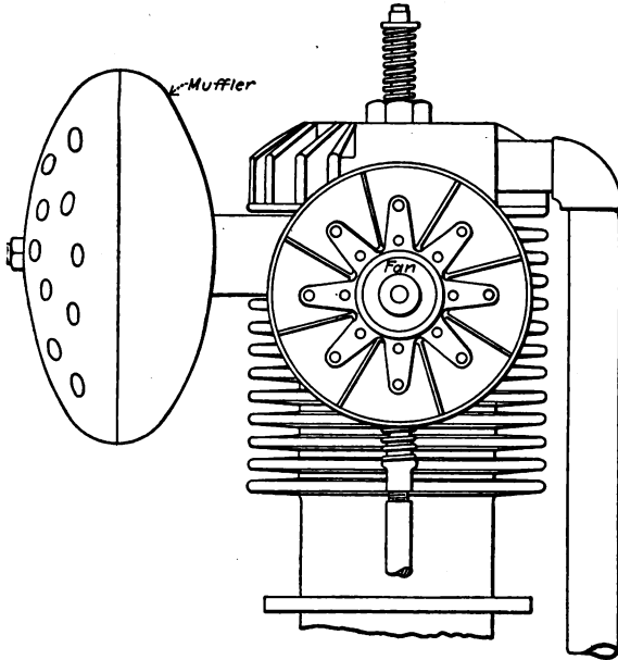
FIG. 84.—Air-cooled engine.
