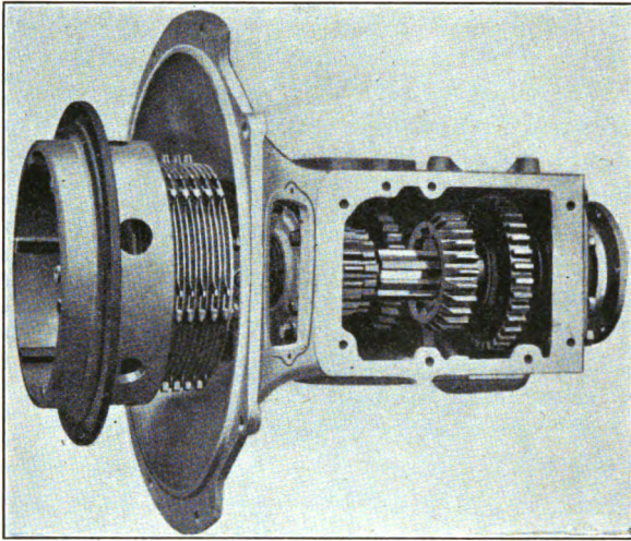
FIG. 137.—Transmission system and clutch.
