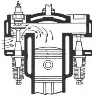
FIG. 127.—Motor with poppet valves.
