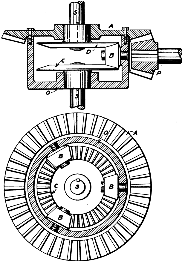
FIG. 141.—Bevel-gear differential.
