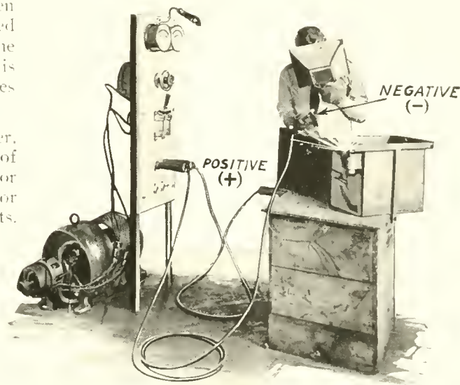
Fig. 1. In arc welding, one wire (the positive) from the welding apparatus is attached or laid upon the steel which is to be welded; the other wire (the negative) is attached to the electrode of carbon or metal which the operator holds.
