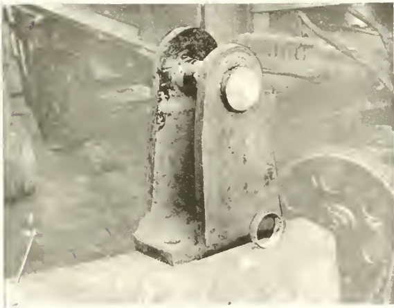
Fig. 32. Brake fulcrum repaired by Electric Arc Welding. The hole in this fulcrum was badly worn. By placing a copper band or ferrule of the right size in the hole and building up around it the hole could be knocked out after the welding was completed, leaving a perfectly smooth, round hole, which needed no machining.
