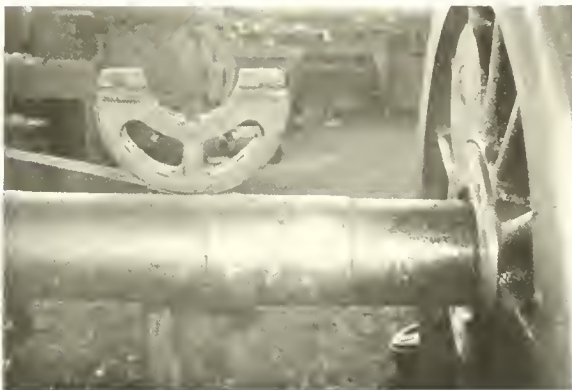
Fig. 33. An eccentric shay repaired by electric welding showing how it is possible to weld both malleable and grey iron. The key way in the driving wheel shaft has also been built up and milled out, saving the scrapping of the entire shaft.
