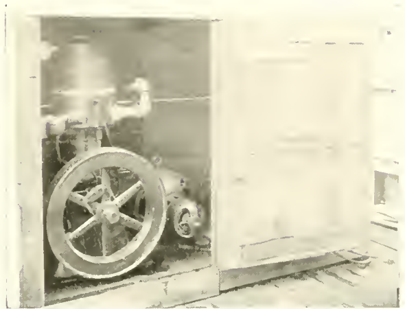
Fig. 63A. Lincoln Arc Welder direct geared to a 10 H. P. Novo Gasoline Engine, making an ideal outfit for ship building and repair work, where a portable outfit is required.
