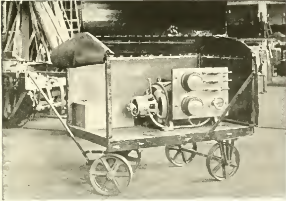
Fig. 51. Lincoln Arc Welder (Portable Type) with canvas housing as used in engine house on Eastern Railroad. The canvas burns out the dust and dirt prevalent around the engine house.
