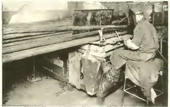
Fig. 98. Welding defects in steel tubes with an electric arc welder.
