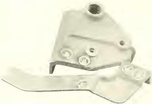
Fig. 28. Same parts as shown in Fig. 27, after welding. The faces are ground off clean and no difficulty was experienced in machining.
