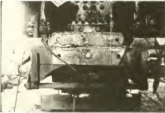
Fig. 37. BEFORE. The edges of the sections are clipped off with the hammer, making a "V" shaped groove.
