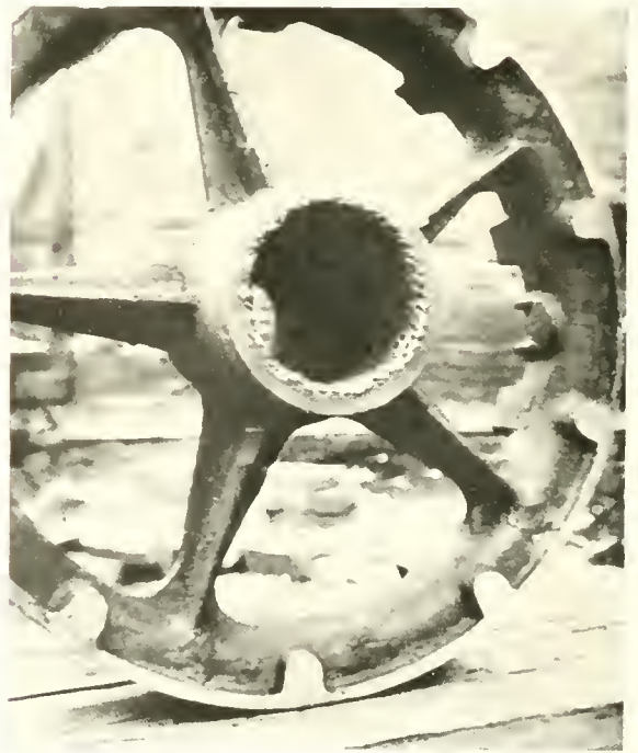
Fig. 103. This steel casting was wrongly machined. The hole in the center being machined out too large. This shows how it was built up with a Lincoln Arc Welder and afterwards machined to the proper size, saving the casting from the scrap heap.
