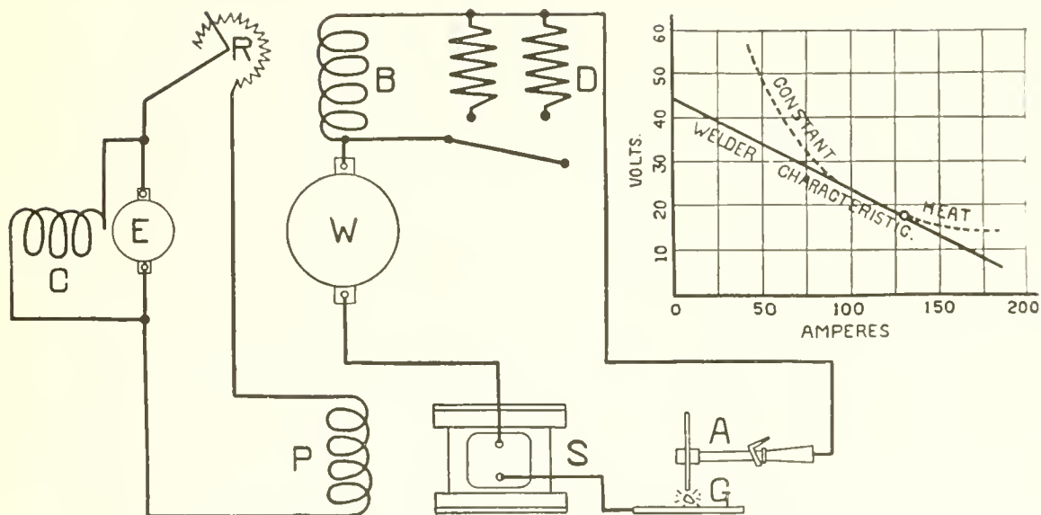
Fig. 1. Diagram of Electrical Connections of D.C. A.C. Welder, and Volt-Ampere Characteristic
