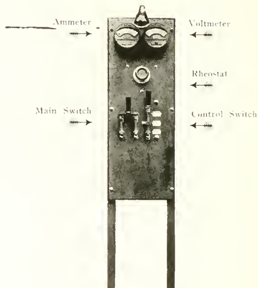
Fig. 126. Stationary Panel
