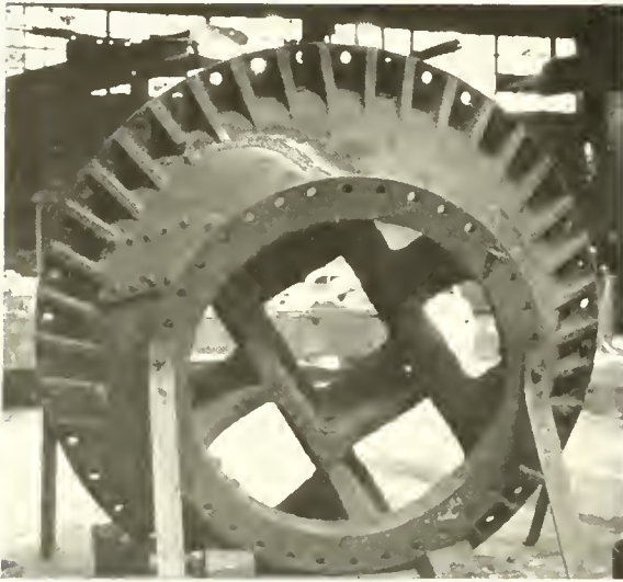
Fig. 22. Large steel casting repaired by arc welding after it had been in service. This casting was also been repaired once by riveting. Note how much cleaner the welded job is.
