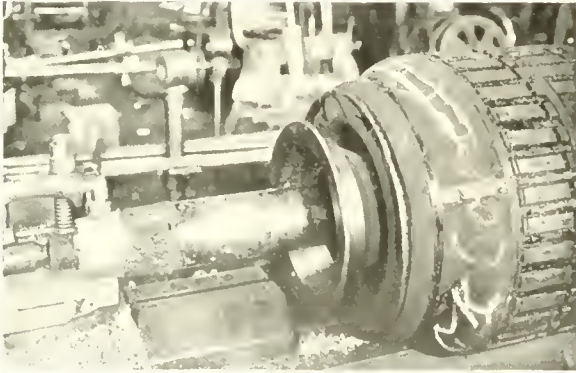
Fig. 12. An Arc Welded cast iron flange cut to the size of a machine shaft which has been worked to the full size by welding. The new metal has the same strength as the original.
