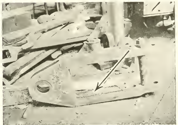
Fig. 48. Worn Steel Casing—Locomotive Part—repaired by building up worn surface by arc welding.
