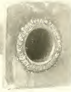
Fig. 104B. FLUE WELDING. 1. Put the flue in if it were not to be welded. 2. Send the engine out for a few trips to let the tubes take their set. 3. Sand blast the flue sheet. 4. Weld flues. A heavy bead of welded metal around the flue is not desirable. Put on the smallest bead that can be thoroughly welded to both flue and sheet.
