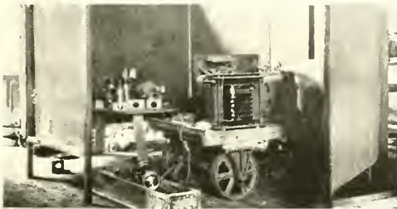
Fig. 34. Lincoln Arc Welder in Rock Island R. R. shops, Selvis, Ill., showing the black canvas screen with which the Welder is surrounded, thus protecting the eyes of other workmen from glare.
