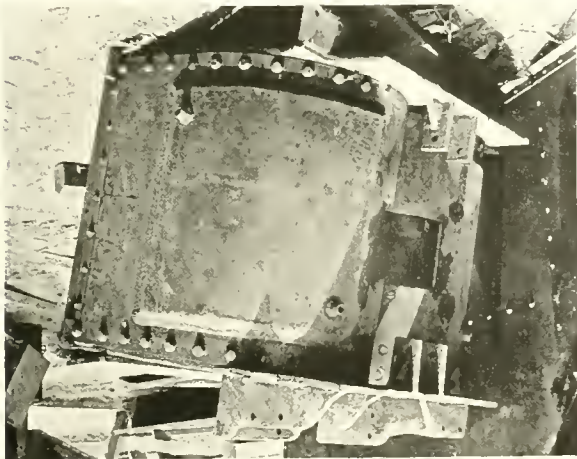
Fig. 88A. Asphalt Mixer with arc welded Heating Jacket. Welding saved 70% over riveting and increased jacket capacity by avoiding flanges and rivets on the inside.
