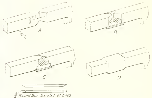
Fig. 39. Drawing showing method of repairing engine frame. (Courtesy RAILWAY MECHANICAL ENGINEEFF)
