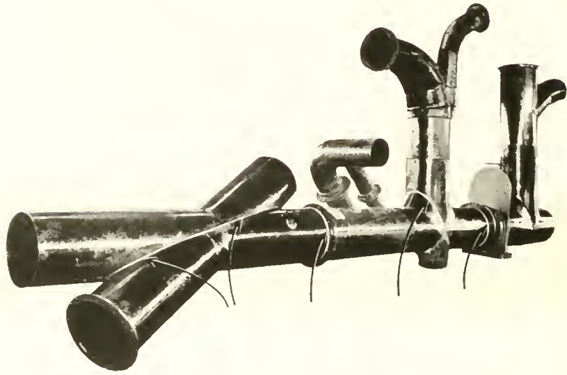
Pipes for gas apparatus made by the Connerly Co., Philadelphia, Pa., with Lincoln Arc Welder.
