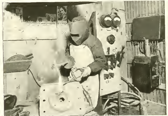
Fig. 10. Carbon Electrode Welding. The operator holds the carbon electrode with the right hand and feeds the filling metal into the weld from a roll held in his left hand.
