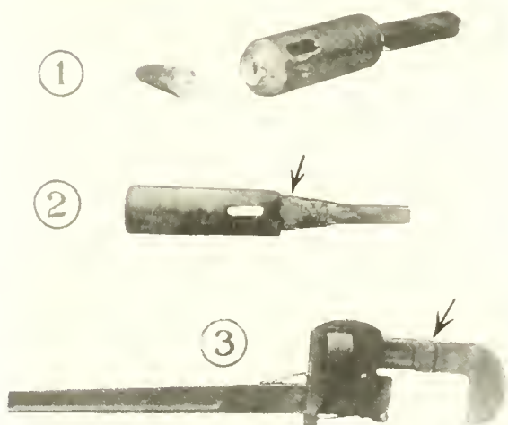
FIG. 50. The prompt repair of broken shop tools is often of great importance in the railroad repair shop. (1) A broken air drill socket for 1" diameter drill. A new socket would have cost $1.80, besides delaying an important repair job. (2) The same drill socket repaired by the Lincoln Arc Welder. Cost of repair, including preparation of weld, was 12 cents. (3) Broken pipe wrench for 3" pipe, repaired by the Lincoln Arc Welder. A new wrench would have cost about $6.00. The repair cost 20 cents, including preparation, welding and grinding off superfluous metal at weld.
