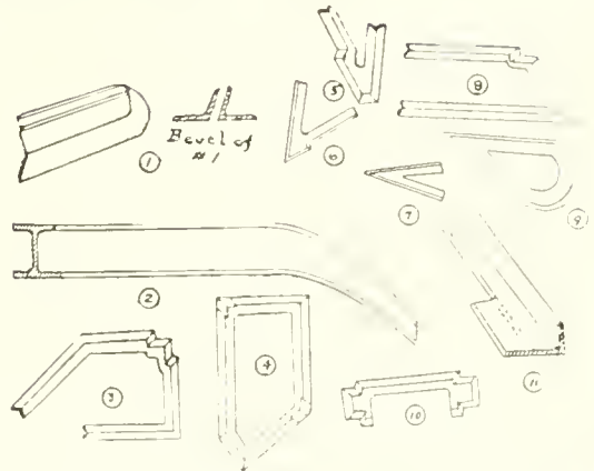
Fig. 56. The sketches show pieces which can be made with the electric arc in ship yards. No. 1 is a very difficult and expensive job for the angle smith, but can be made for a few cents with the electric arc welder. No. 2 is a boat davit made from an 8 inch I beam split and rewelded. The cost of this from the angle smith would be $6.00 or $7.00, whereas it can be electric welded for $1.00.
