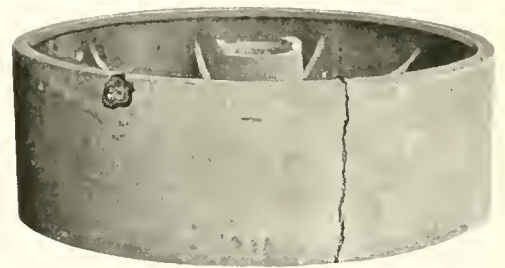
Fig. 24. Defective pulley casting. Repairing this with a Lincoln Arc Welder saved $10.20 in 10 minutes.
