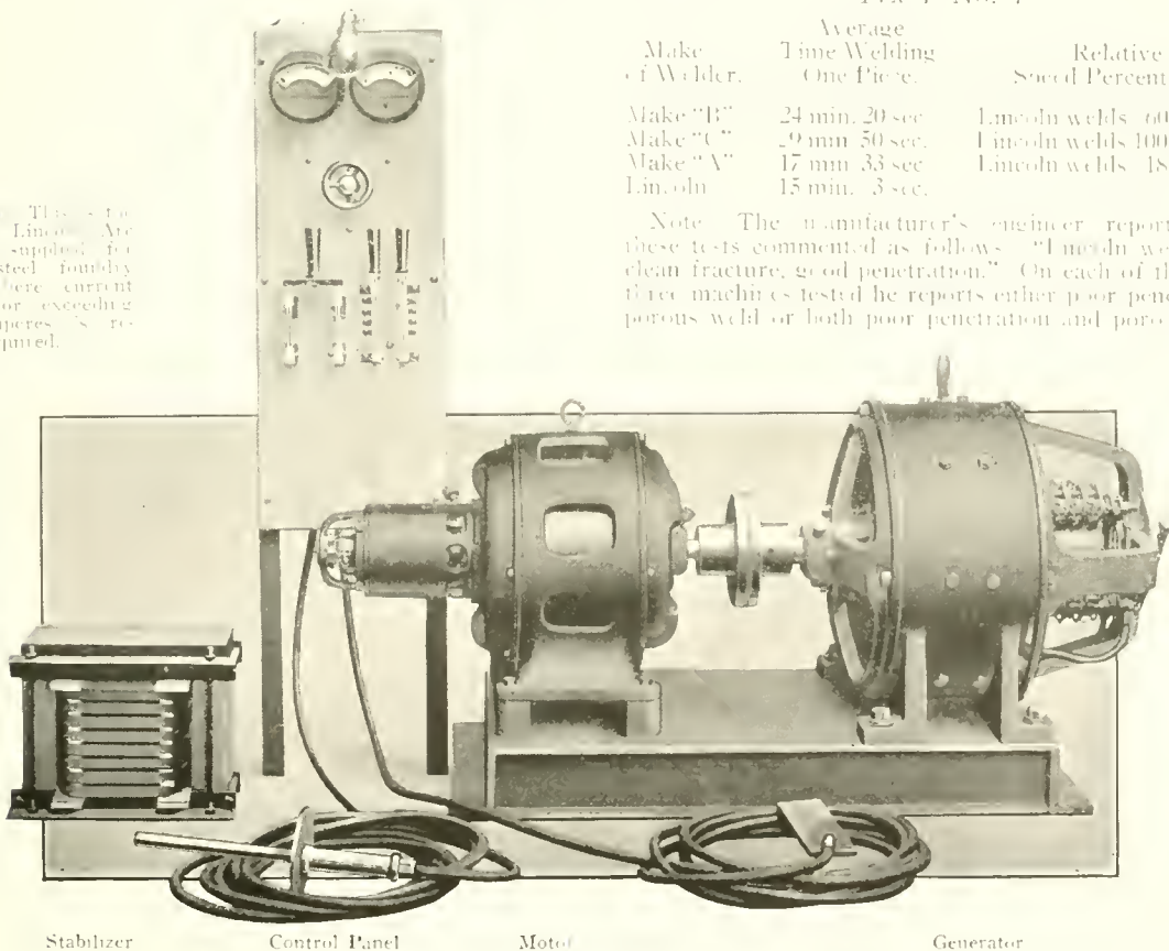
Stabilizer
