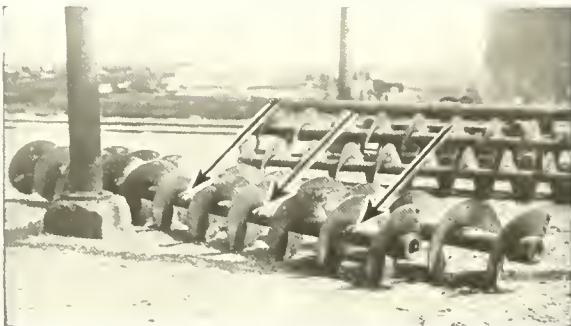
Fig. 92 Screw conveyors made by arc welding the spiral steel vanes to a central shaft.
