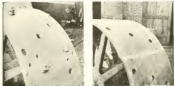
Fig. 91. BEFORE GRINDING. Steel Wheel made by welding a steel plate rim and bolting it to steel spokes. AFTER GRINDING. Steel Wheel after the weld in the rim has been ground down to give smooth surface.
