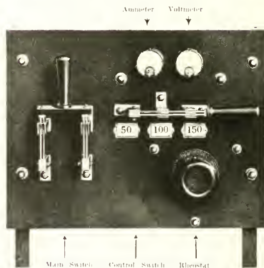
Fig. 127. Portable Panel
