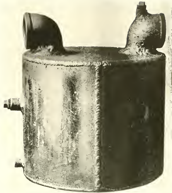
Fig. 7. Gas tank made by the Boom Boiler & Welder Co., Cleveland. This tank has been made both by arc welding and by acetylene welding. The arc welding costs 1 to 1½ as much as gas welding. The tank is tested at 150 lbs. water pressure.
