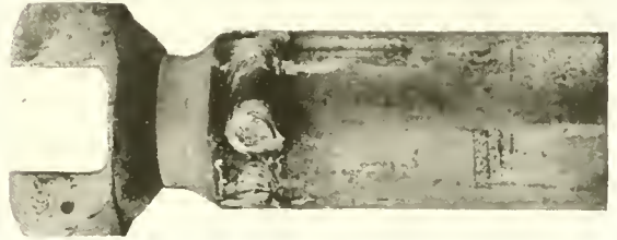
Fig. 97. Flexible shaft for automobile, arc welded.
