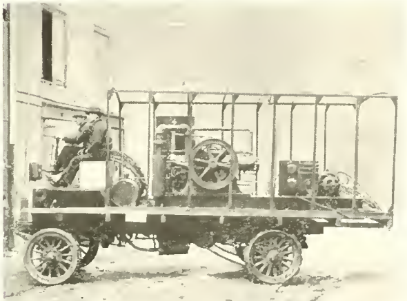
Fig. 65. Gasoline driven unit on motor truck.
