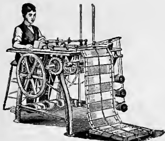
Jacquard Card-Lacing Machine.
