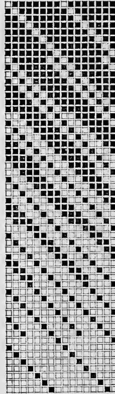
FIG. 103. 8-HARNESSTWILL.
