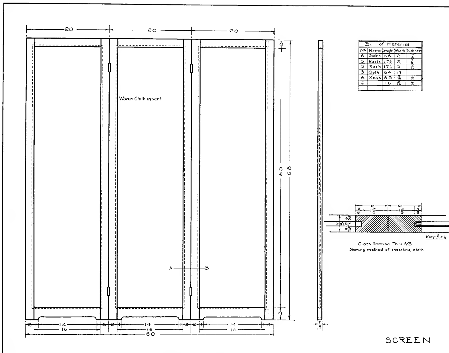
Fig. 420—Working Drawing of Screen
