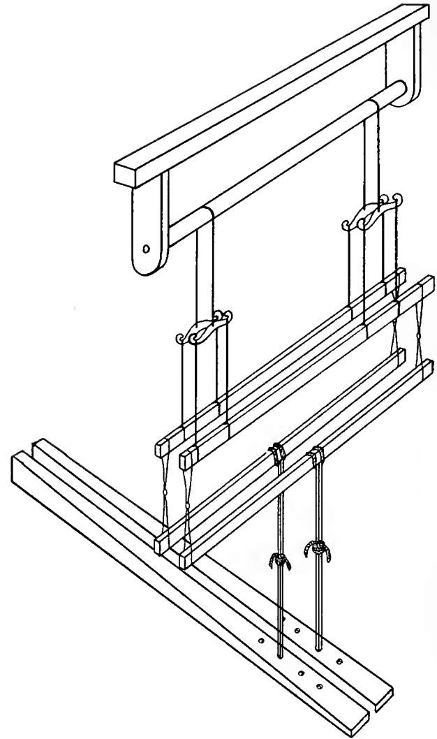
Fig. 42—Method of Tying Heddle Sticks to Treadles
