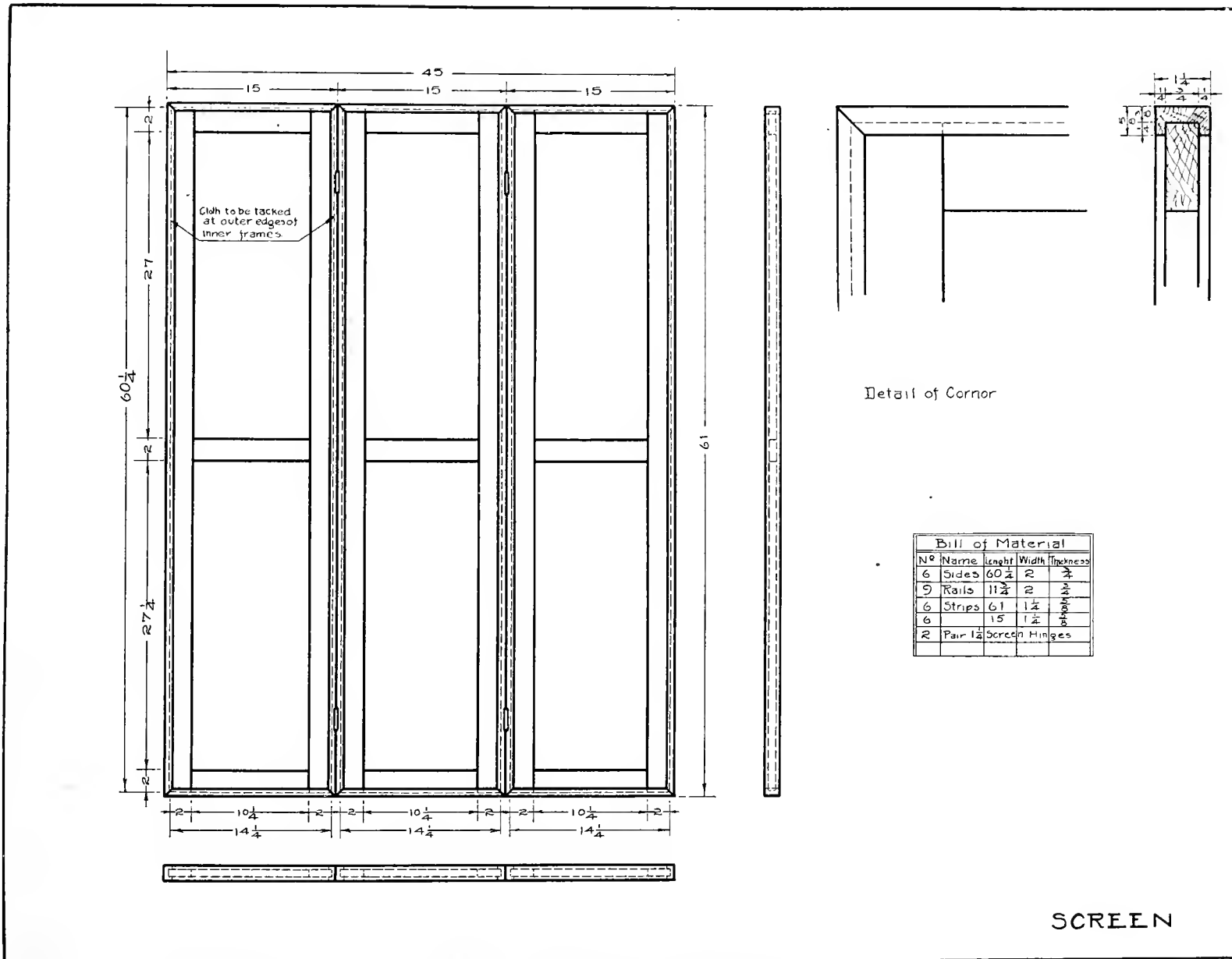
Fig. 422—Working Drawing of Screen
