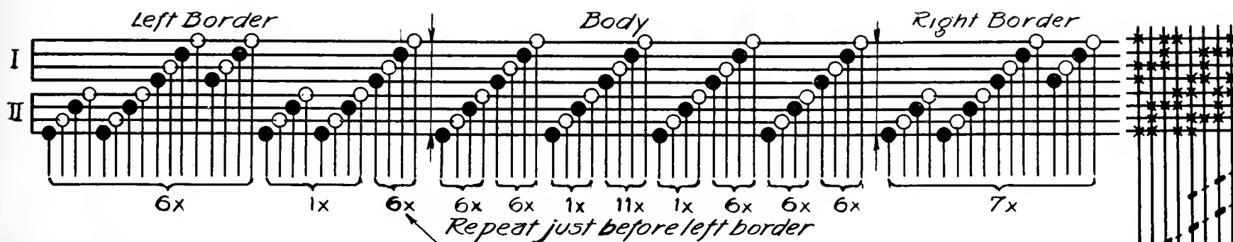
Fig. 412—Double Weave Draft.
