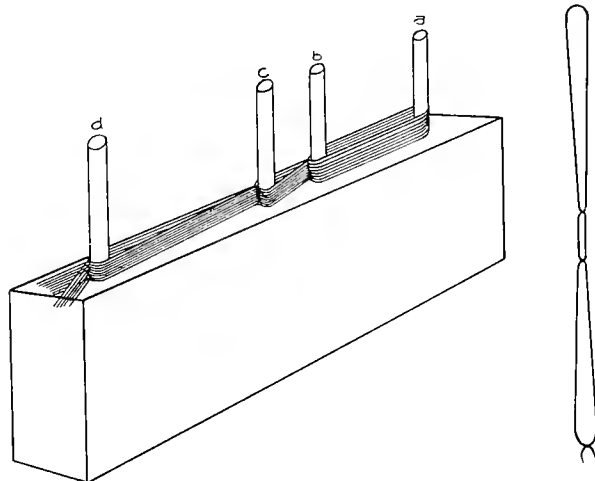
Fig. 30—Method of Tying Heddles
