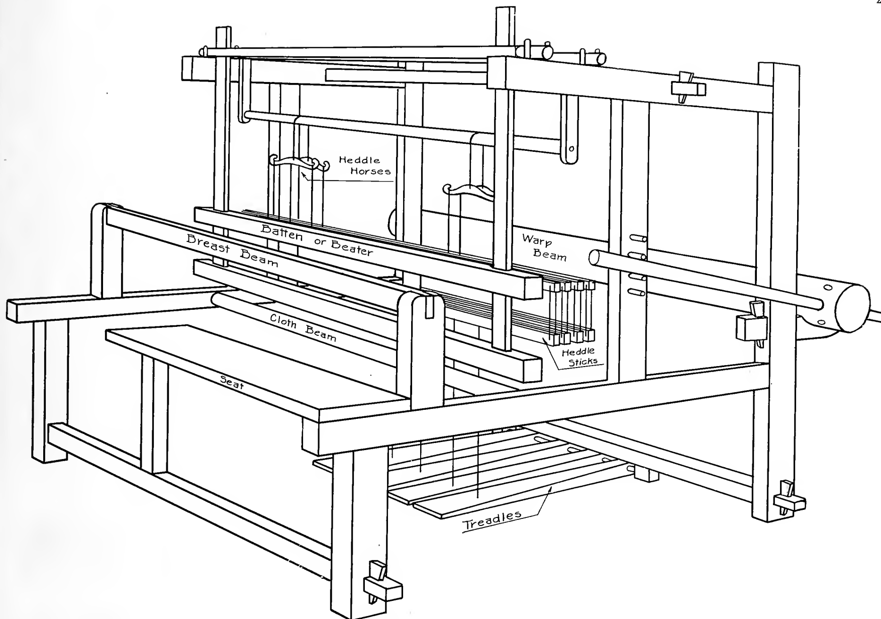
Fig. 20—Loom with Parts Named
