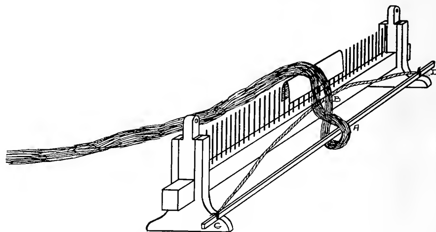
Fig. 25—Stand to Hold Spreader
