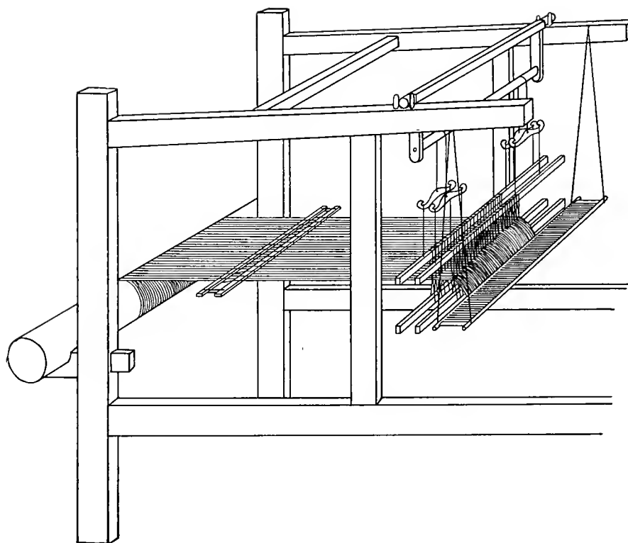
Fig. 34—Reed in Position for Threading
