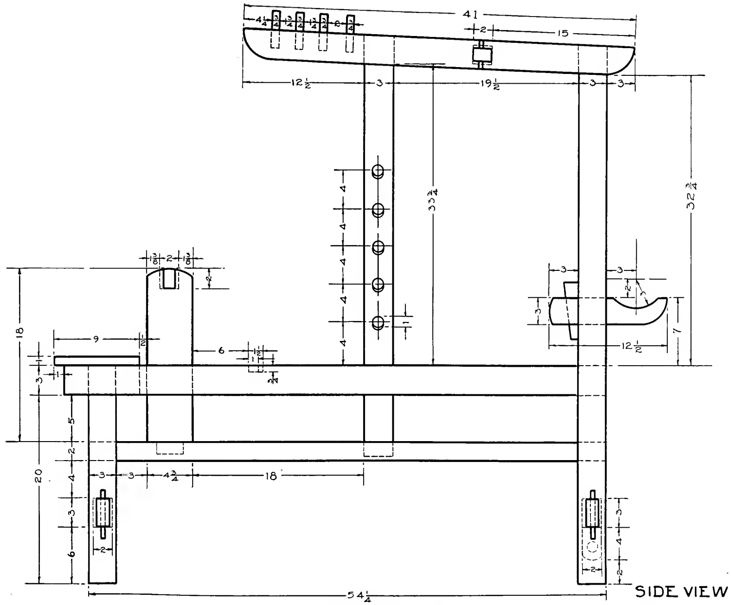
Fig. 430—Working Drawing of Swedish Loom
