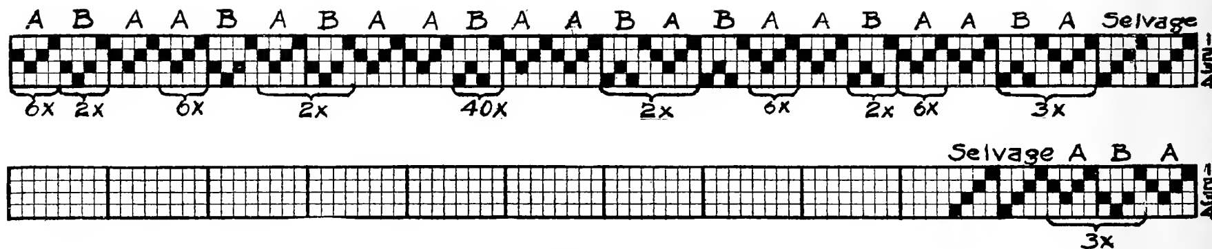
Fig. 404—Table Mat. Draft of Pattern
