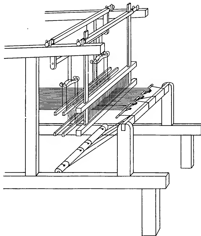
Fig. 44—Warp Tied to Cloth Beam
