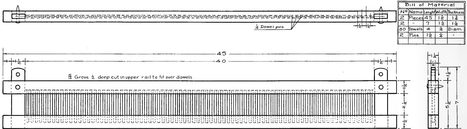
Fig. 21—Working Drawing of Warp Spreader or Raddle
