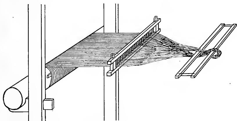
Fig. 27—Lease Rods in Place
