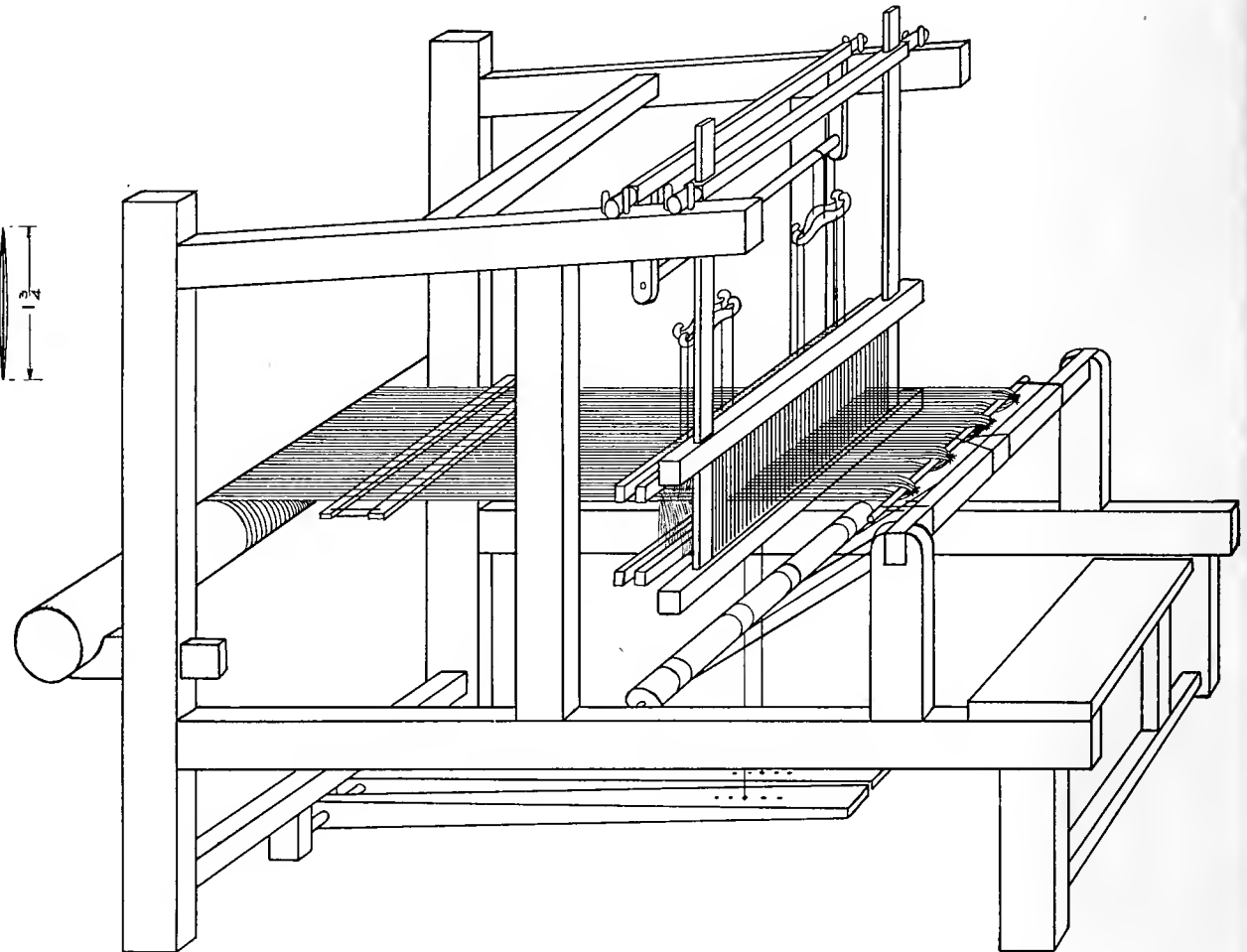
Fig. 36—Loom Ready for Tying Up
