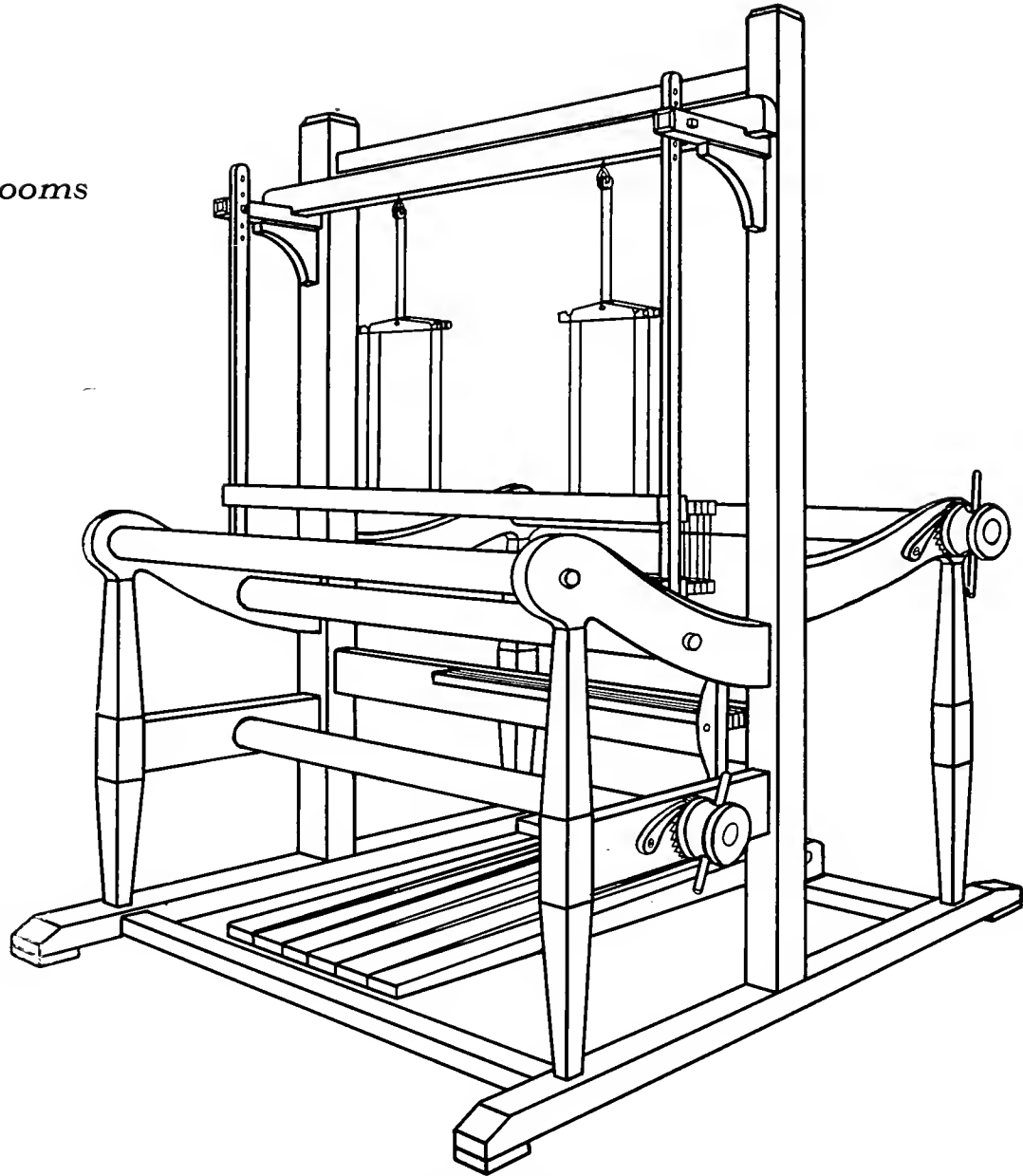
Fig. 424—Sketch of Danish Loom
