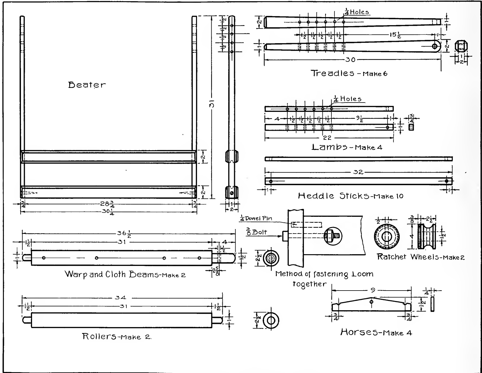
Fig. 427—Working Drawing of Loom—Details
