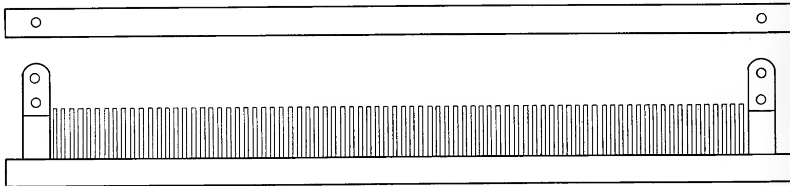
Fig. 22—Warp Spreader with Cap Removed
