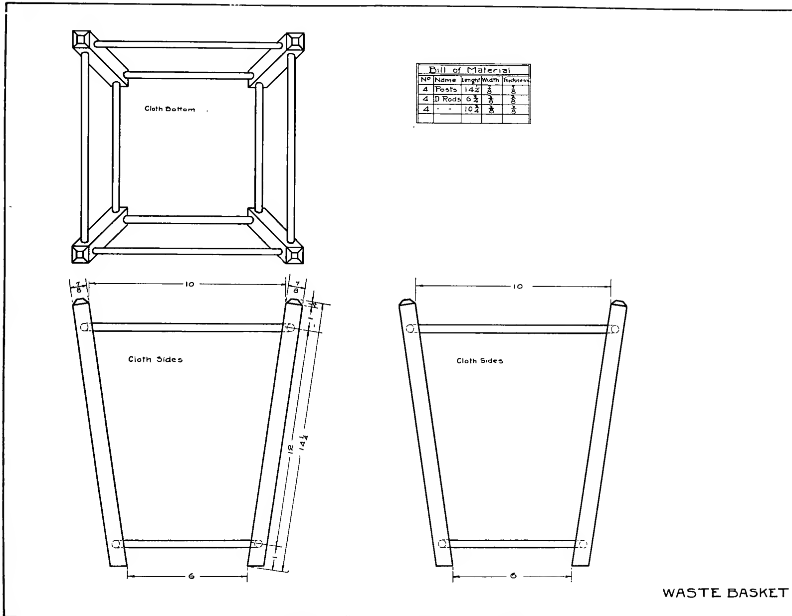
Fig. 418—Working Drawing of Waste Basket
