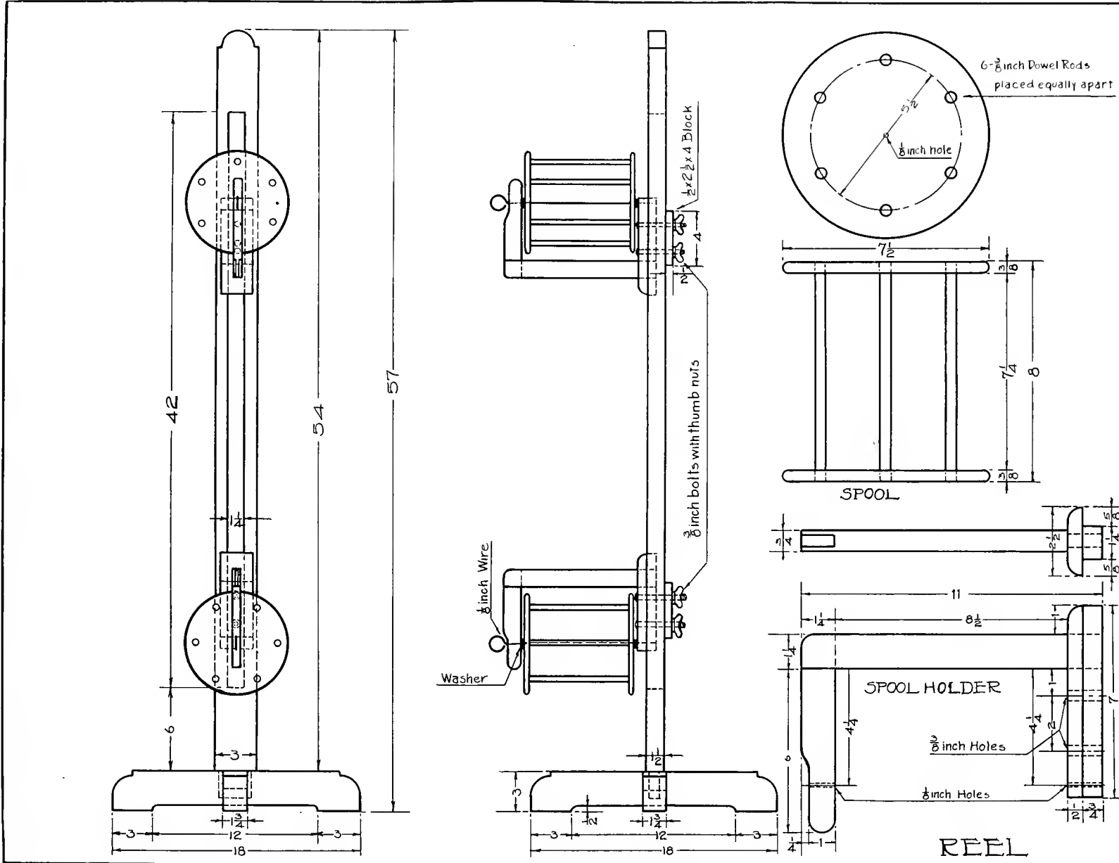
Fig. 54—Working Drawing of Reel
