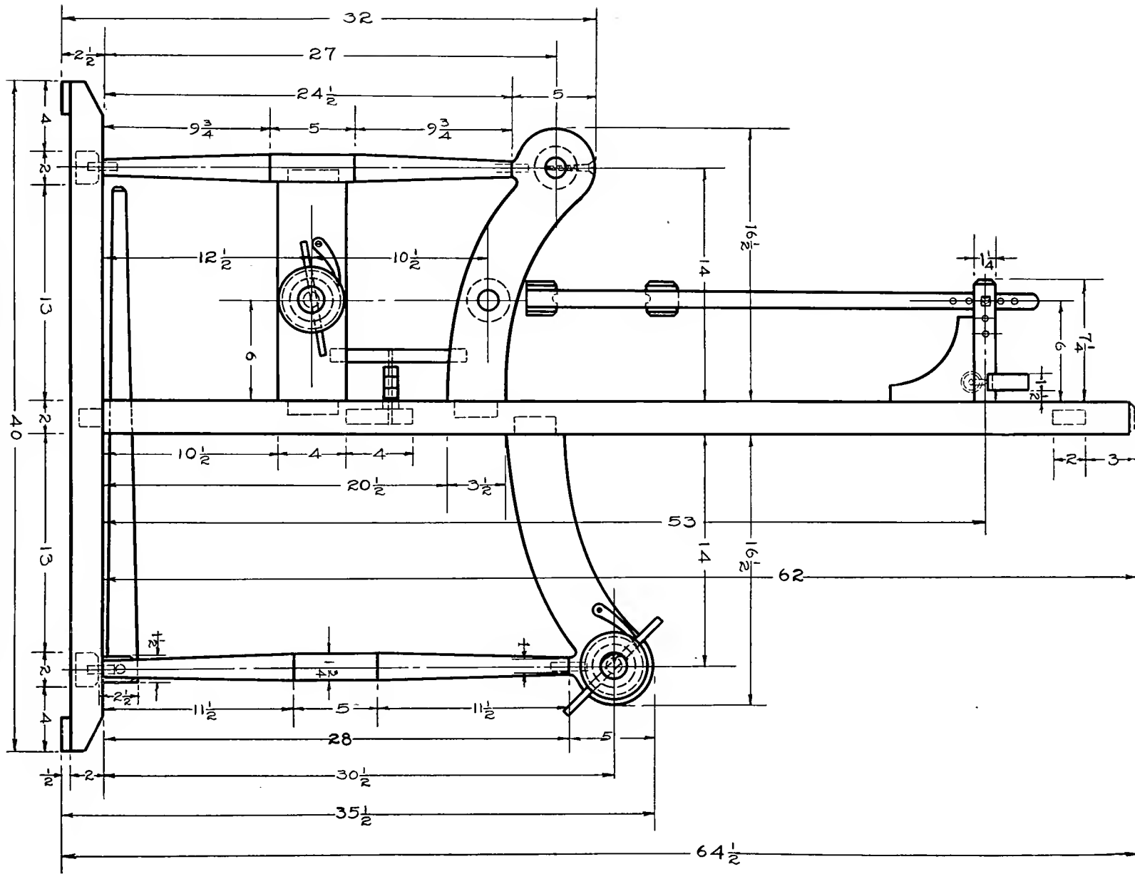
Fig. 426—Working Drawing of Loom—Side View
