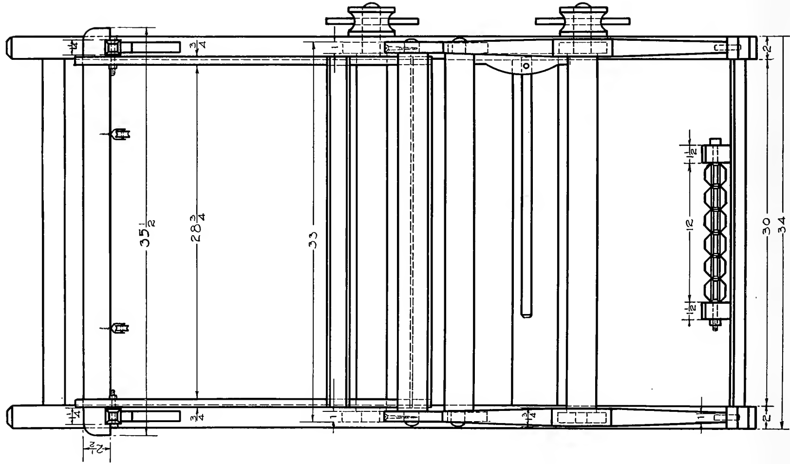
Fig. 425—Working Drawing of Loom—Front View
