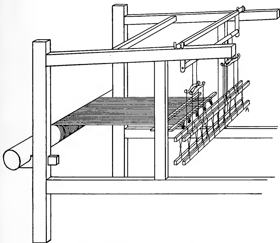
Fig. 31—Heddles in Place for Threading
