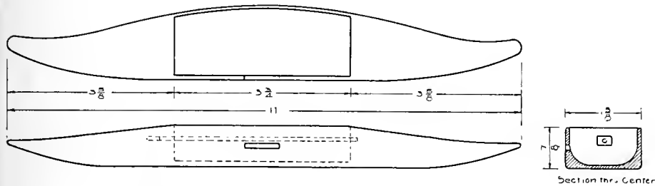
Fig. 46a—Working Drawing of Small Shuttle
