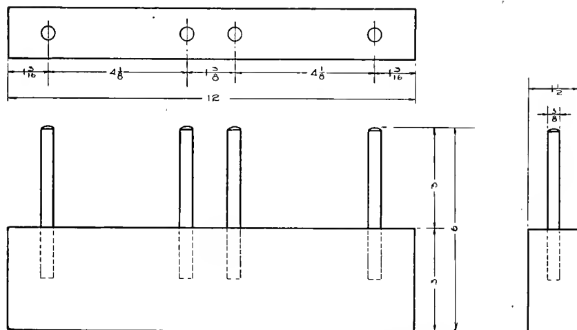
Fig. 29—Working Drawing of Heddle Frame
