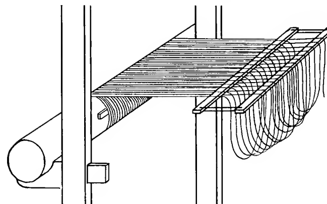
Fig. 28—Loops Hanging Over Lease Rods
