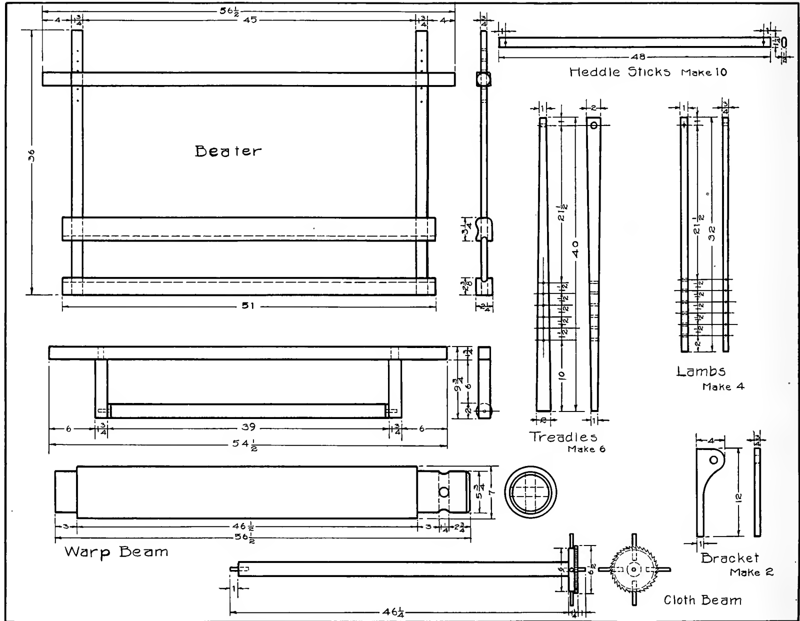
Fig. 431—Working Drawing of Swedish Loom—Details
