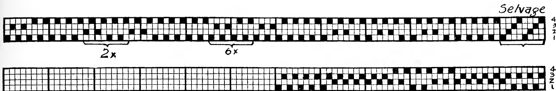
Fig. 161—The Platform. Draft of Pattern
