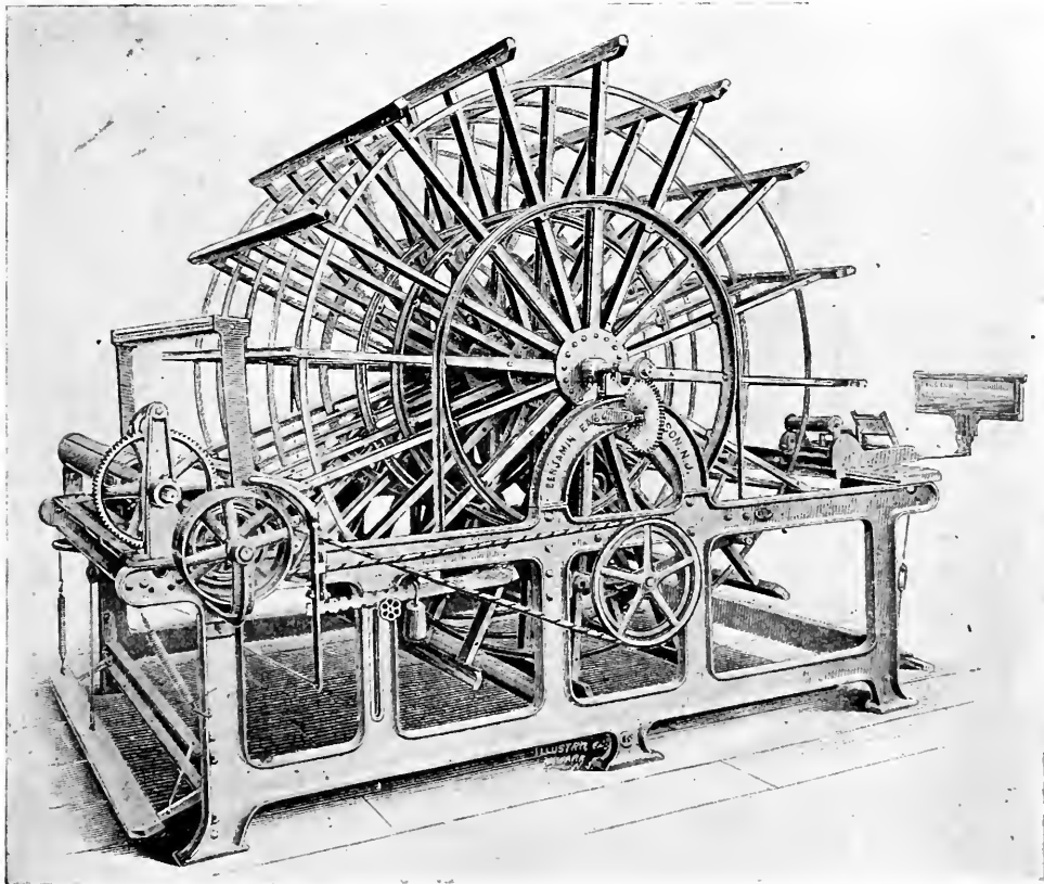
FIG. 10.—Empty Horizontal Warper (without Swiss Attachment).
