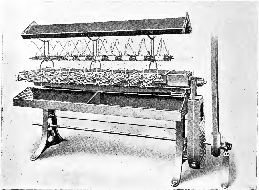
FIG. 16.—High-speed, Underdrive, Quiller.
