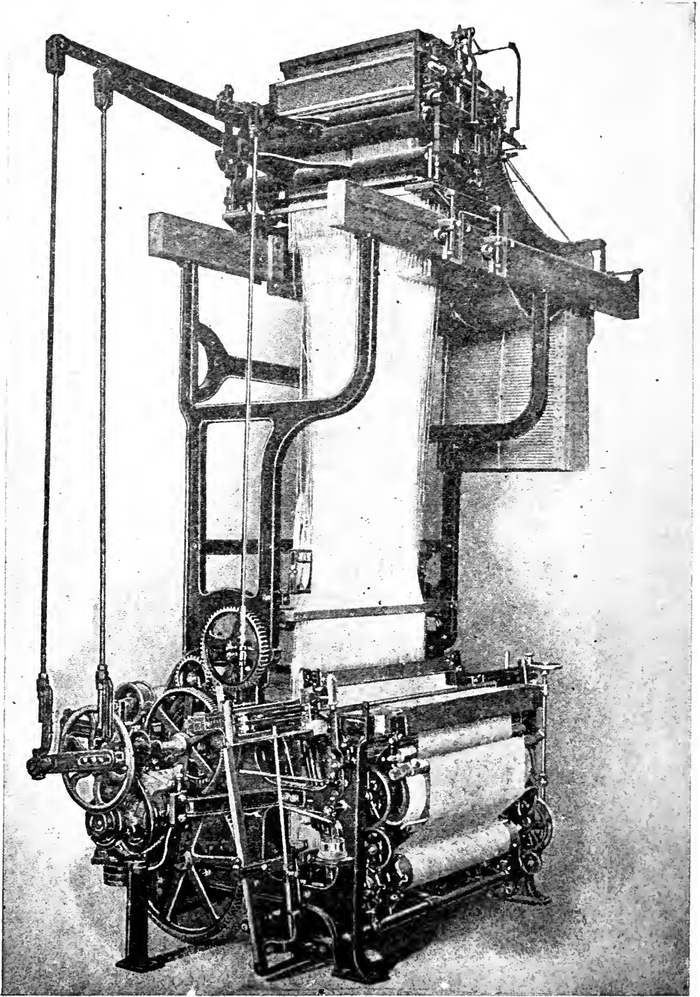
FIG. 19.—Jacquard Silk Loom with Motor Drive.
