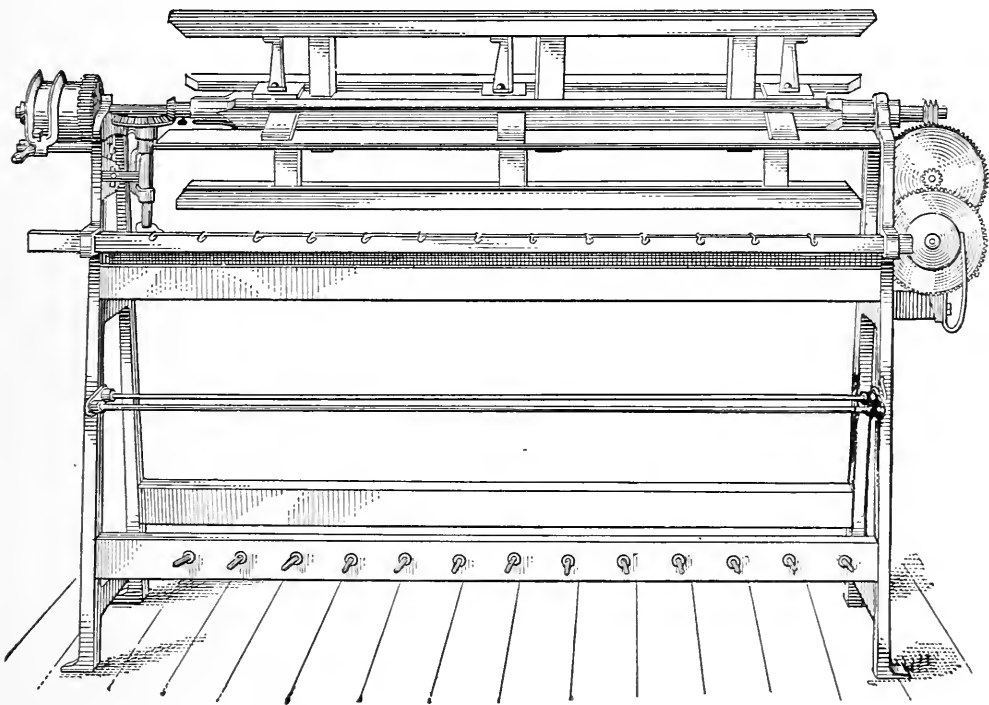
FIG. 20.—Skein Reel, with Single Fly.
