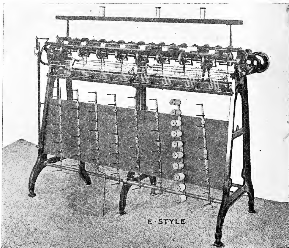
FIG. 17.— Doubling Machine.
