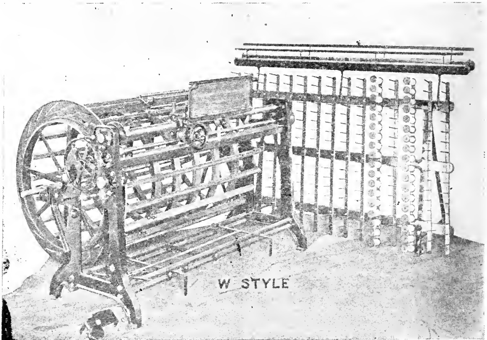
FIG. 6.—Swiss Sectional Warping Frame, and Creel.
