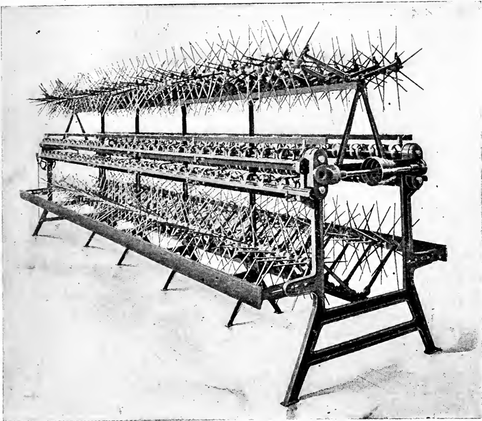
FIG. 2.—Double-deck Winding Machine.
