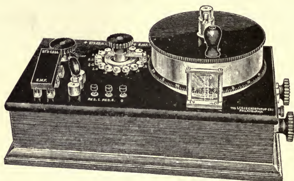
FIG. 113.—The Leeds and Northrup potentiometer (type K).
