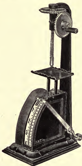
FIG. 66.—The Scott glue tester. (Kindness of The Arthur H. Thomas Company of Philadelphia.)
