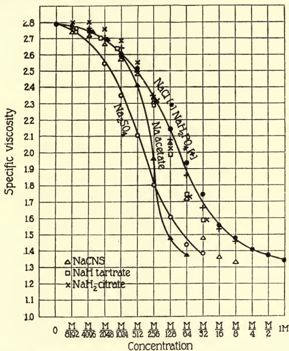
FIG. 46.—The depressing effect of different salts with monovalent anion ( \text{NaCl} , \text{NaH}_2\text{PO}_4 , \text{NaClNS} , \text{NaH tartrate} , and \text{NaH}_2 citrate) on the specific viscosity of 1 per cent solution of gelatin chloride of pH 3.0. The effect of \text{NaCl} and \text{NaH}_2\text{PO}_4 are identical since the pH is not altered by the addition of these salts. The depression in the values for the specific viscosity is greater in the case of \text{Na acetate} than in the case of \text{NaCl} for the reason that the \text{Na acetate} raises the pH of the gelatin solution.
