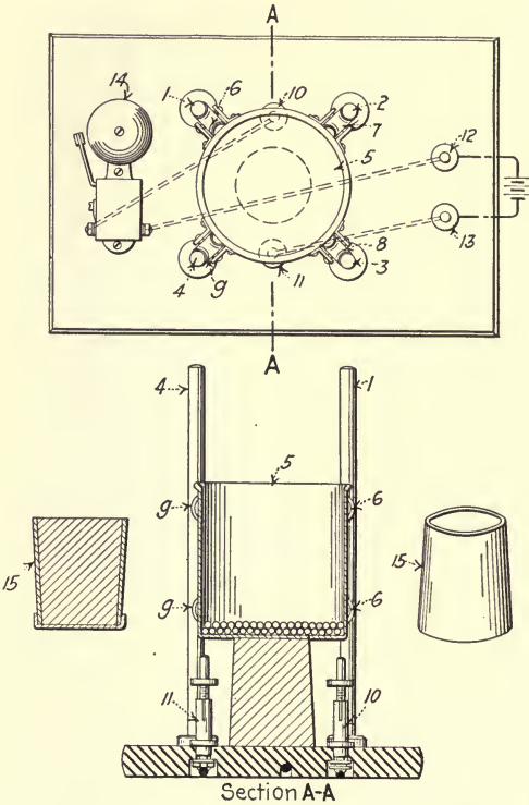
FIG. 67.—Alexander's jelly strength apparatus.
