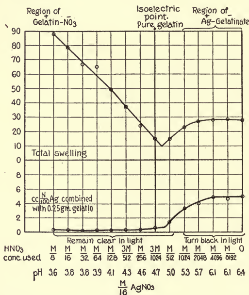
FIG. 35.—Gelatin treated with different concentrations of \text{HNO}_3 , from M/8 to M/8192, washed, and then treated with the same concentration of \text{AgNO}_3 , (M/16), and then washed again.
