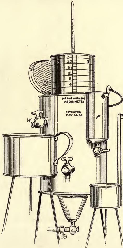
FIG. 77.—Kahrs' viscosimeter glue pot.
