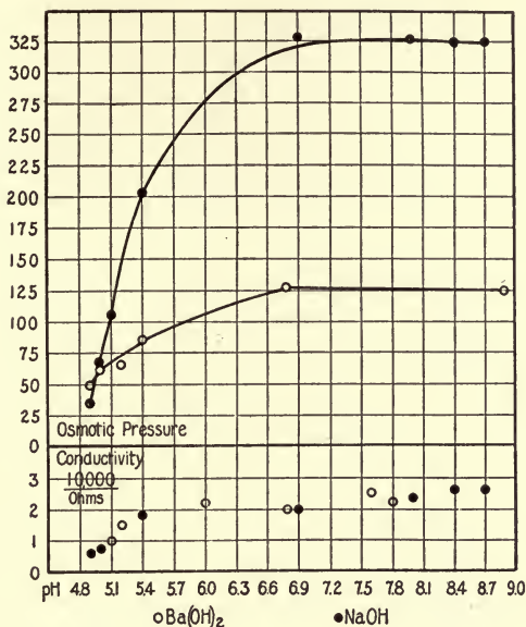
FIG. 40.—Showing that while the curves for conductivity of sodium and barium gelatin are practically identical, the curves for the osmotic pressures are very different.
