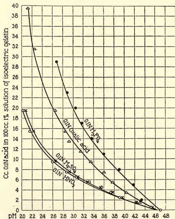
FIG. 37.—Curves for the number of cc. of 0.1N HNO 3 , H 2 SO 4 , oxalic, and phosphoric acids required to bring 1 gm. of isoelectric gelatin to different pH (in 100 cc. of solution).
