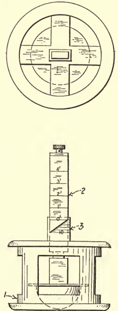
FIG. 68.—Jelly strength tester used by the Forest Products Laboratory.
