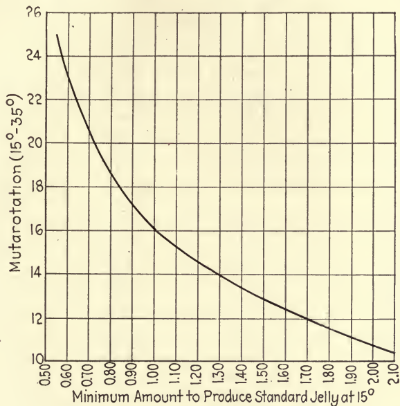
Fig. 97.—Mutarotation and jellying power. (From data of C. R. Smith.)
