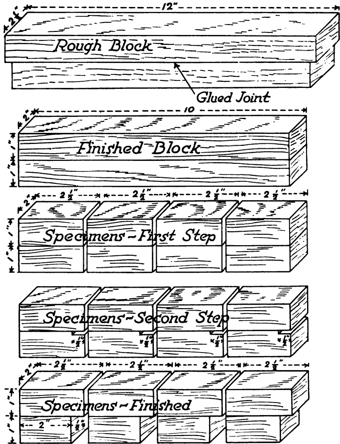
METHOD OF PREPARING SPECIMENS FOR GLUE STRENGTH TESTS
