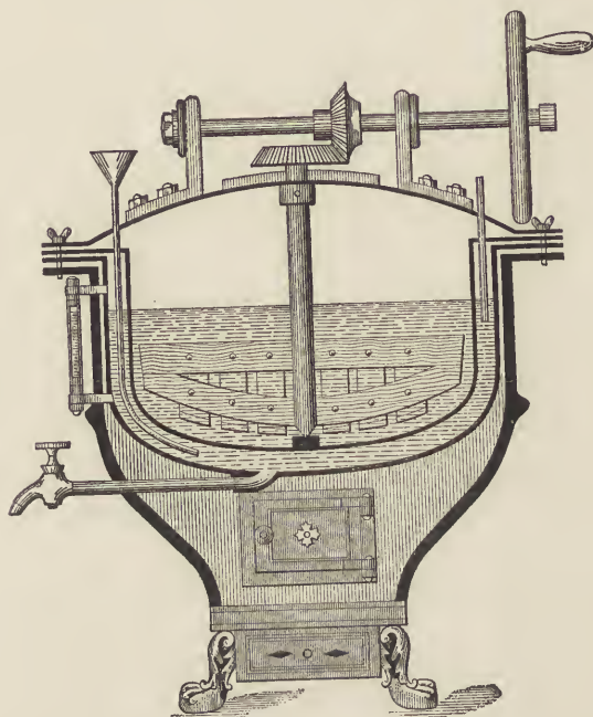
FIG. 24.—Zemsch's Spirit-varnish Apparatus.
