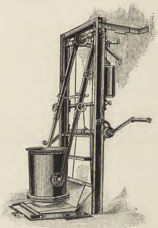
FIG. 21.—Weber's Elevator, First Position.
