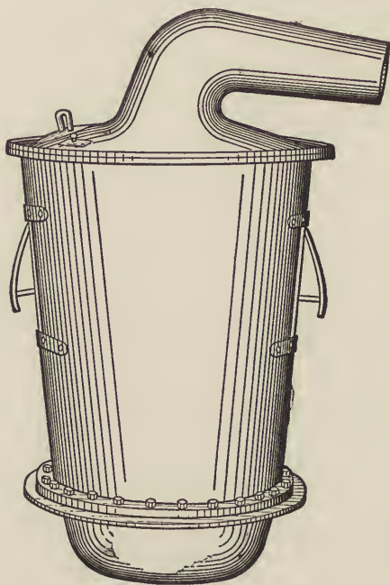
FIG. 14.—Heraeus' Varnish-kettle.
