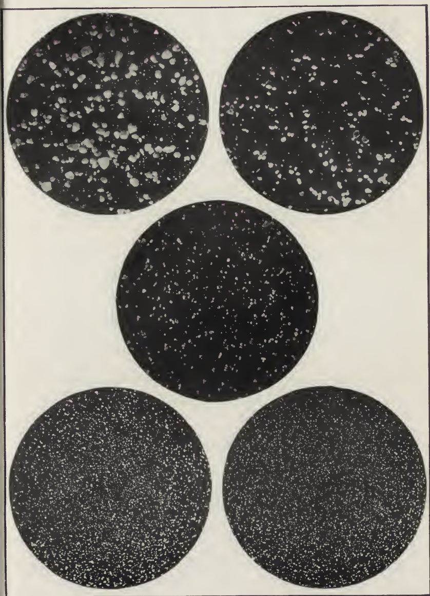
FIG. 45.—Red Lead, \times 40 .
