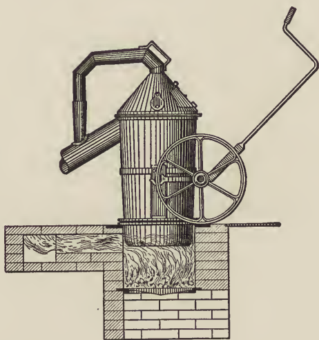
FIG. 18.—Sommer's Kettle, Truck, and Fire.
