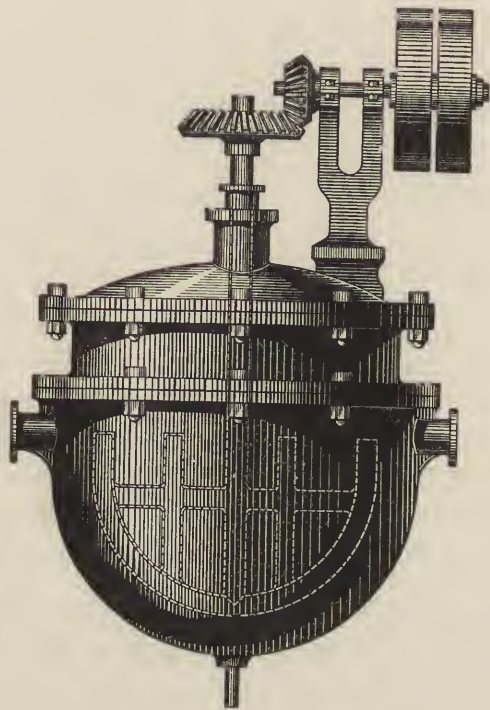
FIG. 11b.—Zemsch's Varnish-kettle.
