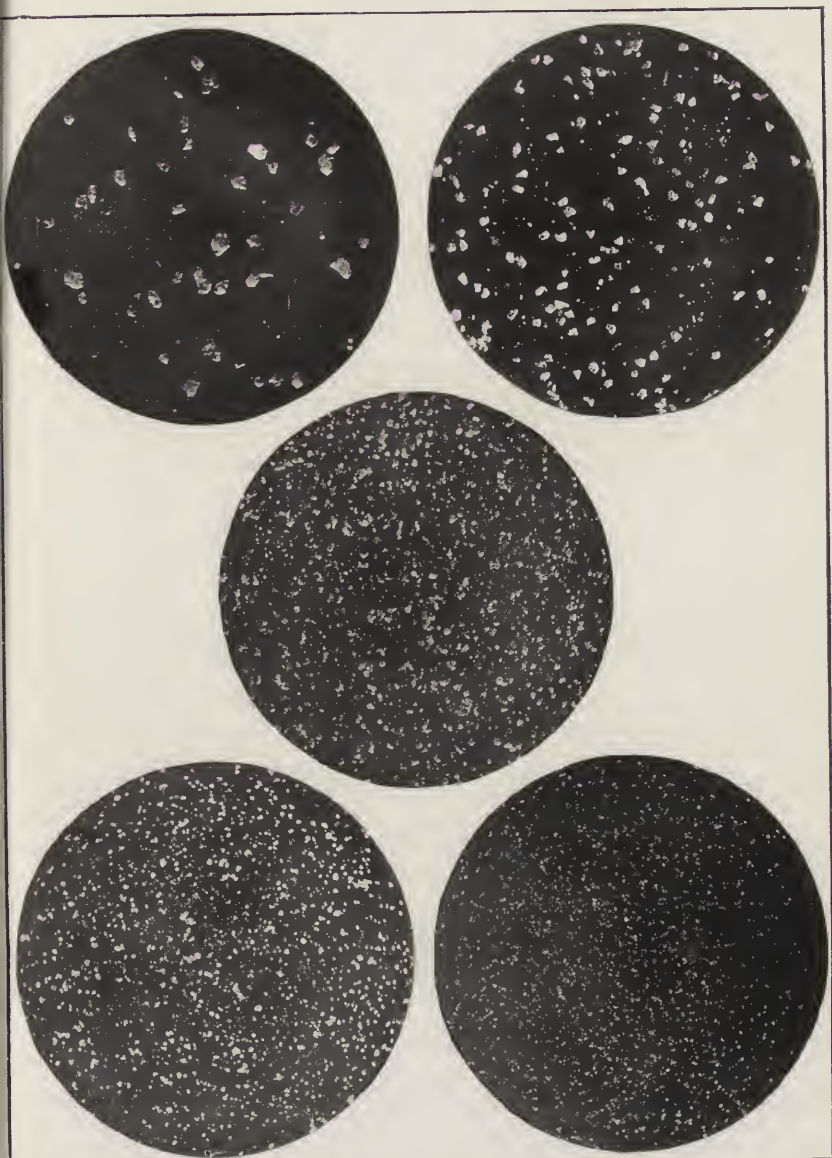
FIG. 47.—Cement, \times 40 .
