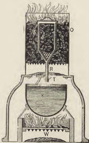
FIG. 9.—Andrès' Apparatus.
