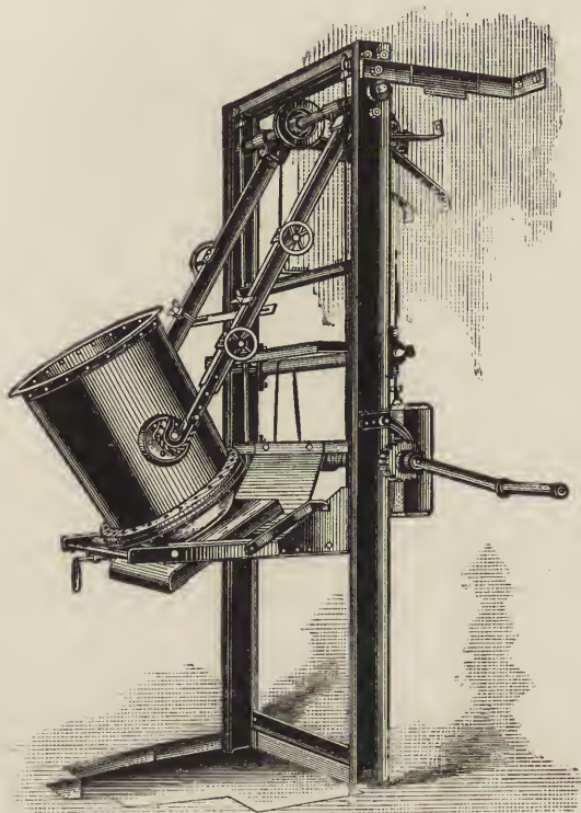
FIG. 22.—Weber's Elevator, Intermediate Position.
