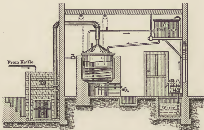
FIG. 8.—Lehmann's Apparatus.
