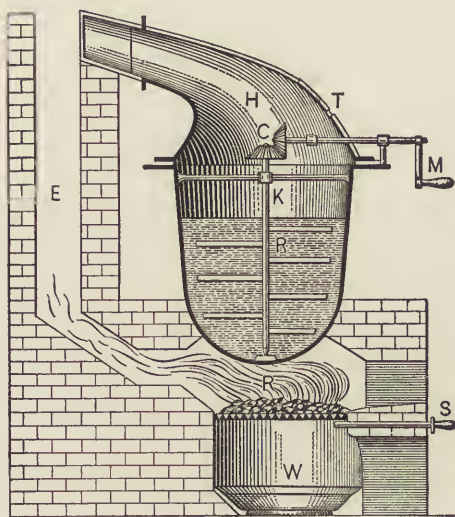
FIG. 6.—Varnish-kettle, According to E. Andrès. The fire, R , may be dumped into the water, W , by pulling out the support, S .
