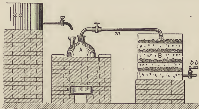
FIG. 25.—Würth's Apparatus.
