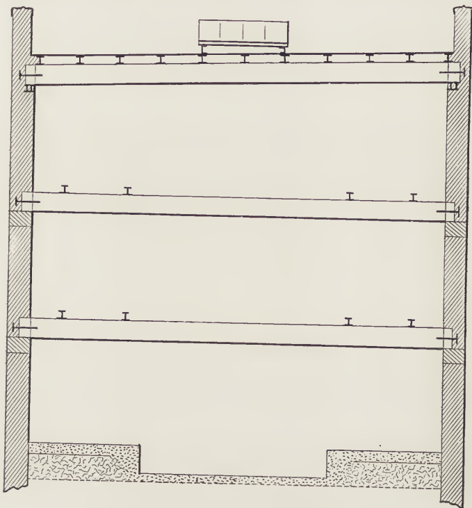
FIG. 48.—Section of a Varnish Storage-Building.
