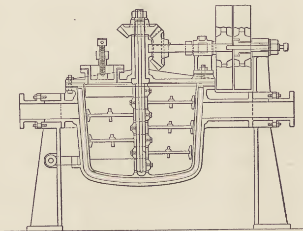
FIG. 11a.—Zensch's Steam-jacketed Melting and Cooking Kettle.
