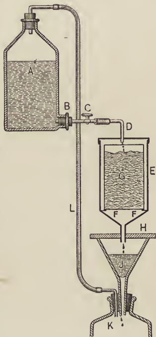
FIG. 27.—Andrès' Filtering Apparatus.
