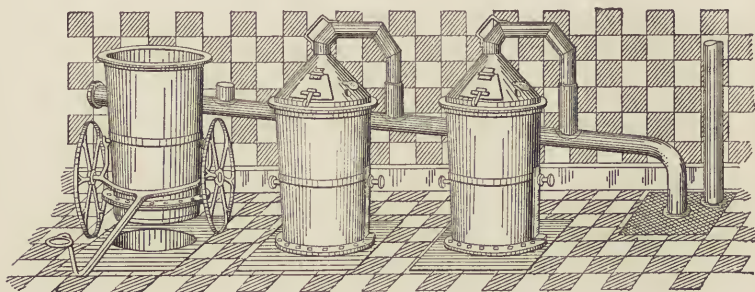
FIG. 19.—German "Varnish-chimney."
