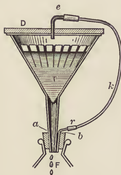
FIG. 26.—Varnish Filter.
