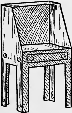
Top and legs cut - Drawer front fastened
