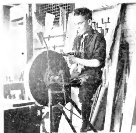
Grinding Tool on Grindstone using Tool Holder.
