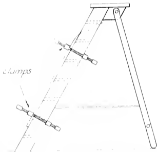
VIEW SHOWING METHOD OF BENDING AND HOLDING RUNNERS WITH CLAMPS
