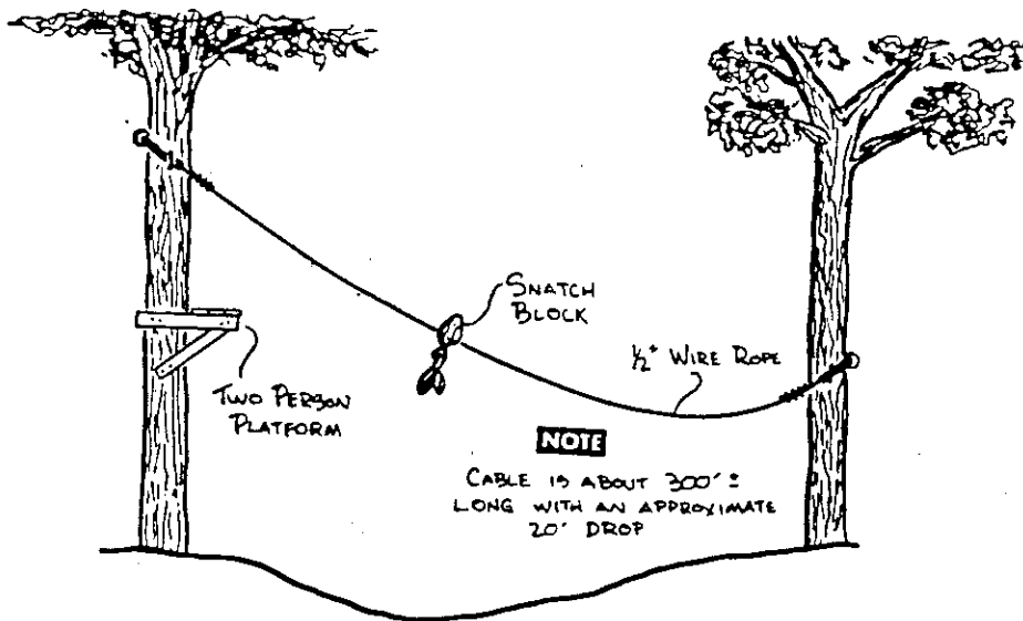
G. The Aerial Runway
