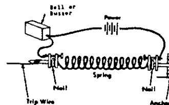
Figure 385 Tension Release Device Booby Trap
