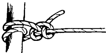
Figure 139 The Round Turn and Two Half Hitches
