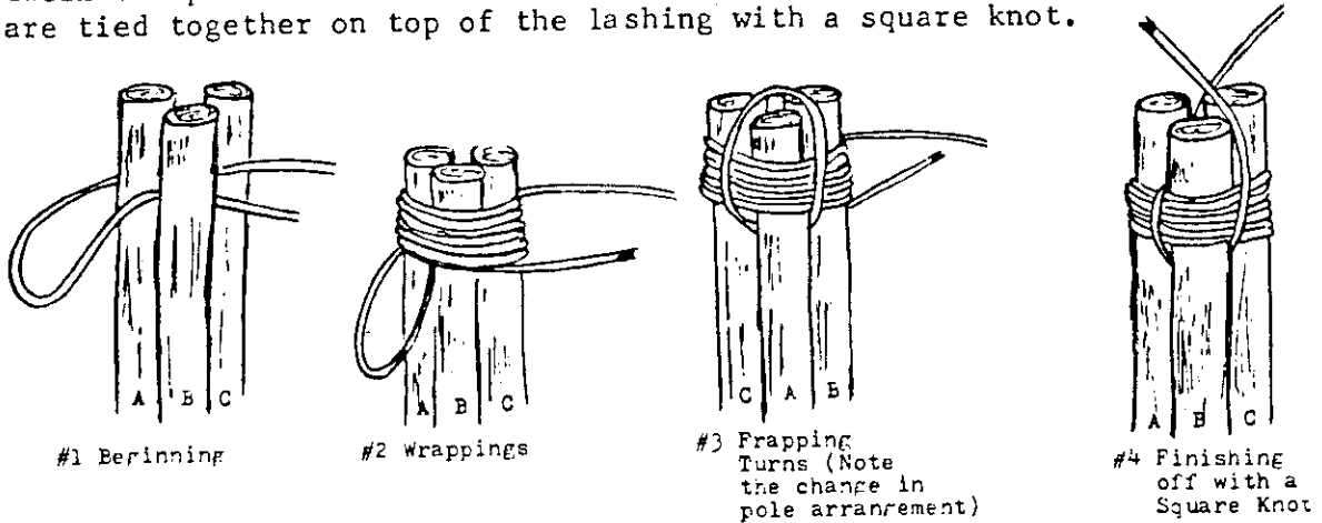
Figure 181 The Sailmaker's 3 Pole or Tripod Lashing
