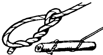
Figure 122 The Timber Hitch
