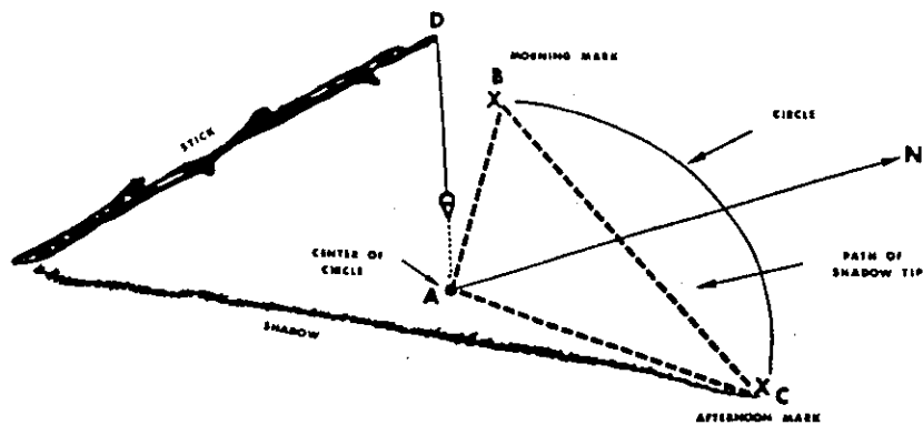
Figure 368 The Plumb Bob Method
