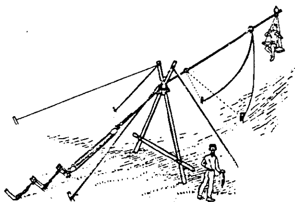
K. A Brake System for an Aerial Runway
