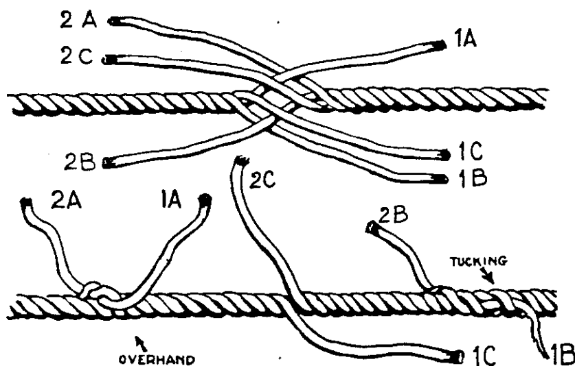
Figure 173 The Long Splice
