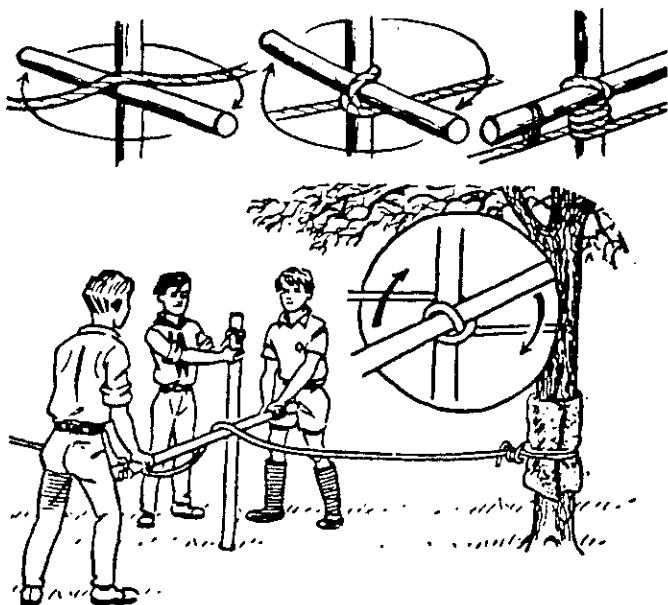
Figure 195 The Spanish Windlass
