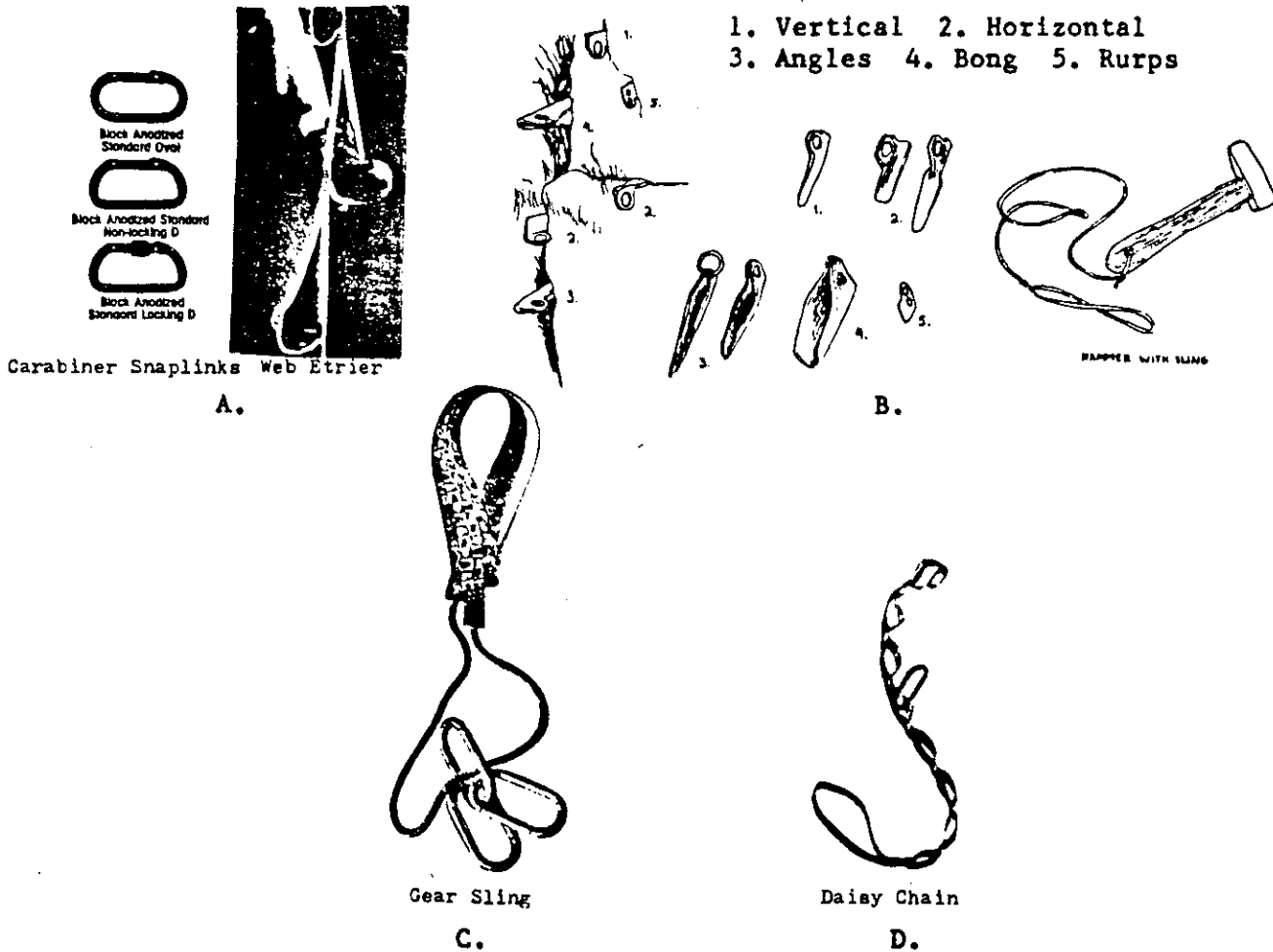
Figure 210 Rope Climbing Equipment
