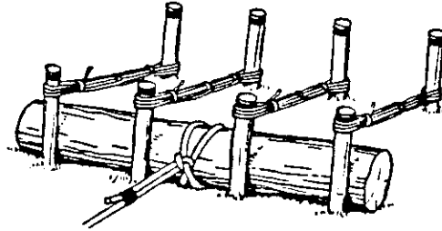
Figure 189 Log and Picket Holdfast
