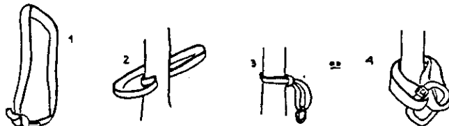
Figure 245 One Type of Anchor for Anchoring the Belayer
