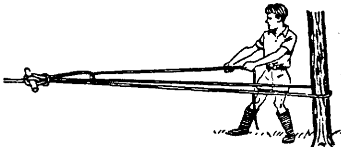
The Harvester's Figure 196 or Hayman's Hitch
