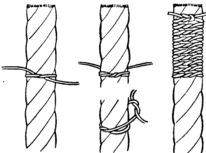
B. The American Plain Whipping
