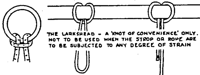
The Girth Hitch or The Larkshhead
