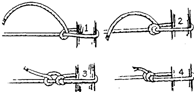
Figure 124 The Tautline Hitch
