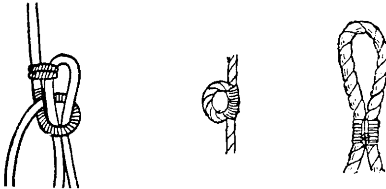
Figure 183 Rope Seizings
