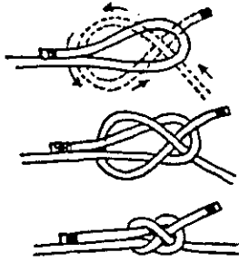
Figure 134 The Sheet Bend
