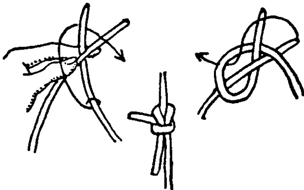
Figure 137 The Weaver's Knot
