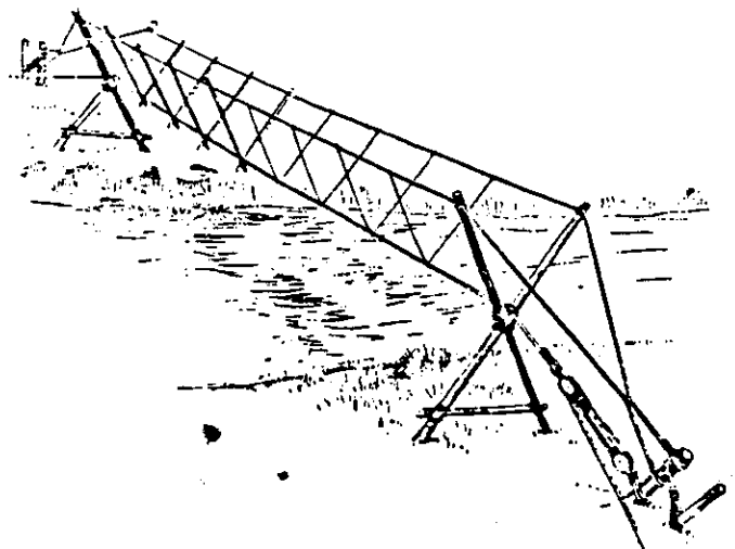
Figure 263 A Three Rope Monkey Bridge
