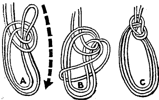
Figure 153 The Bowline on a Bight
