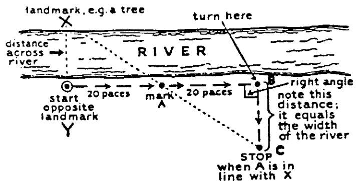
Figure 356 Stick Method of Determining Width
