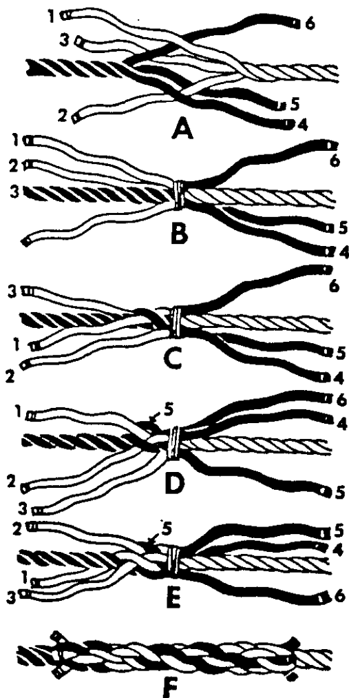
A. Short splice
