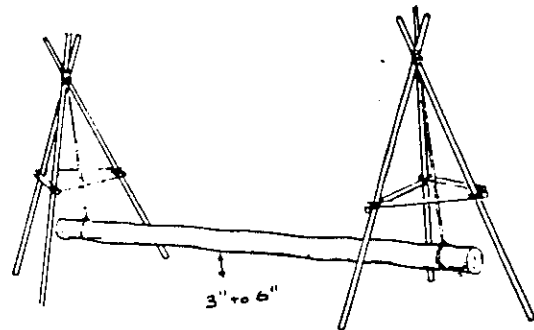
Figure 412 The Floating Log
