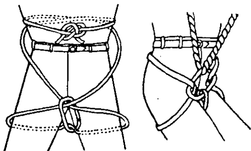
Figure 223 One Type of Diaper Sling
