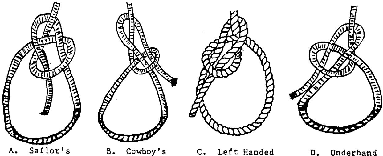
Figure 150 The Bowline
