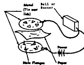
Figure 382 Pressure Device Booby Traps
