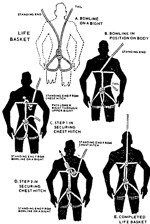
Figure 249 Details for Making a Life Basket for Rescue Operations
