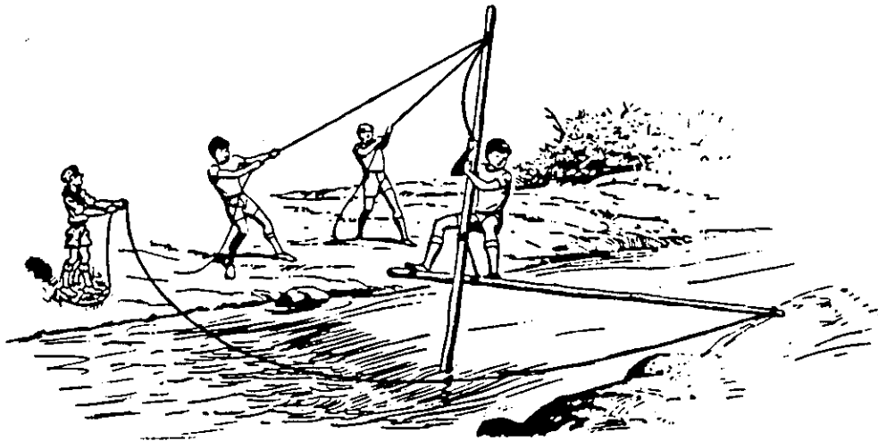
Figure 252 The Kickbridge
