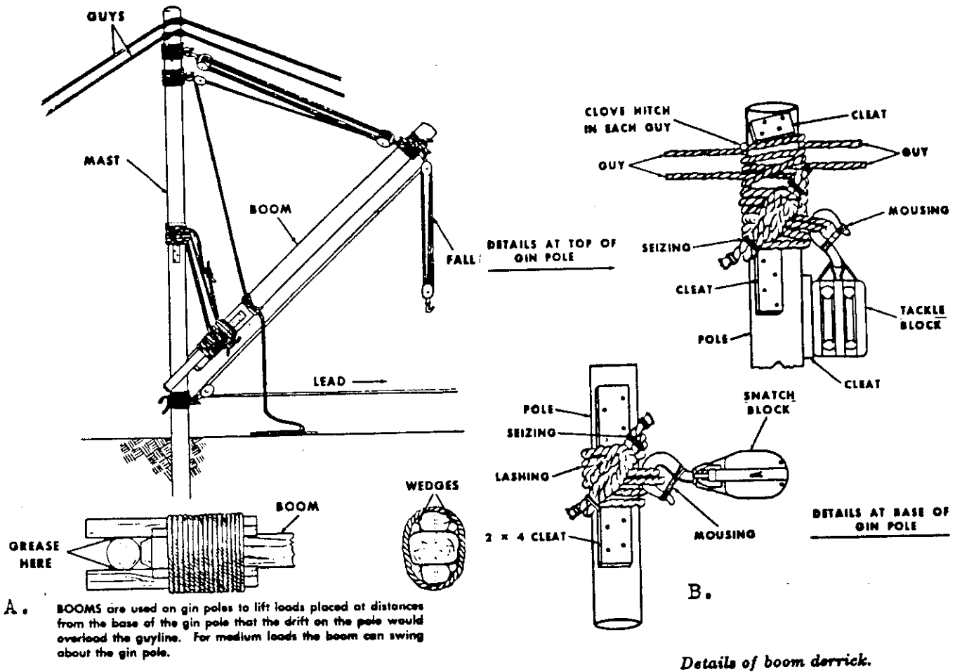
Figure 97 Boom Derrick
