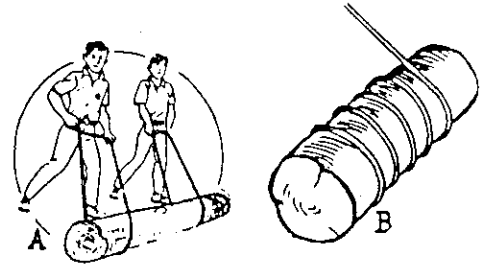
Figure 403 The Gun Tackle
