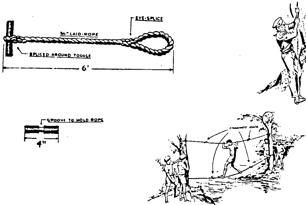
Figure 247 Using the Commando Rope (Toggle Rope)
