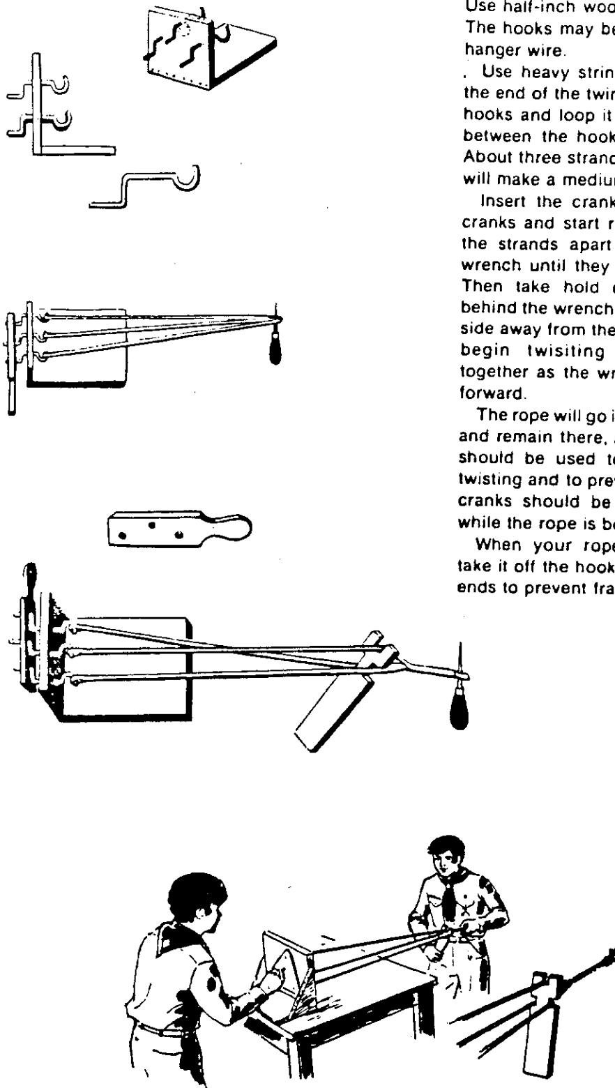
Figure 107 The Rope Crank
