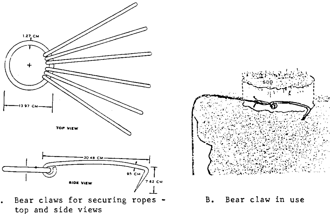
Figure 191 The Bear Claw
