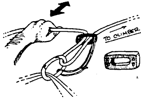
Figure 237 Method of Using the Stitch Belay Plate for Belaying
