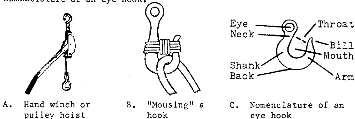
Figure 192 The Hoist
