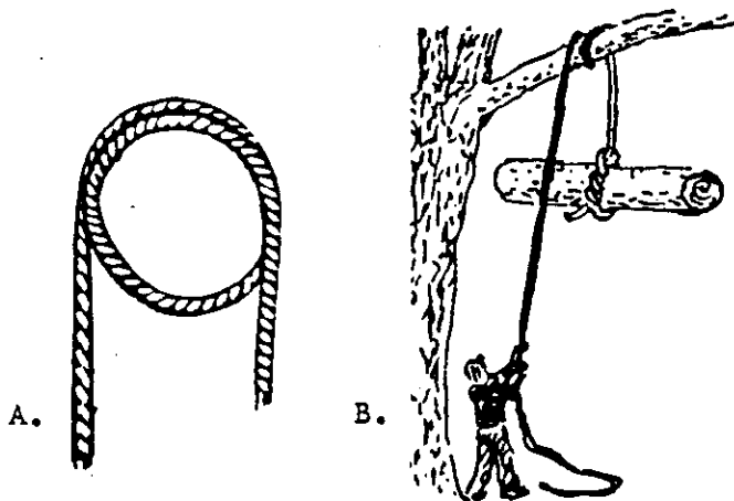
Figure 111 The Round Turn
