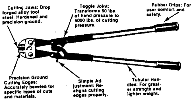
Figure 72 Bolt Cutters
