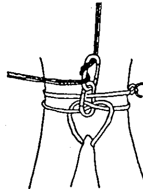
Figure 222-B The Rappel Rope Snaplink Attachment for the Seat-Hip Rappel
