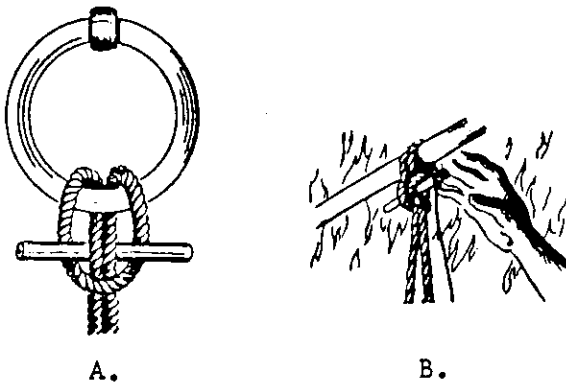
Figure 159 The Larkshead with a Toggle
