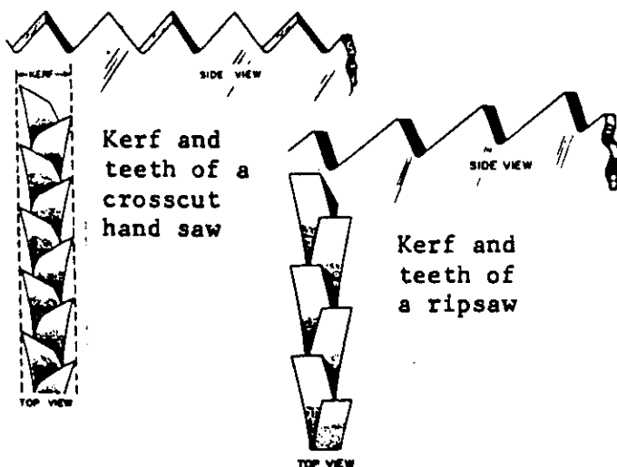
Figure 48-A The Teeth and Kerf of a Hand Saw
