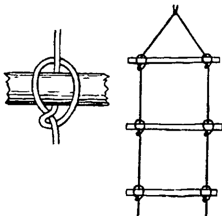
Figure 161 The Marline Spike Hitch
