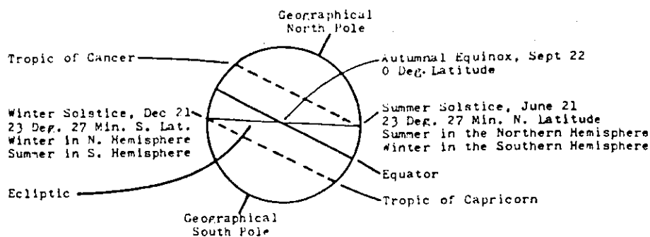
Figure 369 The Ecliptic and Shadow Phenomenon in the Torrid Zone
