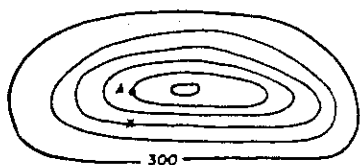
Figure 277-A Intermediate Contour
