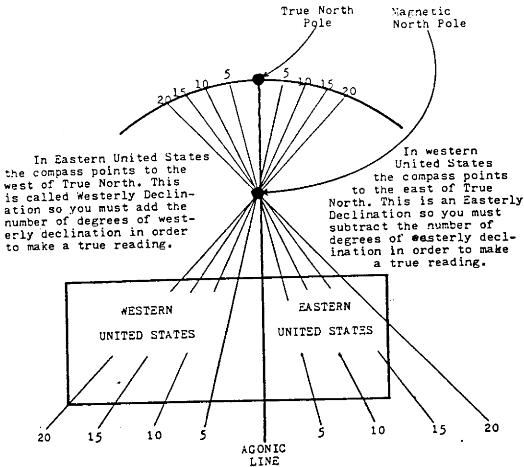
Figure 280-B Schematic drawing to Aid in Understanding Easterly and Westerly Declination (Variation).
