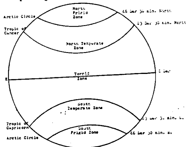
Figure 266 The Five Zones of the Earth With the Latitudinal Divisions of the Earth's Surface
