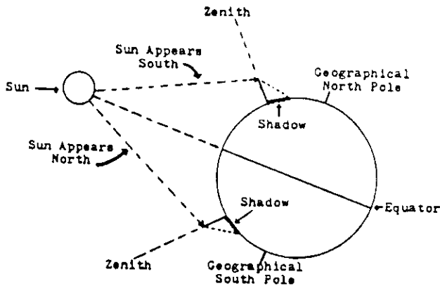
Figure 366 The Sun in Relation to the North and South Hemispheres
