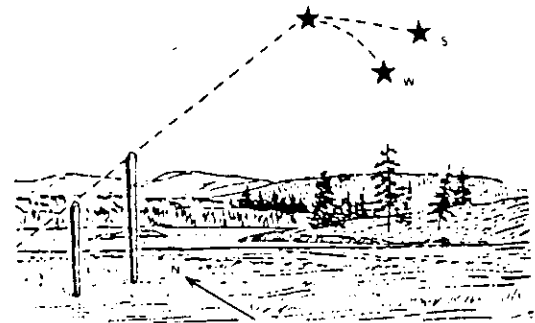
Figure 374 Finding Directions Using Any Star
