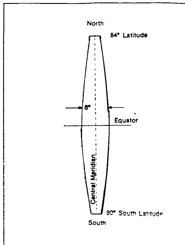
Figure 273 The Shape of an Individual Universal Traverse Mercator Zone
