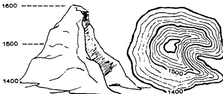
Figure 275 Depiction of a Hill Above Sea Level
