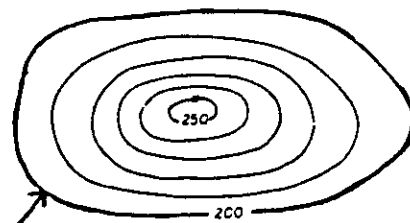
Figure 276 Index Contour
