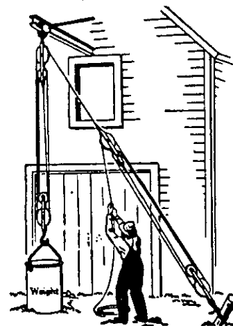
MA Equals 20 Figure 84-F
