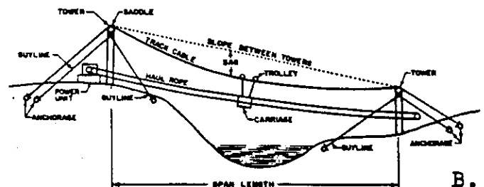
Nomenclature of components of a cableway system.
