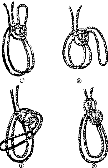
c. The Bowline on a Bight Also called the Man Sling
