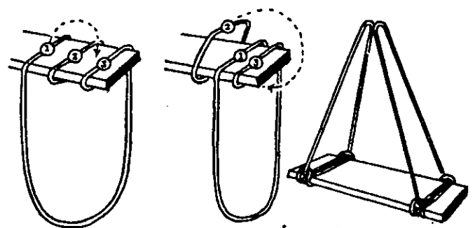
F. Using A Scaffold Hitch to Make A Boatswain's Chair
