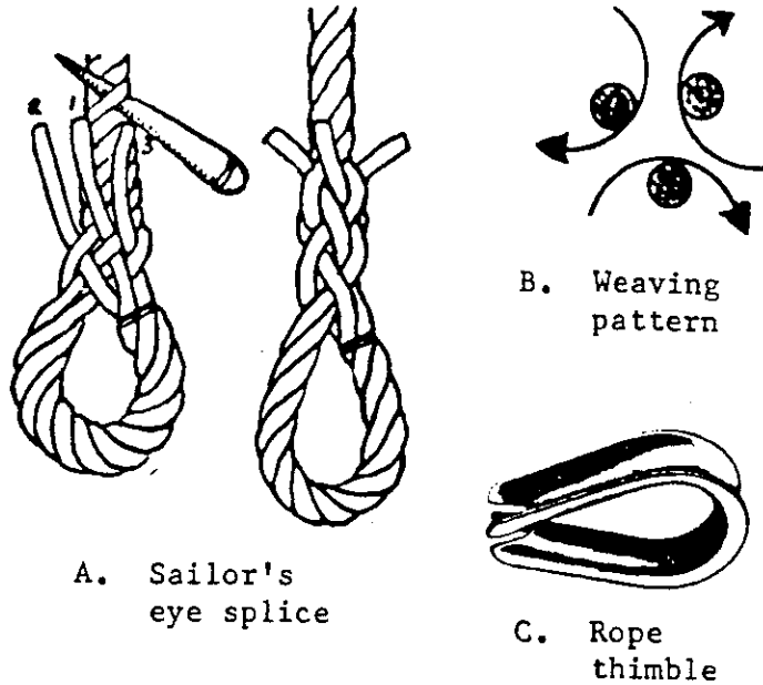
Figure 170 Sailor's Eye Splice
