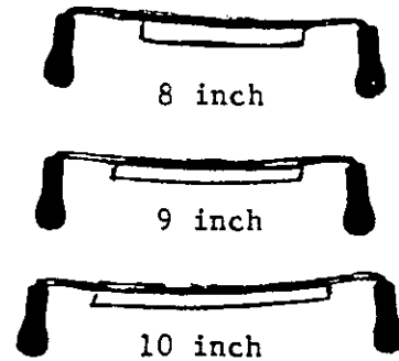
Figure 68 Drawknife
