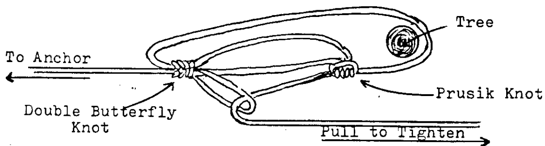
Figure 197 The Double Butterfly-Prusik Tightening Arrangement
