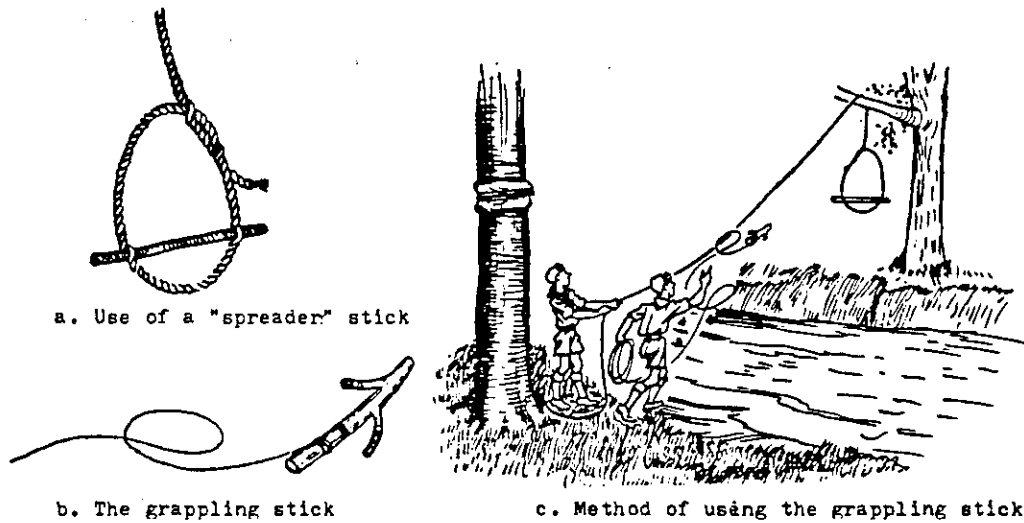
Figure 254 Using a Grappling Stick to Get a First Line Across for a One Rope Bridge
