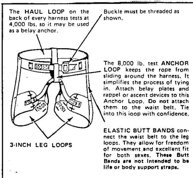
Figure 225 A Commercial Seat Harness
