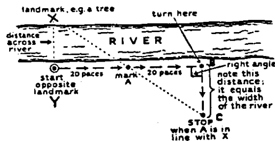
Figure 433 Determining the Width of a River
