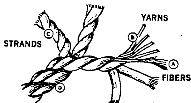
Figure 98 Twisted Rope
