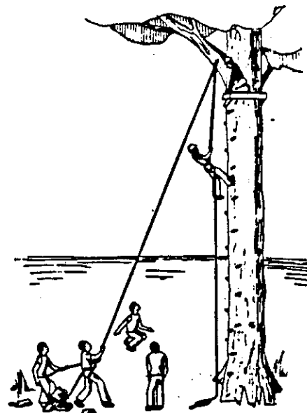
Figure 235 Belaying a Climber Rappelling Down a Large Tree Trunk With a Lower Belay
