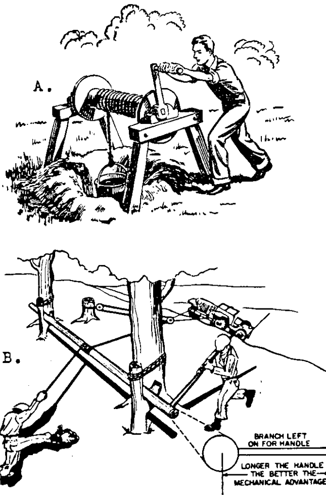
Figure 95 Windlass
