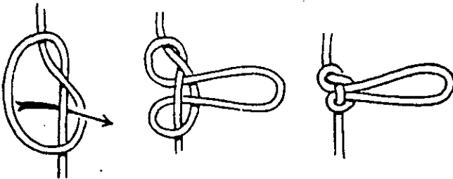
Figure 147 The Man Harness Knot
