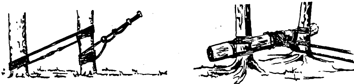
Figure 184 Two Types of Natural Tree Anchorages
