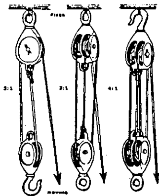
Mechanical Advantage Figure 84-D
