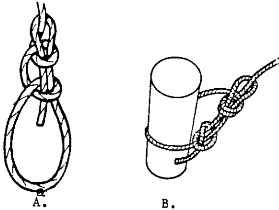
Figure 151 The Water Bowline
