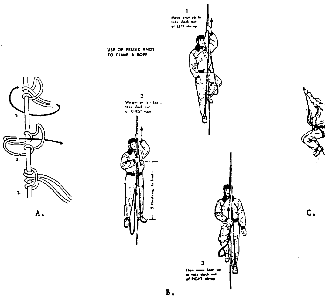
Figure 209 Prusiking
