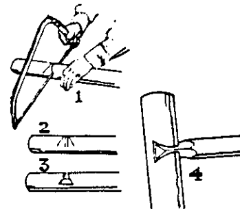
Figure 402 The Dove Tail Notch
