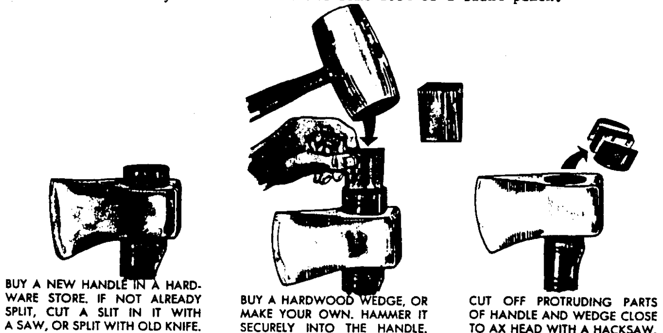
Figure 23 Wedging the Handle
