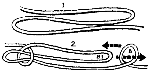
Figure 140 The Sheepshank
