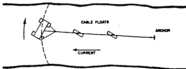
Figure 307 The Flying Ferry
