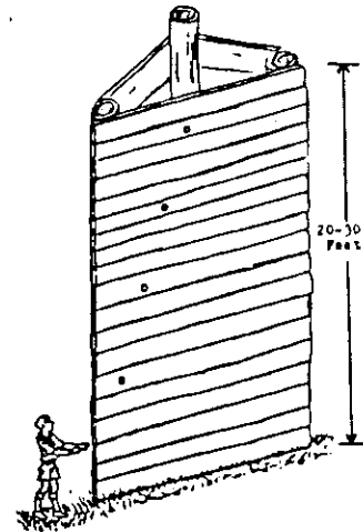
Figure 233 A Rappel Wall With 3/8" Eye Bolts Simulating Pitons Used For Tension Climbing
