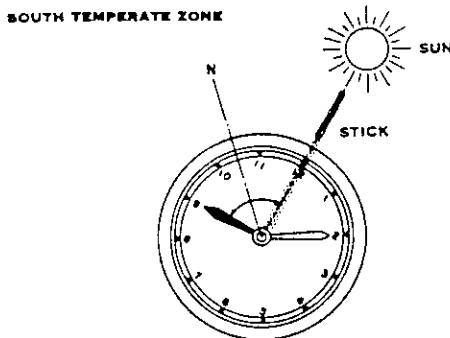
Figure 359 Sun and Watch Method of Finding North in the South Temperate Zone
