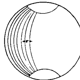
Figure 271 A Universal Transverse Mercator Zone
