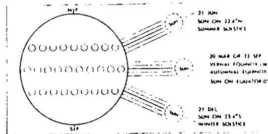
Figure 357 Position of the Sun at Equinox and Solstice
