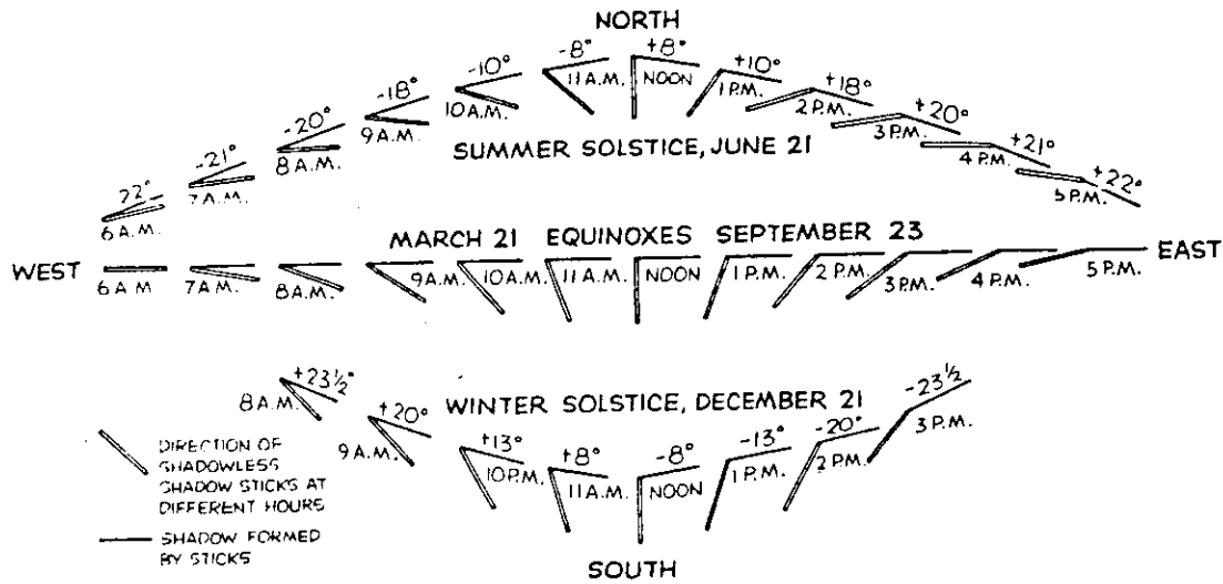
Figure 361 Diagram Showing How Shadows Cast by the Shadowless Stick Method Fall at Different Times of the Day and at Different Times of the Year
