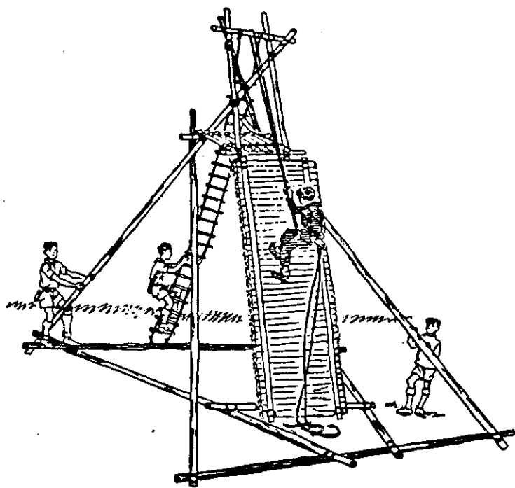
Figure 231 An Easy To Build Beginners Climbing or Rappelling Wall
