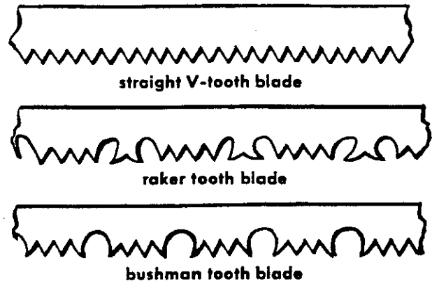
Figure 57 Bow Saw Blades
