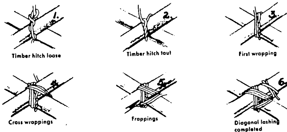
Figure 176 The Diagonal Lashing
