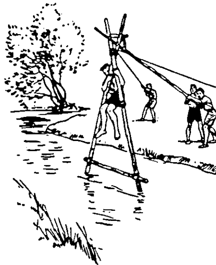
Figure 430 Shear Movement
