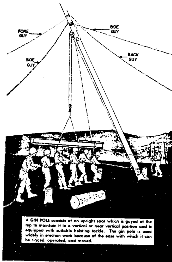
Figure 89 Hoisting With a Gin Pole
