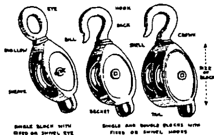
Figure 84-B Nomenclature of Blocks
