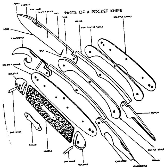
Figure 4 Nomenclature of the Pocket Knife
