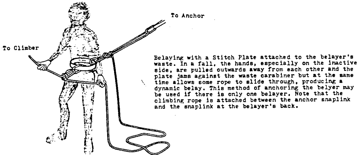
Figure 244 Securing Belay Rope Between the Belayer and Belayer's Anchor
