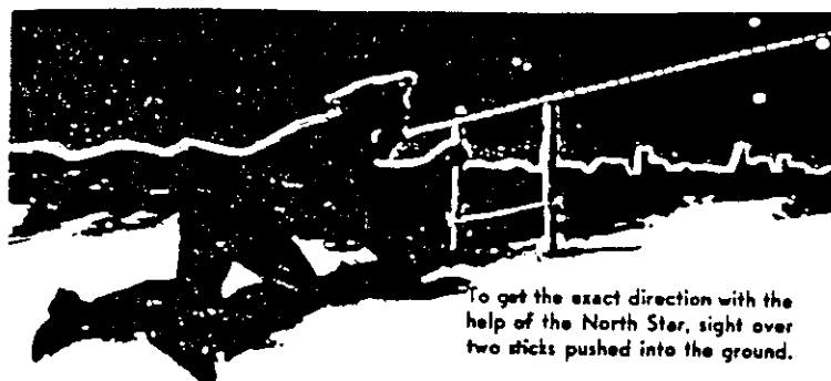
Figure 372 Using Pointer Sticks to Polaris to Make a Daytime North-South Line
