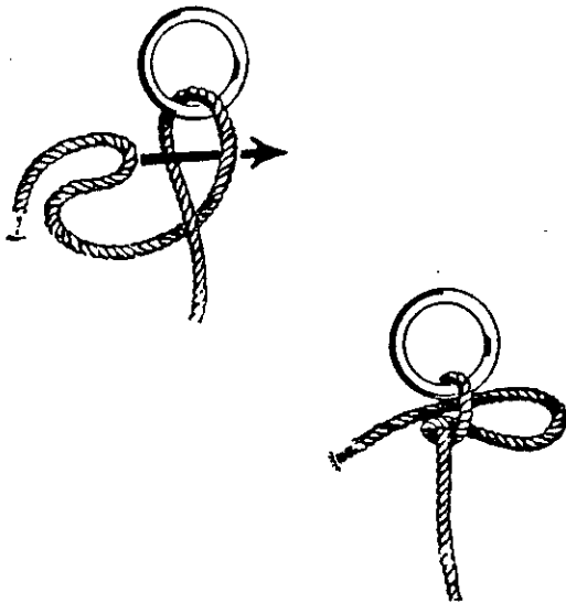
Figure 118 The Slippery Half Hitch
