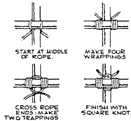
Figure 175 The Japanese Square Lashing
