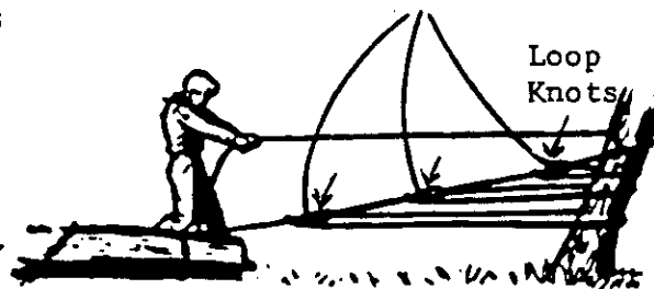
Figure 198 Lumberjack's pulley
