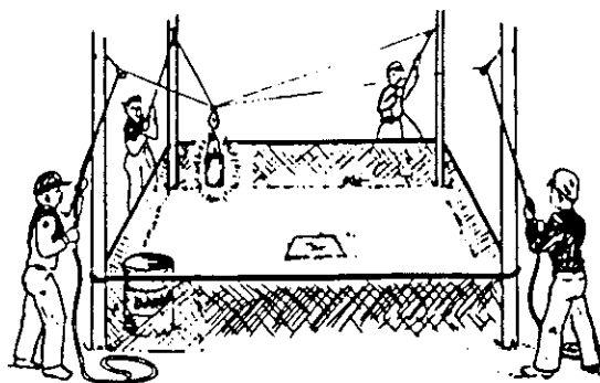
Figure 435 The Red-Hot Isobar
