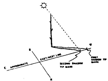
Figure 362 The Shadow Tip Method
