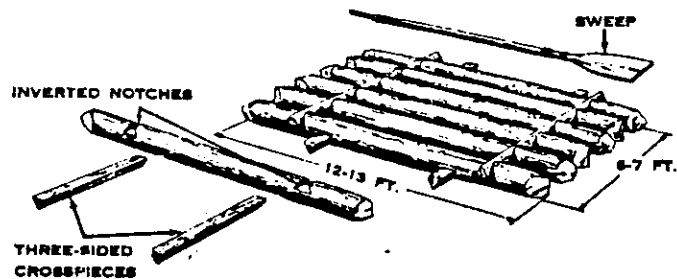
Figure 305 A Rugged Log Raft Developed by Northern Woodsmen
