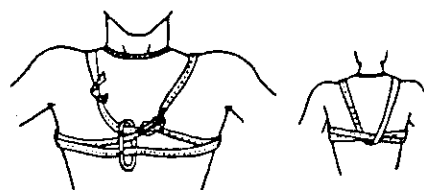
Figure 230 Another Method of Improvising a Chest Harness Using 3/8" Manila or Nylon Rope or Webbing
