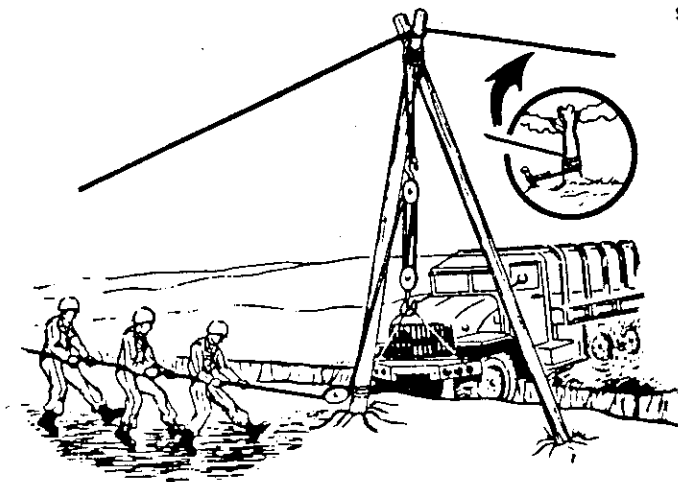
Figure 90 Use of an "A" Frame
