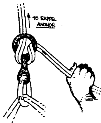
Figure 226 Straight-Figure-8 Descender-Belay Device with the Hook-Up From the Rappel Seat to the Rappel Rope
