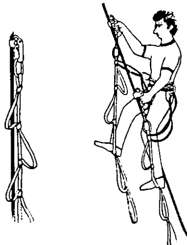
Figure 214 Using Jumar Ascenders
