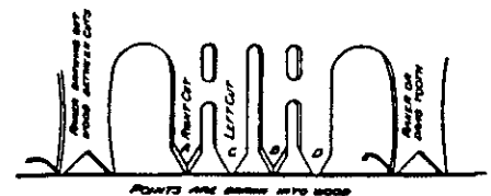
Figure 48-B The Pulp Blade (Lance-Tooth) of a Timber Saw Showing the Work Done by the Cutting Teeth and Rakers
