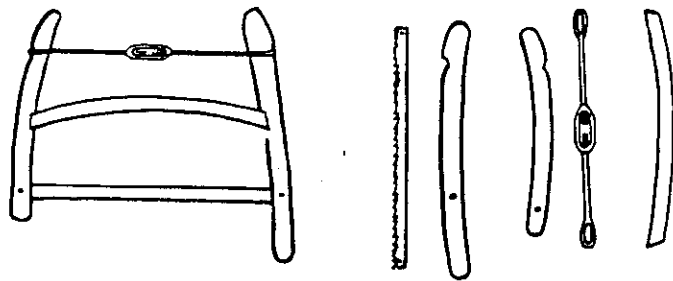
Figure 52 The Five-Piece Bucksaw
