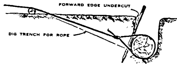
Figure 190 Deadman Anchorage
