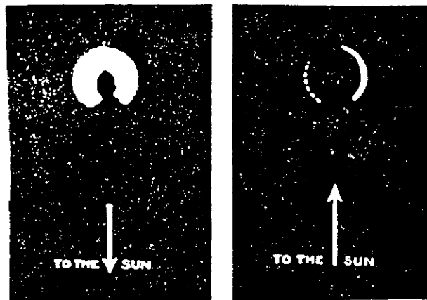
Figure 376 Finding Directions Using the Moon
