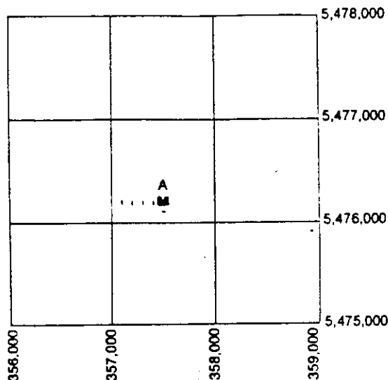
Figure 274 Reading a Map Reference
