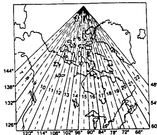
Figure 272 UTM Zones and Central Meridians for Northern United States and Canada
