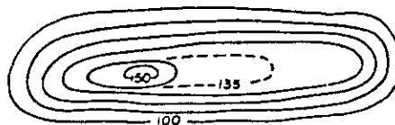
Figure 277-B Supplementary Contour
