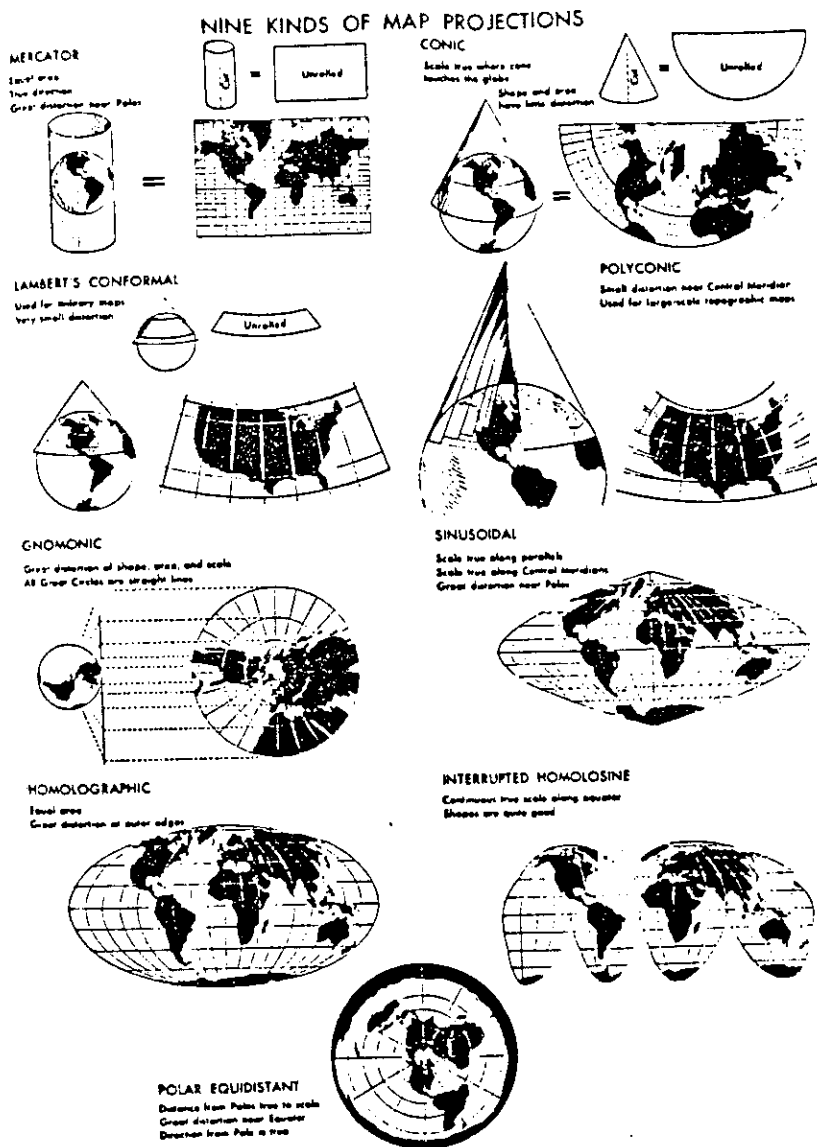
Figure 265 Nine Kinds of Map Projections
