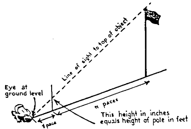
Figure 354 One In Twelve Method of Determining Height
