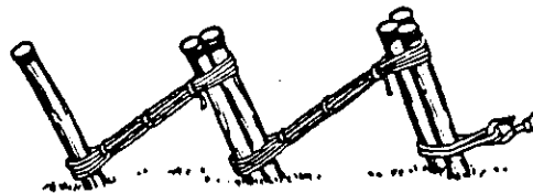
Three-Two-One Figure 188 Picket Holdfast
