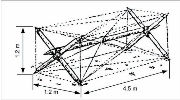
Figure 052-195-3066-4. Knife rest
