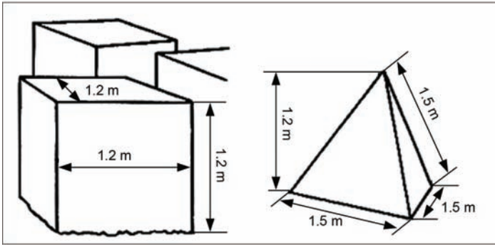
Figure 052-195-3066-8. Concrete Cubes and tetrahedron
