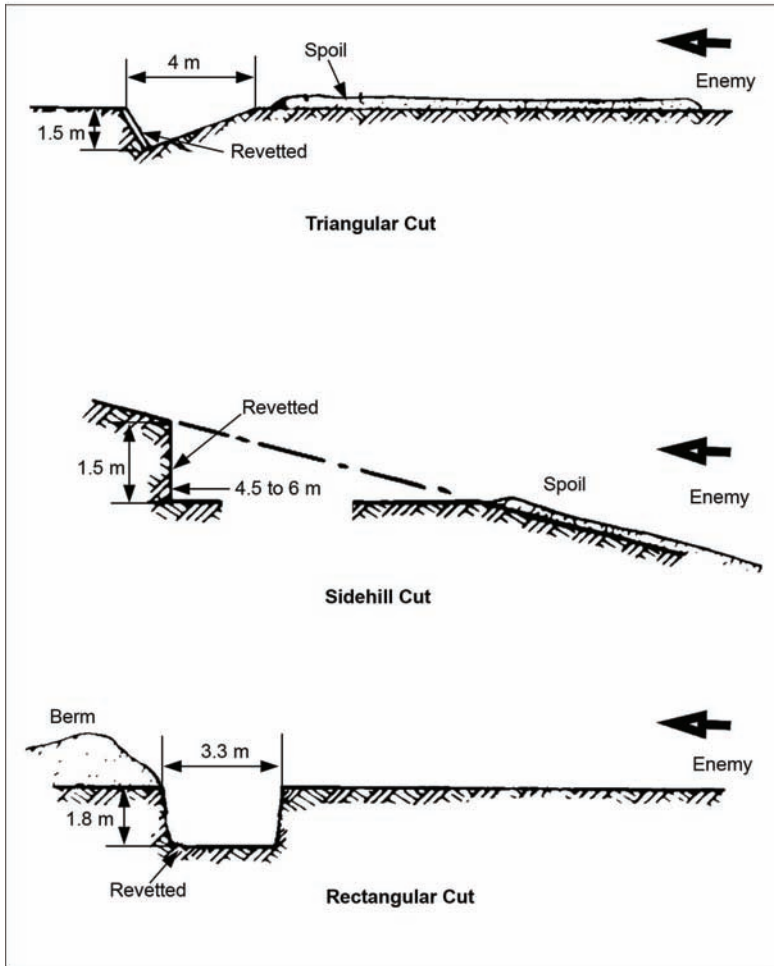
Figure 052-195-3066-6. AT ditch obstacles
