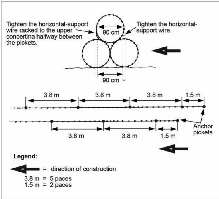
Figure 052-195-3066-1. Triple-standard concertina fence
