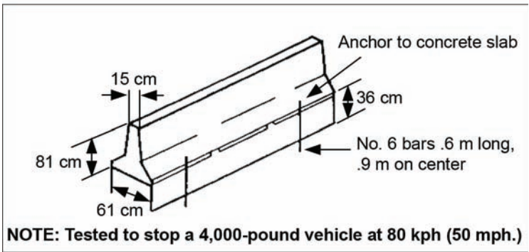
Figure 052-195-3066-9. Jersey barrier
