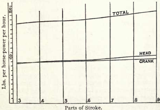
Steam in Cylinder. (Buckeye Engine.)
