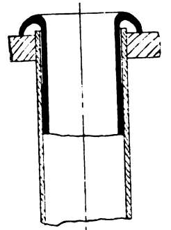
FIG. 36.—Ordinary Tube.
