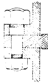
ENLARGED VIEW OF TUBE PLATE JOINT
