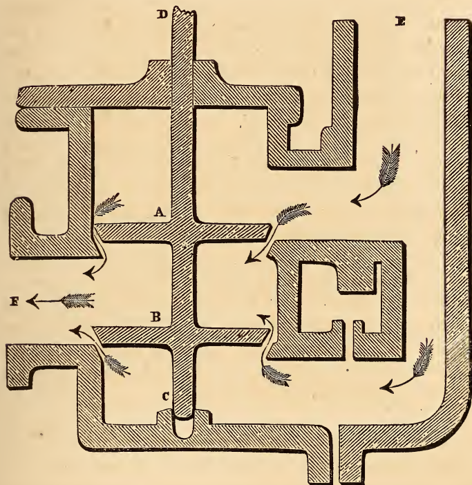
147. Equilibrium-valves as fitted to H.M.S. Penelope.
