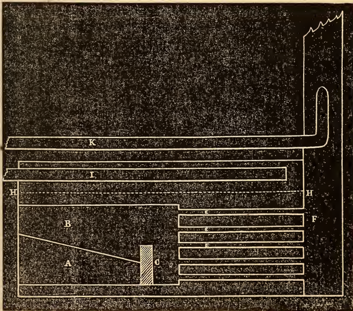
71. Gun-boat Boilers.
