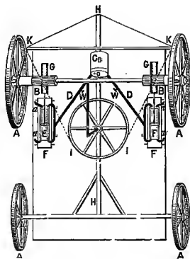
FIG. 43.—Read's Steam-Carriage, 1790.
