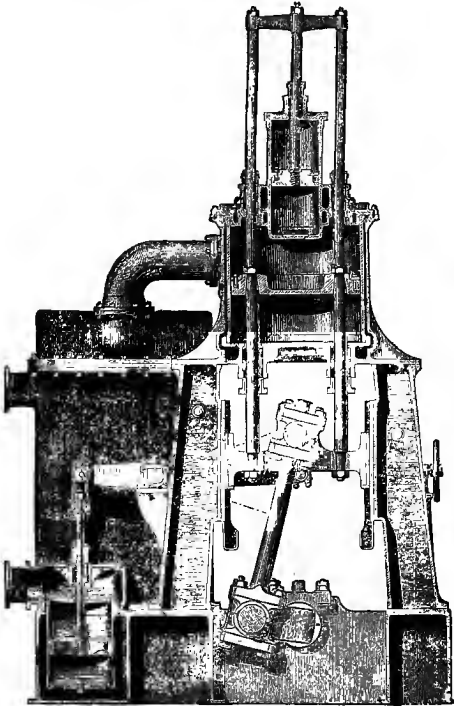
FIG. 155.—Tandem Compound Engine. (Scale \frac{1}{16} .)
