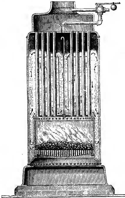
FIG. 103.—Babcock & Wilcox's Vertical Boiler.
