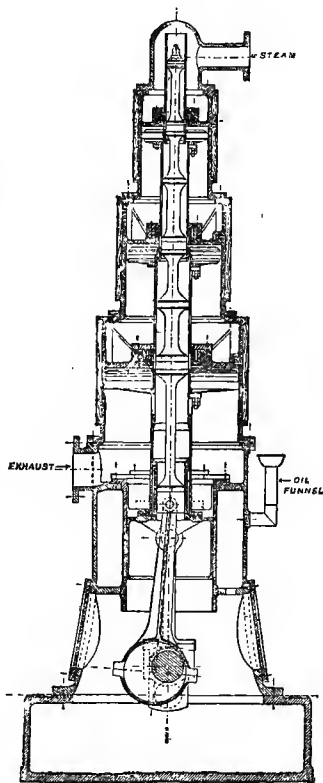
FIG. 165.—Central-Valve Engine.
