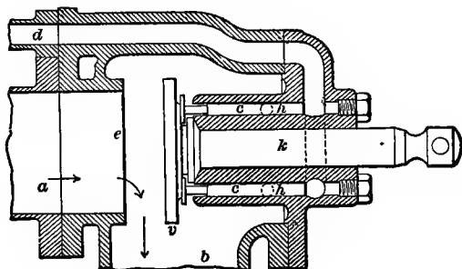
FIG. 150.—“Intercepting Valve.”
