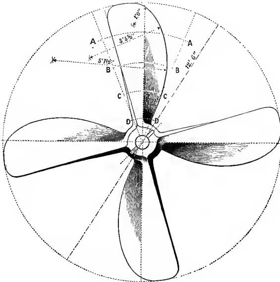
FIG. 139.—Screw-Propeller.
