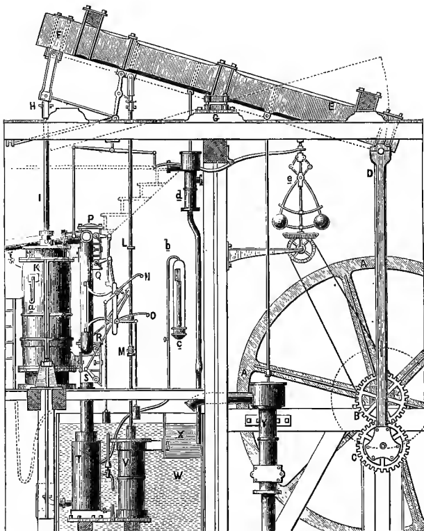
FIG. 27.—Watt's Engine, 1781.
