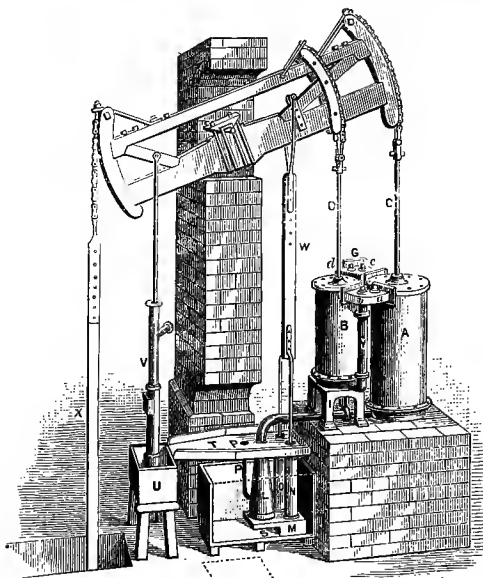
FIG. 37.—Hornblower's Compound Engine, 1.81.
