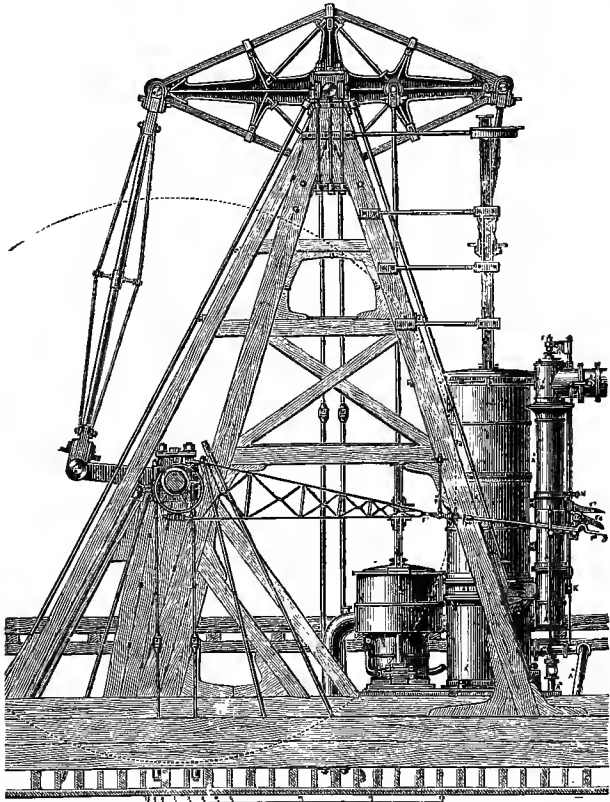
FIG. 130.—Beam-Engine.
