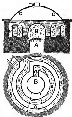
FIG. 22.—Boiler of Newcomen's Engine, 1769.
