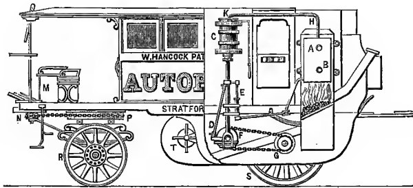
FIG. 49.—Hancock's "Autopsy," 1833.
