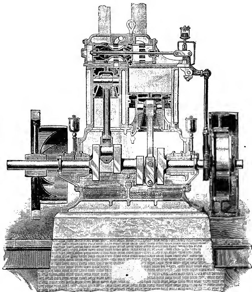
FIG. 164.—Single-acting Compound Engine. (Scale \frac{1}{12} .)
