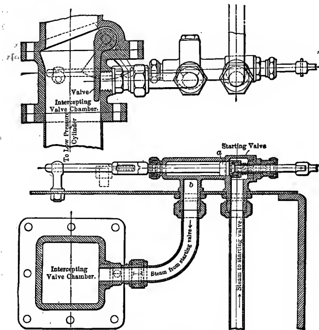
FIG. 152.—Plan and Section, Worsdell's Valve.
