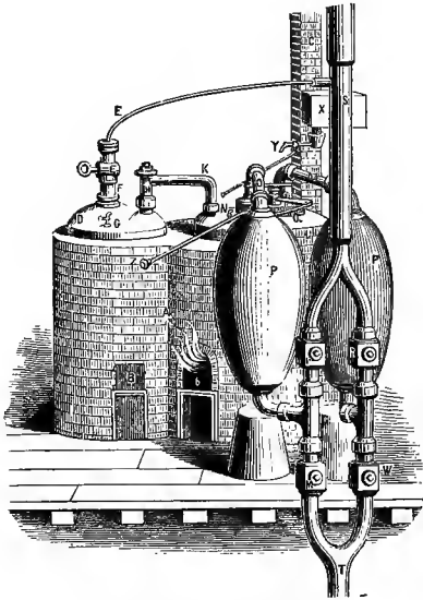
FIG. 13.—Savery's Engine, A. D. 1702.
