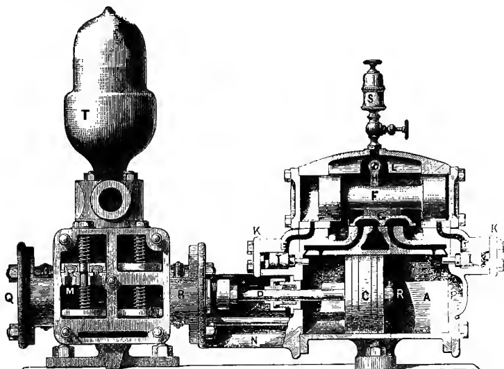
FIG. 102.—Steam-Pump.
