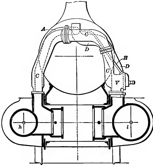
FIG. 148.—Compound Locomotive Engine.
