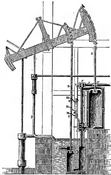
FIG. 26.—Watt's Engine, 1774.
