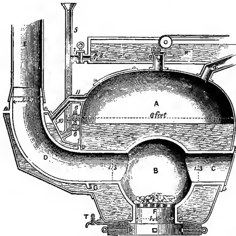
FIG. 23.—Smsaton's Portable-Engine Boiler, 1765.
