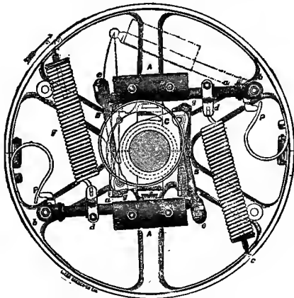
FIG. 160.—Shaft-Governor.
