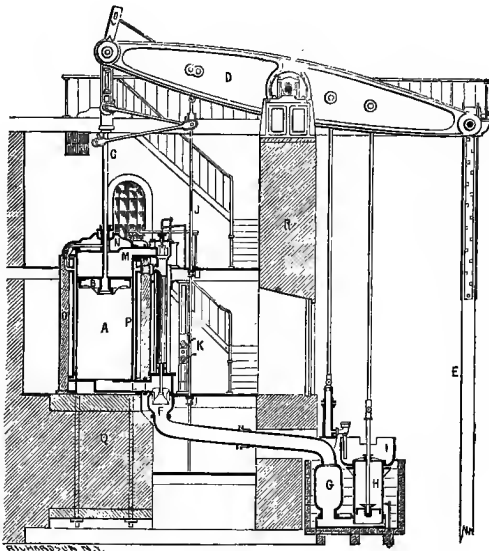
FIG. 101.—Cornish Pumping-Engine, 1880.
