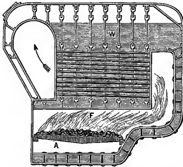
FIG. 142.—Marine Fire-tubular Boiler. Section.
