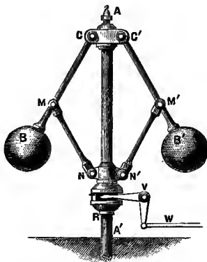
FIG. 29.—The Governor.
