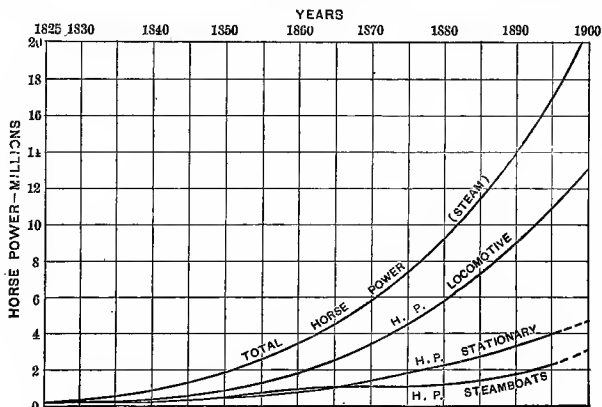
FIG. 169.—Available Steam-Power in United States.
