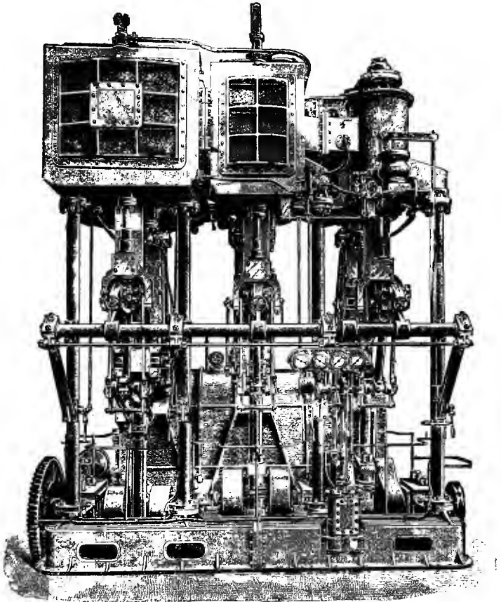
FIG. 156.—Triple-expansion Engine.
