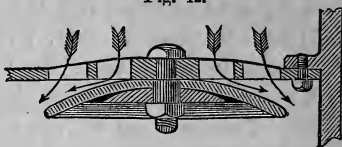
PENN'S DISC VALVE FOR AIR PUMP. Section.
