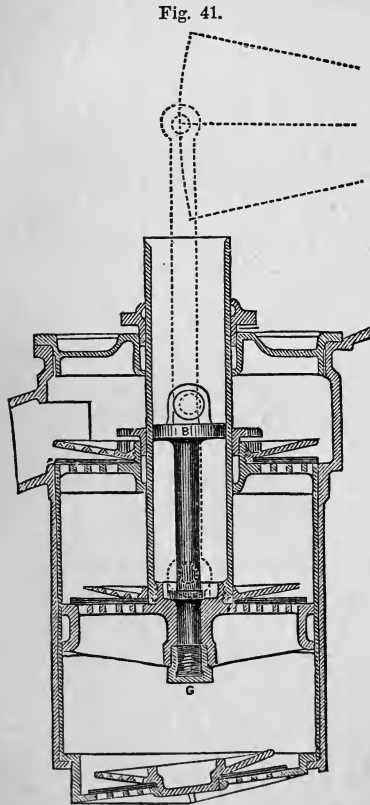
TRUNK AIR PUMP. Scale \frac{1}{4} inch to 1 foot.
