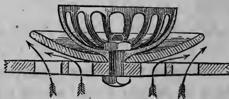
MAUDSLAY'S DISC VALVE FOR AIR PUMP. Section.
