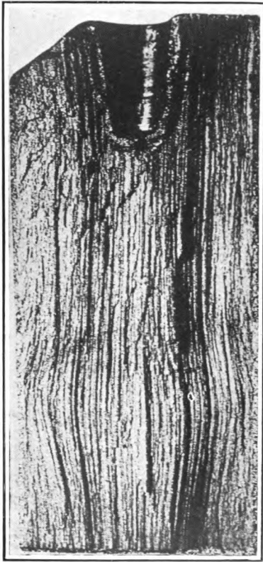
FIG. 32.—Fibrous fracture along length of case-hardened die.
