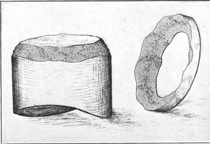
FIG. 83.—Effect of hardening stresses on sharp corners.
