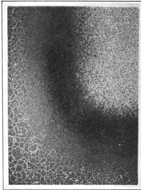
FIG. 80.—Crystal outlines about corner in quenched bar.
