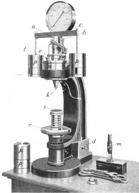
FIG. 62.—Brinell hardness-testing machine.
