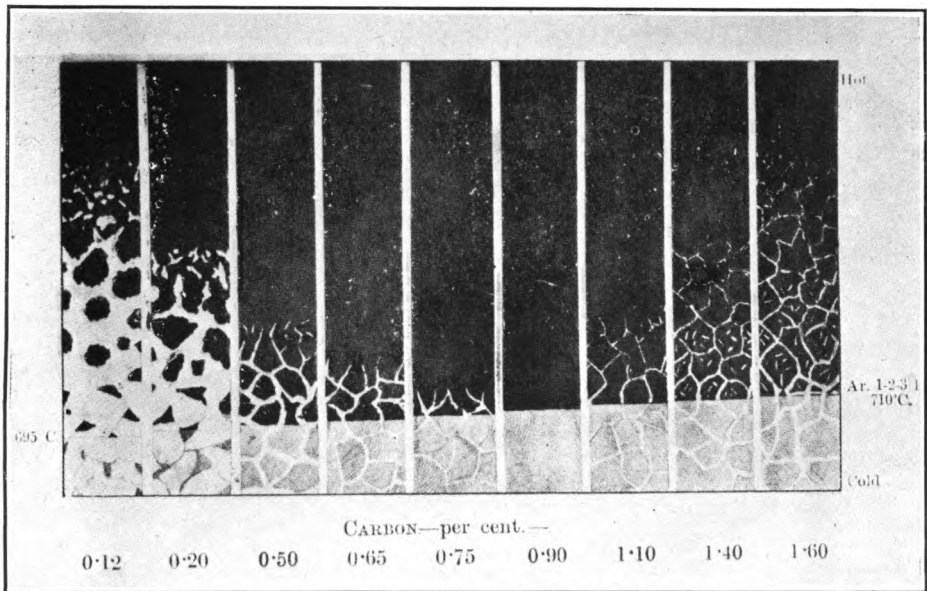
FIG. 55.—Mr. Stead's pictorial diagram.
