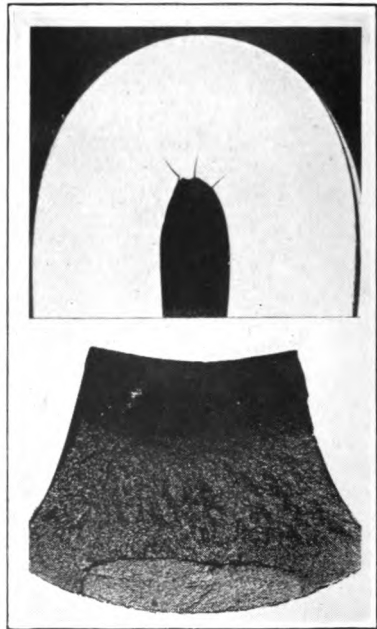
FIG. 86.—Cracks and fracture due to compression.
