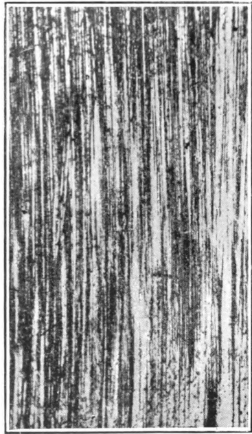
FIG. 37.—Streaky troostite due to grinding. x 25.
