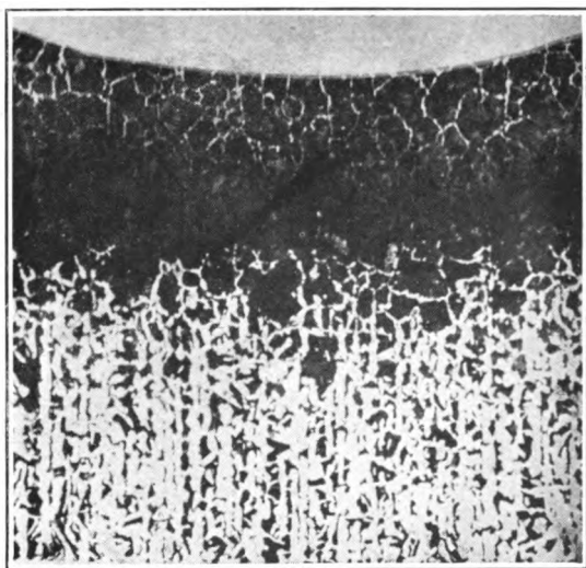
FIG. 48.—Degree and depth of carburisation as seen on polished and etched section. x 25.
