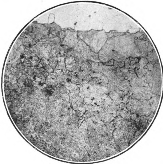
FIG. 44.—Quenched bar with sharply defined carbonless envelope. \times 100 .
