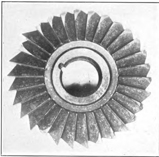
FIG. 84.—Splintered teeth of milling cutter caused by hardening.
