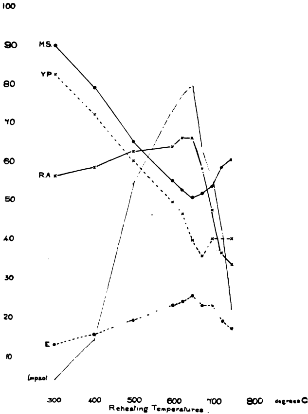
FIG. 74.—Mechanical properties of nickel-chrome steel after different forms of heat treatment.
