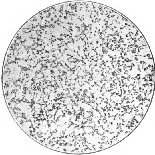
FIG. 18A.—Mild steel quenched from 800° C. after previous quenching from 920° C. x 200.
