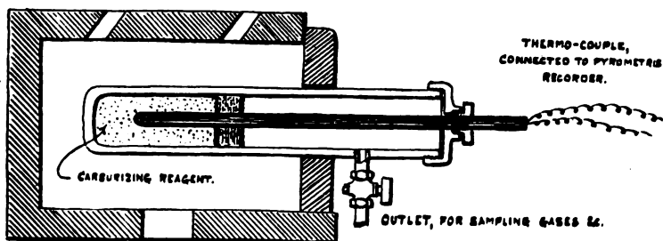
FIG. 57.—Arrangement for testing carburisers.
