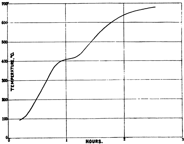
FIG. 58.—Heating curve of greasy bone black.
