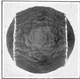
FIG. 88.—Disc of mild steel distorted by repeated quenching.
