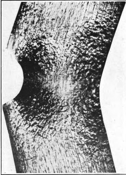
FIG. 66.—Distortion in impact test piece.
