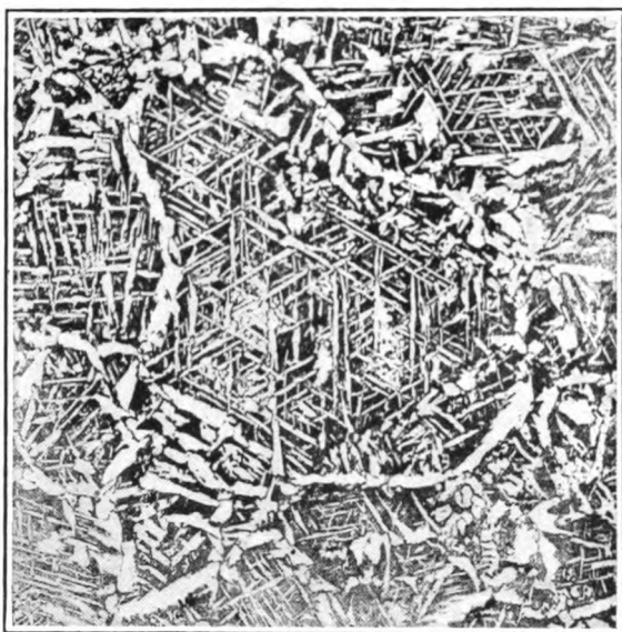
FIG. 5.—Peg quenched at 750° C. on heating. x 25.
