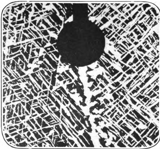
FIG. 65.—Irregular impact figures are obtained from coarsely crystalline material according as the bottom of the notch falls on or on either side of a crystal junction.
