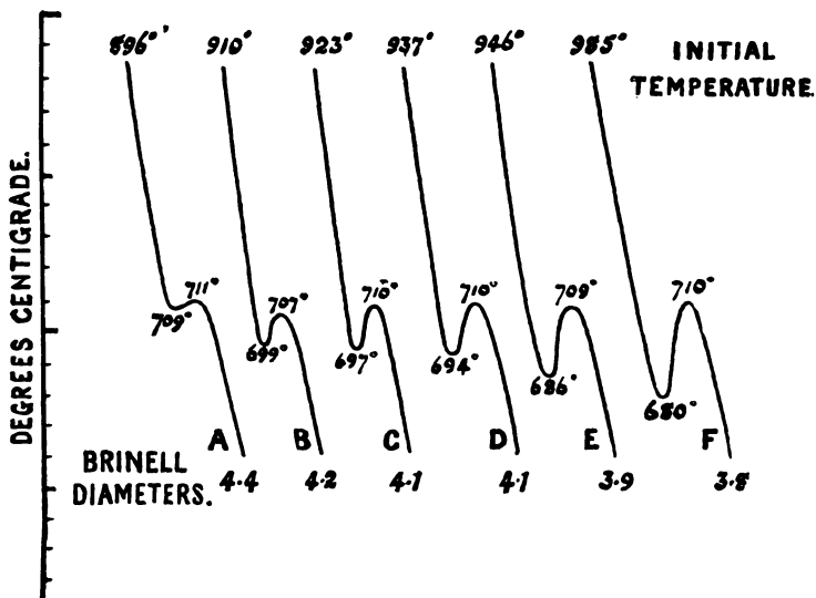
FIG. 76.—Effects of initial cooling temperature on chromium steel.
