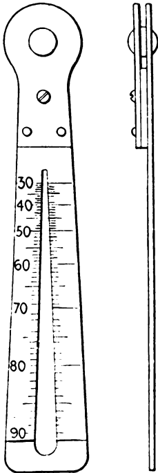
FIG. 63.—Ball holder for simplified form of Brinell test.
