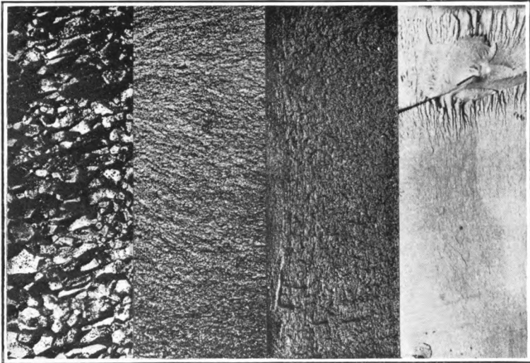
A B C D FIG. 72.—Different fractures from the same steel.
