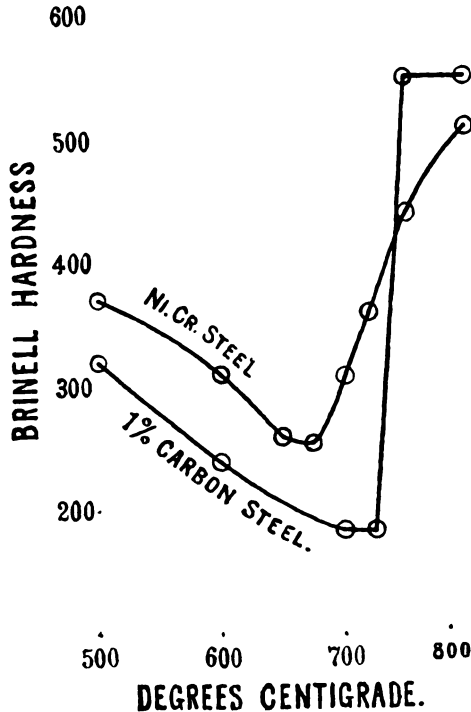
FIG. 75.—Comparative behaviour on tempering of carbon steel and nickel-chrome steel.
