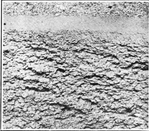
FIG. 27.—Coarse crystalline appearance of fracture due to free cementite.
