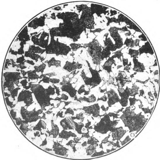
FIG. 14.—Peg quenched at 740° C. on cooling. x 100.
