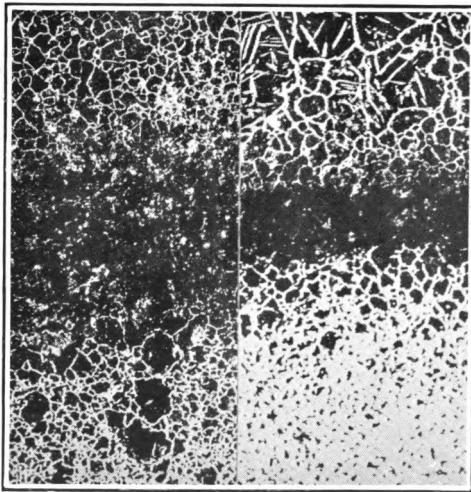
FIG. 3IB. FIG. 3IA. FIG. 3IA.—Bar cemented at 1,050° C. for eight hours. x 25. FIG. 3IB.—Same bar as 3IA reheated twelve hours at 1,000° C. x 25.
