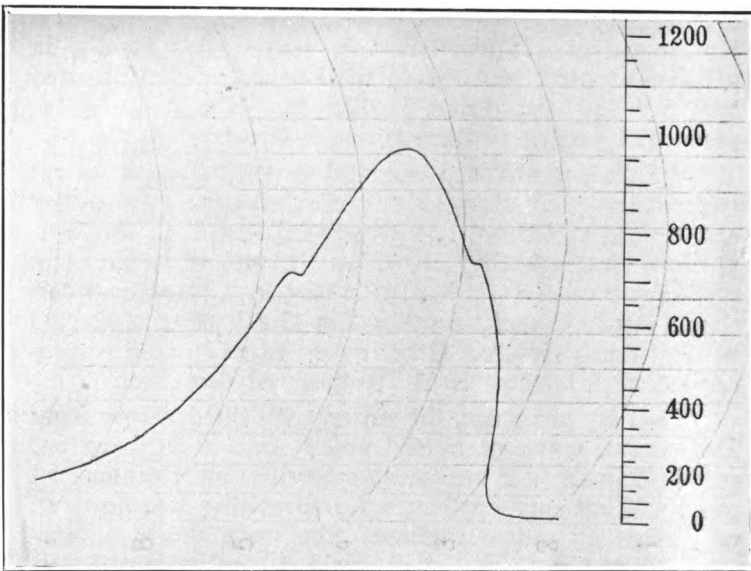
FIG. 89.—Heating and cooling curve made on works recorder.
