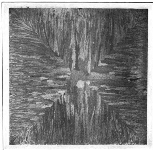
FIG. 79.—Polished and etched section of chrome steel ingot.
