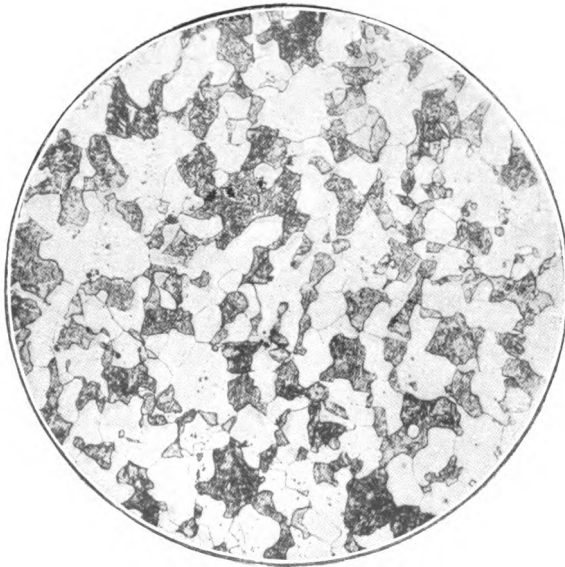
FIG. 18B.—Mild steel quenched from 800° C. after cooling slowly and reheating. x 100.
