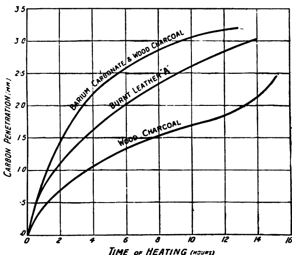
FIG. 59.—Time-penetration curves.
