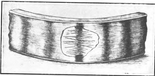
FIG. 39.—Soft splinter on hardened ring.
