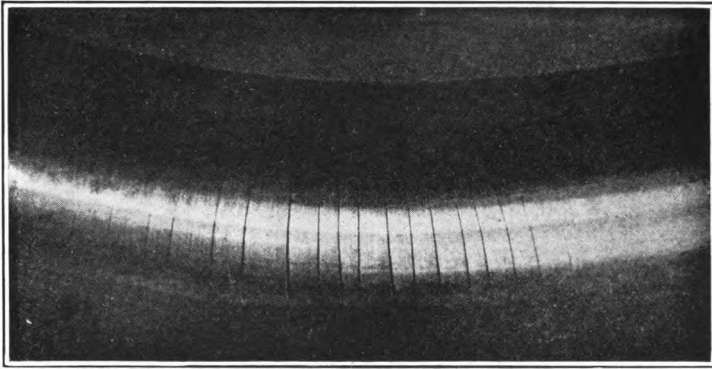
FIG. 70.—Ring cracks on bent case-hardened bar.
