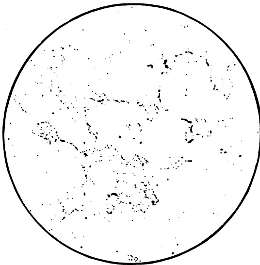
FIG. 46.—Cementite envelopes in slowly-cooled mild steel. \times 100 .
