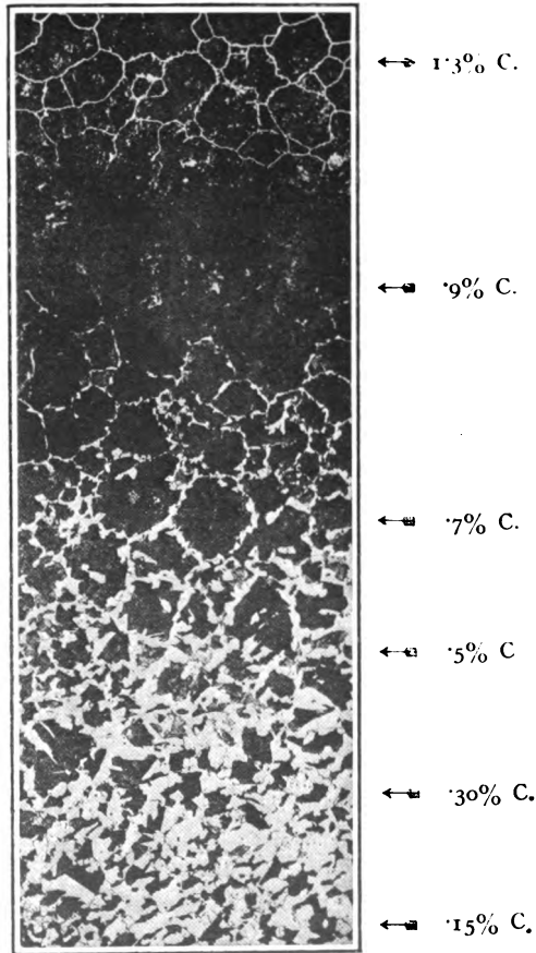
FIG. 1.—Section through cemented part of case-hardened bar.
