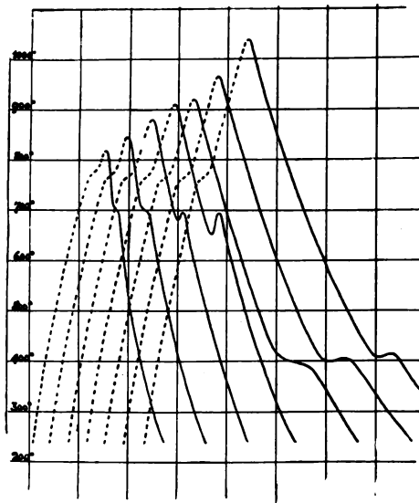
FIG. 77.—Effects of initial cooling temperatures on nickel-chrome steel.
