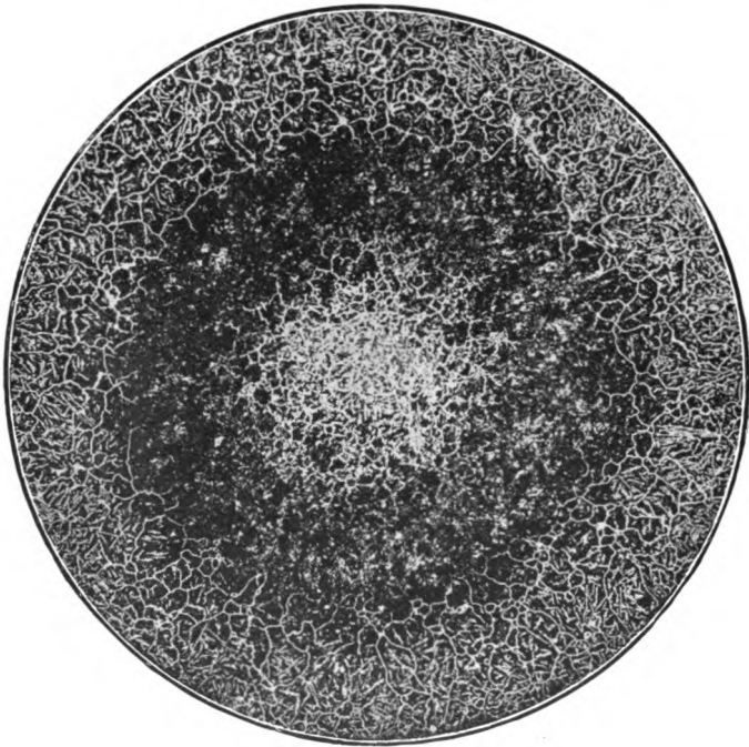
FIG. 49.—Entire cross section of case-hardened bar.
