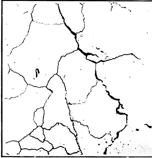
FIG. 29.—Crack proceeding along cementite outlines. \times 100 .
