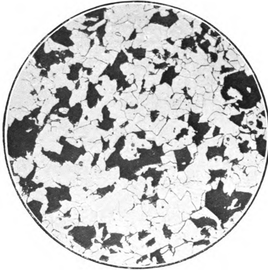
FIG. 16.—Any peg withdrawn below 670° C. on cooling. x 100.
