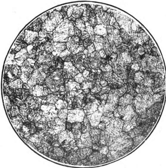
FIG. 10.—Peg quenched at 850° C. on heating. \times 100 .
