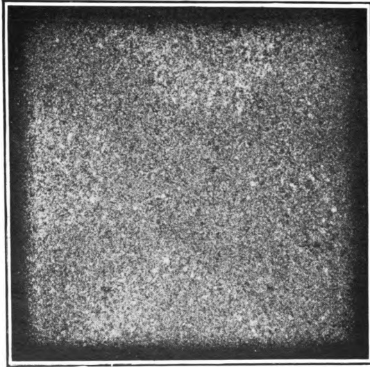
FIG. 71.—Section of cemented impact bar.
