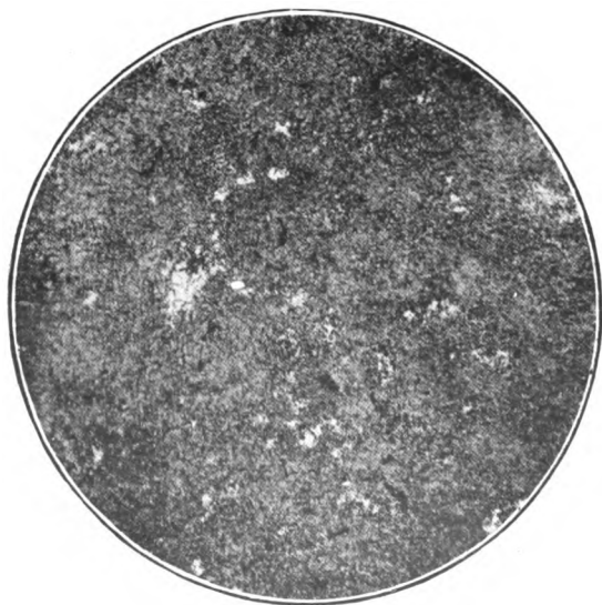
FIG. 9.—Peg quenched at 800° C. on heating. x 25.
