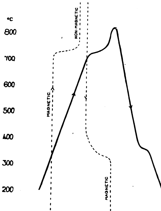
FIG. 78.—Effect of rate of cooling on thermal and magnetic changes.
