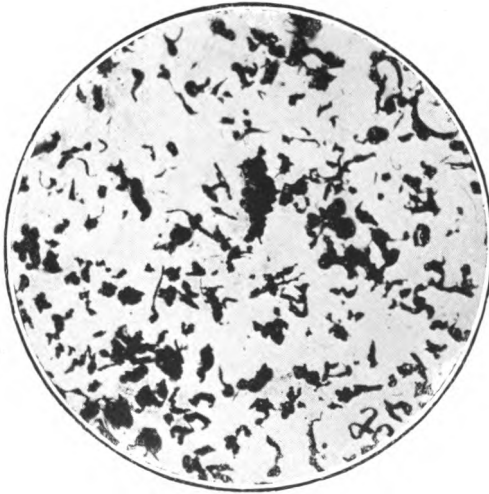
FIG. 36.—Grinding sparks caught on glass plate. \times 20 .
