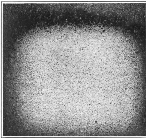
FIG. 43.—Section of bar in contact on one face only with case-hardening powder. x 5.
