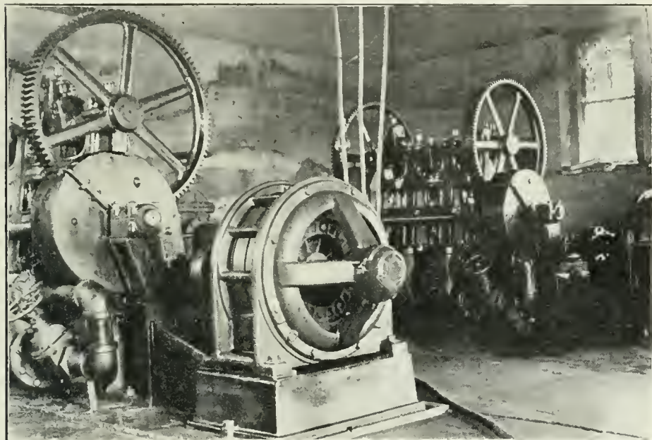
INTERIOR of Marseline, Mo., Water Works, showing producer-gas engine connected to generator.
