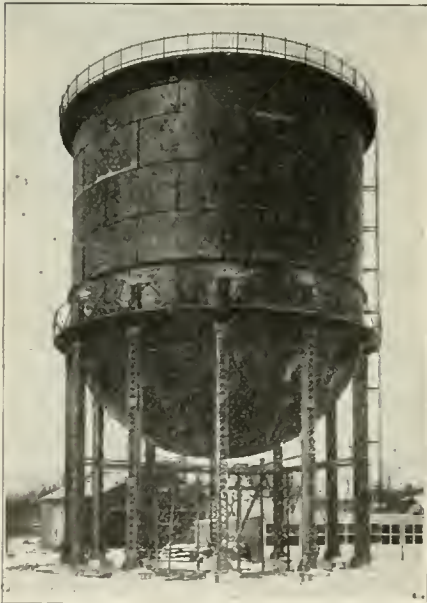
COMPLETED 560,000-gallon Lakeview water tank.
