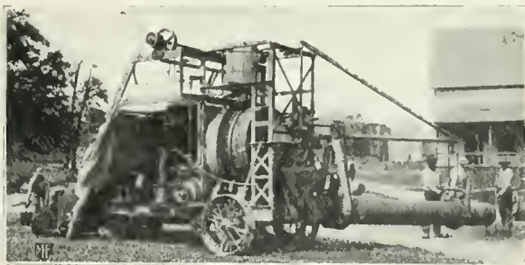
MIXING and placing mortar coat as wearing surface of Westrumite pavement. Chicago mixer in foreground.
