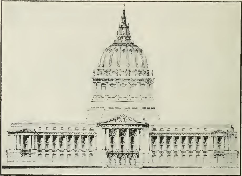
P OLK STREET elevation of San Francisco's new City Hall.
