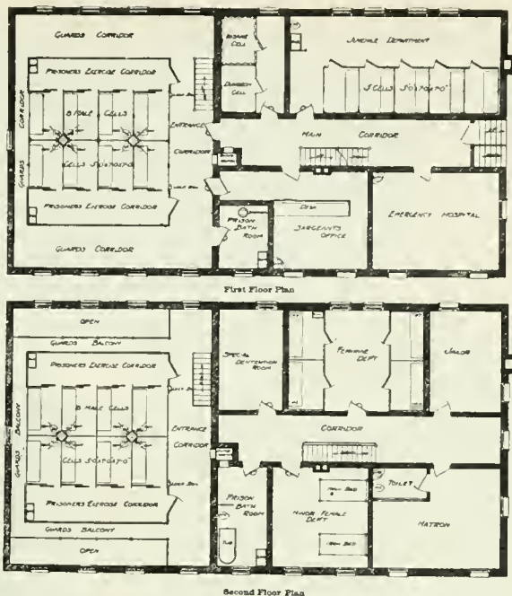
PLANS of first and second floors, City Jail, Salt Lake City, Utah.
