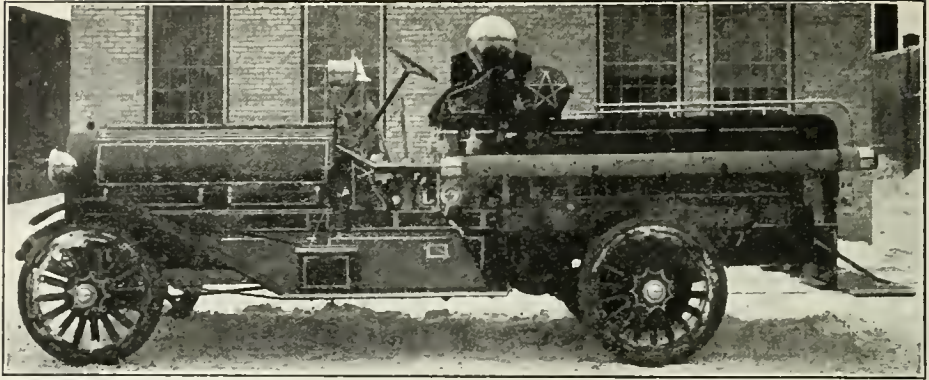
N OTT six-cylinder fire engine and hose wagon with a pump capacity of 900 gallons per minute against 150 pounds pump pressure.
