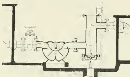
VIOLET-RAY apparatus attached to supply pipe, with agitator, to sterilize small public water supply.
