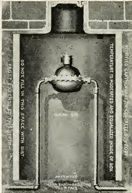
SECTIONAL view showing setting of Clark meter box and how freezing is prevented.
