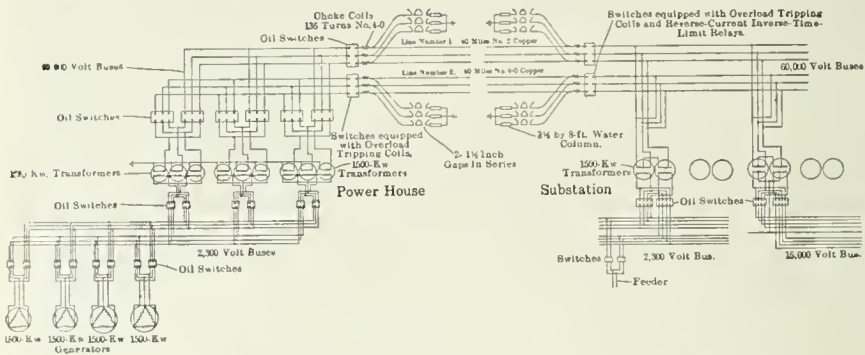
DIAGRAM of connections on special control board.
