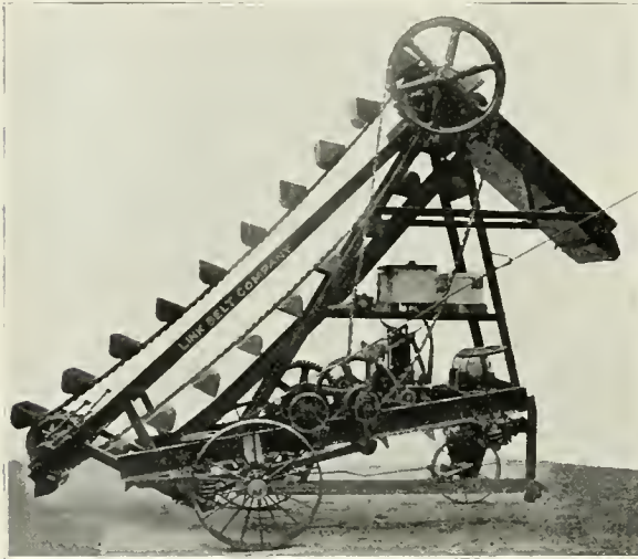
4. EQUIPPED with bevel drive and steering gear for self-propulsion over short distances.
