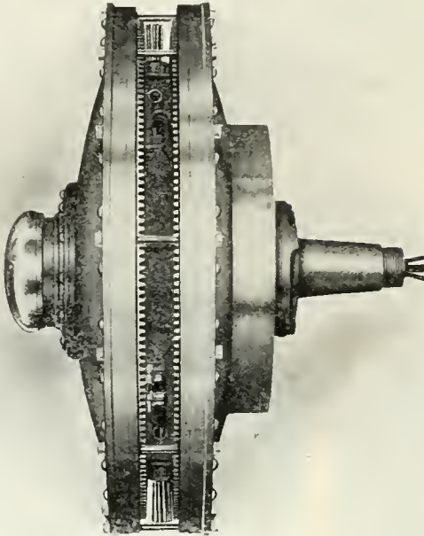
TIRE and band removed from Couple-Gear motor, showing relative position of the two pinions.
