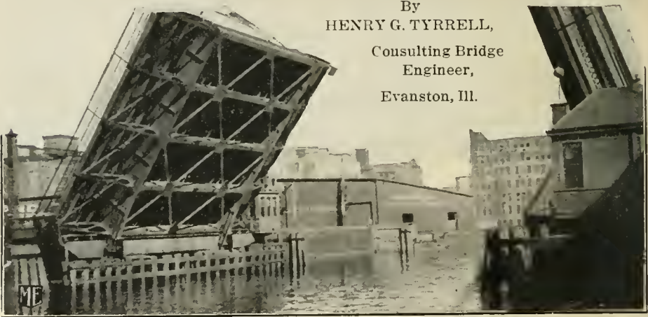
BEST TYPE OF LIFT BRIDGE in Milwaukee. A plate girder lift.
