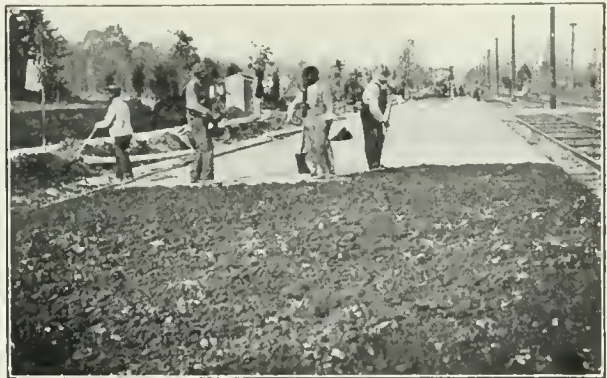
C OVERING Chevy Chase sample concrete road with earth to season. This earth covering was left on all winter and the bituminous surface was put on in the spring.
