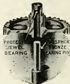
BEARING and pin construction of a Niagara meter.
