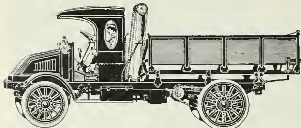
NEW KELLY power dumping truck showing position of dumping mechanism prior to lifting of the body.
