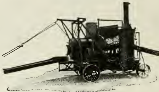
NEW TYPE of Standard Traction Paving Mixer.
