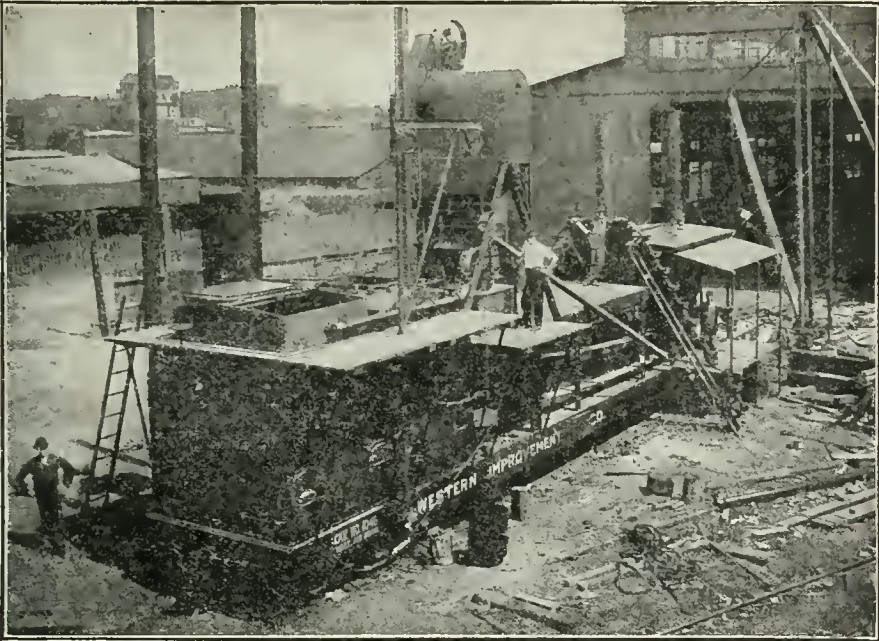
1,000 SQUARE YARDS 2-INCH TOPPING PER DAY.
