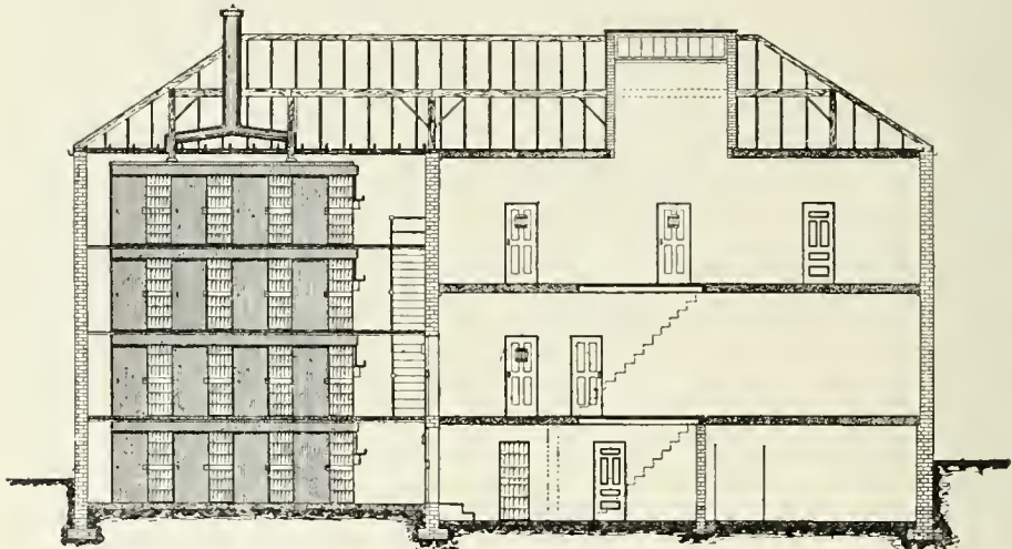
LONGITUDINAL Section of City Jail, Salt Lake City, Utah.
