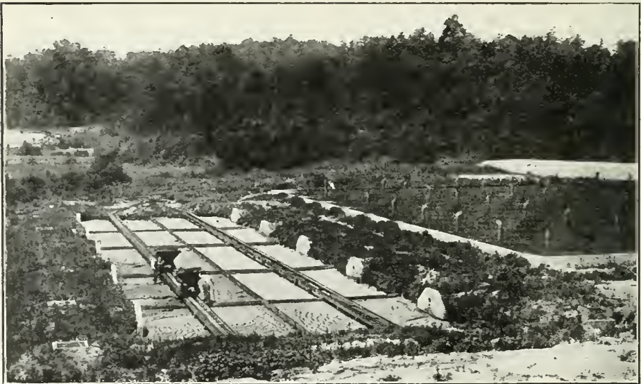
IV. SLUDGE BED. The semi-liquid sludge is run by gravity from the Imhoff tanks thru the pipes whose ends are seen in the small concrete end walls, of which there are five on each side of the bed. Each discharge from one of these pipes is enough to fill one of the divisions of the bed 7 to 10 inches deep. After drying the sludge is shoveled into the little cars running on the railways over the bed.
