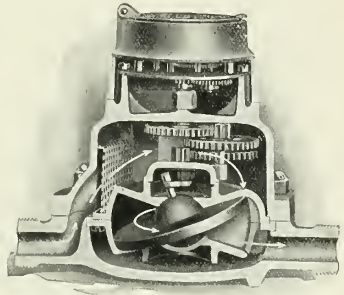
SECTIONAL view of meter in general use by Cincinnati Water Works.
