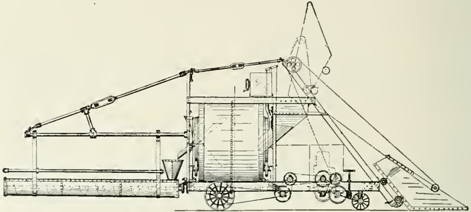
PLAN of 40-cubic-yard paving mixer.
