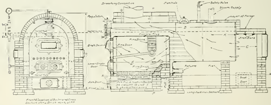
PLAN for setting Kewanee Smokeless Firebox Boiler.
