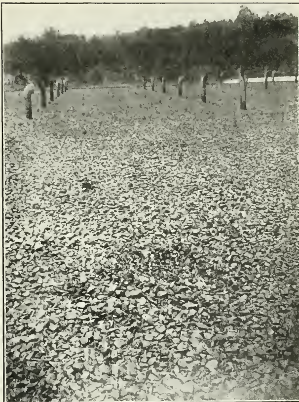
V. THE SURFACE of the contact filter bed filled with broken granite. The sprinkler heads which distribute the tank effluent over the surface of the filter are seen at the level of the surface of the bed. The ventilating pipes from the bottom of the bed, with their wind cowls, are the most prominent feature of the view.
