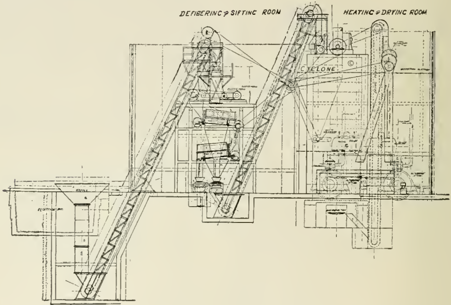
MIXED METHOD OF GARBAGE AND WASTE DISPOSAL. Sectional drawing of design for plant, showing garbage hopper at left, defibering machine at top of center, sifting machines below, heating and drying room, fertilizer plant, incinerating furnace and boilers at right, elevators, conveyors, blowers, etc.
