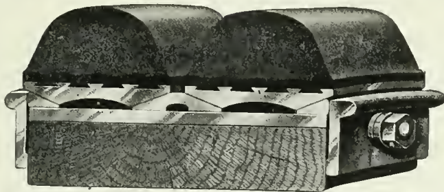
DUAL TREAD demountable cushion tire for fire apparatus.
