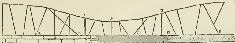
SECTION ILLUSTRATING THE FEEDING OF WATER BEDS IN ROCK THRU JOINTS IN ROCK LAYERS. Water bearing joints are indicated by the heavier lines. A, B, is water bearing area between limestone and a compact, jointed rock fed by joints at A and B. C is a water area between shale and compact jointed rocks, which has only a local circulation. D is a water area fed from a sandstone bed. E is the sandstone bed fed by joints. There is a flowing well at 1 fed from the bedding plane between limestone and compact jointed rocks, A B. The well driven at 2 was a dry hole, there being no circulation of water along the bedding plane at this point. There is a flowing well at 3 from the bedding plane D which is fed from the sandstone E.
