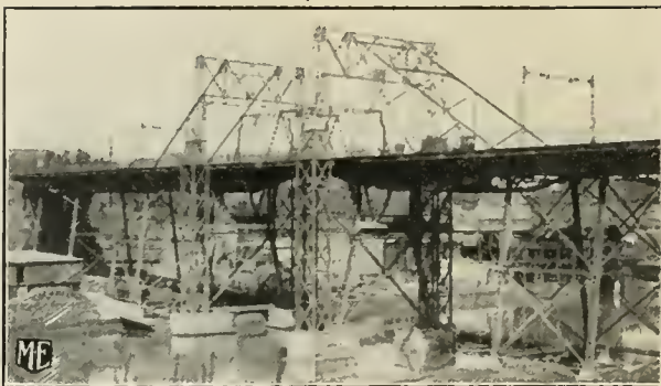
HOLTON STREET LIFT BRIDGE, Milwaukee, Wis.
