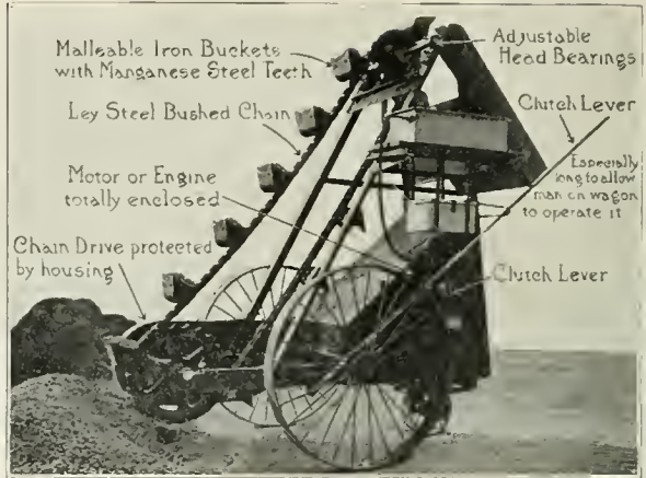
1. LINK-BELT portable loading machine for raising materials to wagons and cars.
