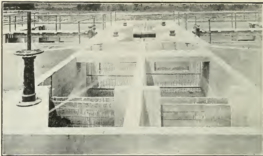
SPRINGFIELD, MO., sewage disposal plant. Completed grit chamber, with settling tanks on either side.
