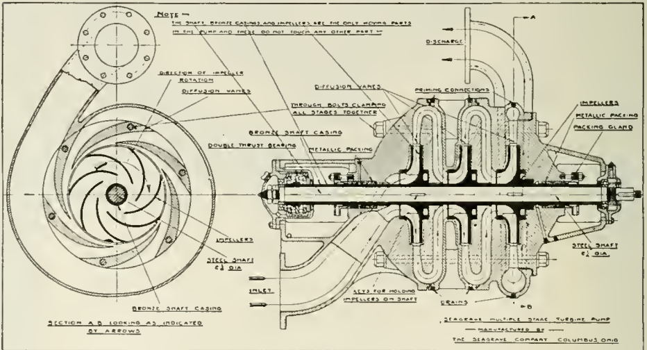
SECTIONAL VIEW OF SEAGRAVE Multiple Stage Pump.
