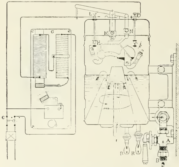
D IAGRAM of small violet-ray apparatus, showing machine attached to tap to purify domestic water supply.
