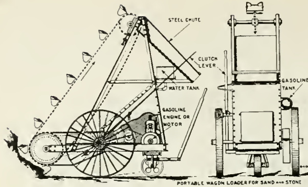
SECTION of link-belt portable excavator and loading machine.
