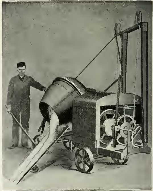
JAEGER MIXER used to distribute cement filler direct to pavement.
