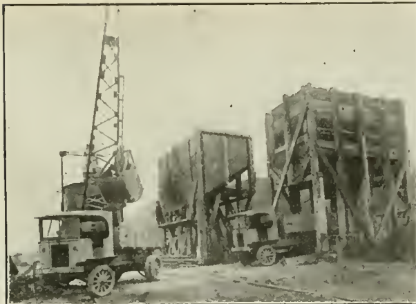
SPECIAL LOADING DEVICES FOR CONTRACTORS' TRUCKS. Garford trucks loading from hopper and from grab-bucket handled by crane.
