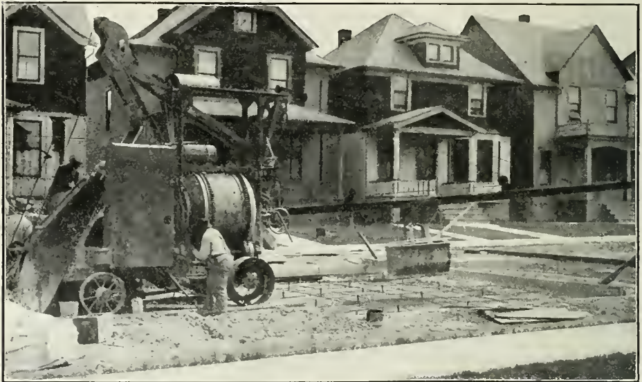
CONSTRUCTING REINFORCED CONCRETE PAVEMENT, Detroit, Mich. Note reinforcement in place, concrete mixer with boom and traveling bucket, placing first layer of concrete. Protection for joint in place at the right.
