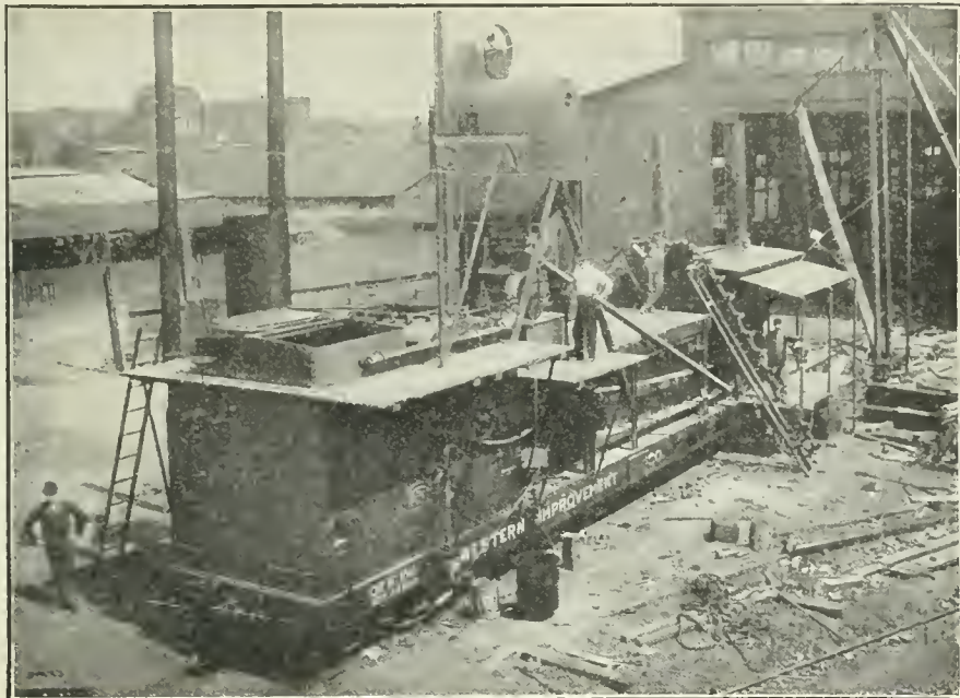
MODEL OF 1912 ONE-CAR PLANT.
