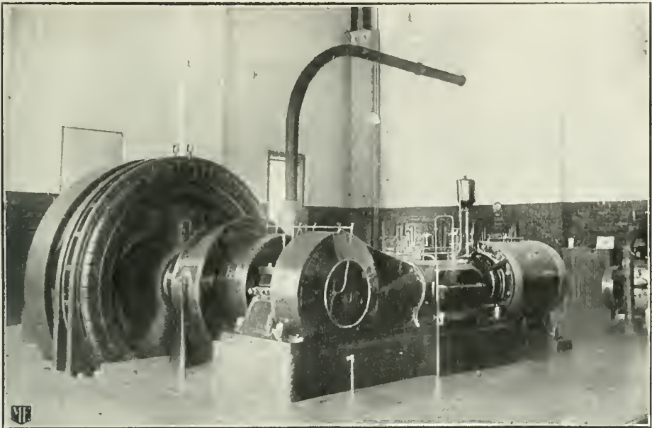
F ORT WAYNE electrical equipment as installed in the municipal electric light and water works plant at Fremont, Nebraska.
