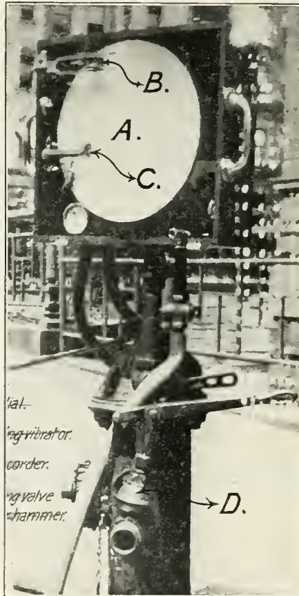
L OCATING LEAK in water main by Pulsograph, shown in place on hydrant. A—Recording dial. B—Time recording vibrator. C—Pressure recorder. D—Quick operating valve to create hammer.
