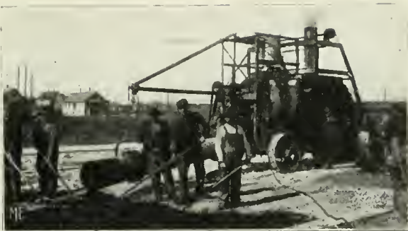
MIXING and depositing Westrumite pavement with Chicago concrete mixer.
