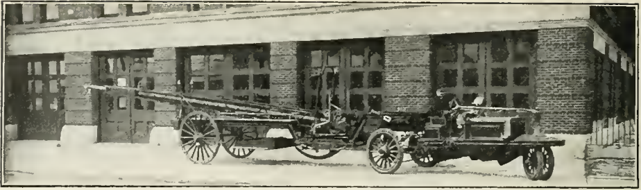
HORSE-DRAWN water tower converted to motor apparatus by connecting a Knox-Martin tractor.
