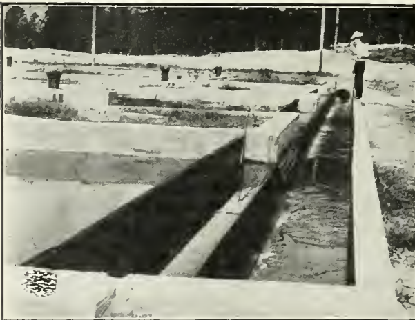
II. CHANNEL at rear of Imhoff tanks, serving to carry sewage to the tanks or by reversal, with stop planks to carry the effluent to the screen and head house, as here operating. The clear water in the settling tank is seen behind the scum board in the left foreground.
