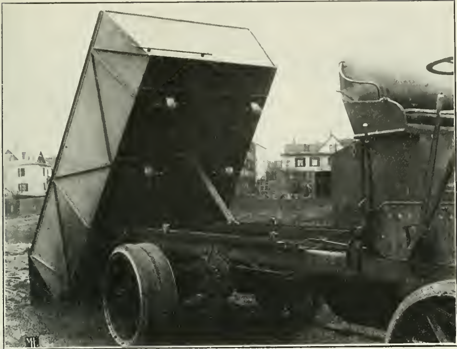
L OCOMOBILE steel demountable dump body, operated by power from the engine, showing rollers and rails.
