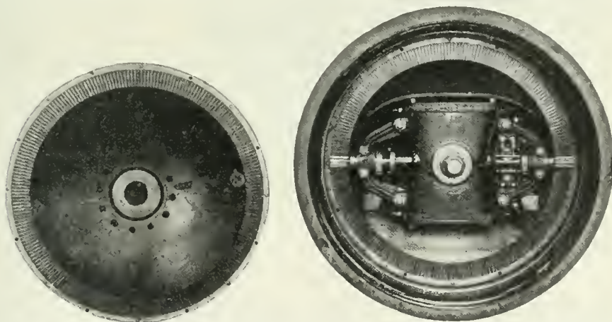
VIEW of Couple-Gear motor wheel showing front disk and, side of motor removed, giving access to the armature, field coils and bearings.
