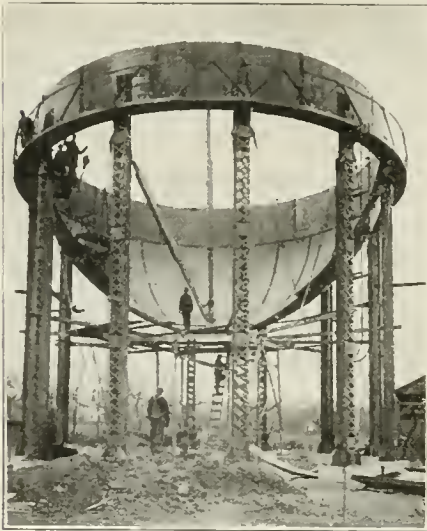
LAKEVIEW TOWER under construction.
