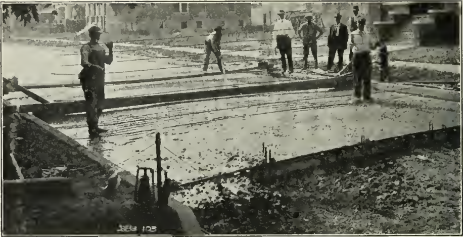
BUENA VISTA AVE., Highland Park, Mich. Construction of concrete pavement, showing pavement reinforcement being placed, and expansion joint which extends entire depth of pavement.
