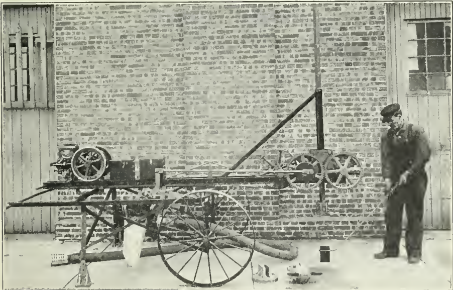
STALEY tamper with attachment for cutting holes in concrete walks.
