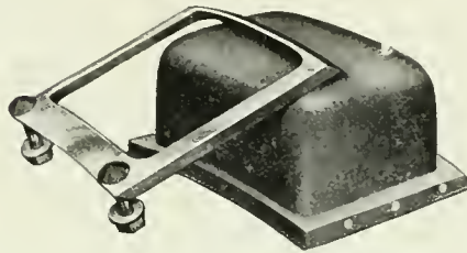
SECTION of block solid tire with frame for fastening to rim.
