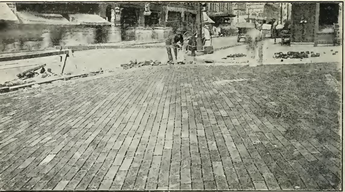
JACKSON AVENUE, Toledo, O., creosoted yellow pine wood lug block pavement under construction. Grade over 3 per cent.
