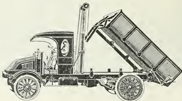
POSITION of dumping apparatus when truck body is completely elevated for dumping. Entire mechanism controlled from driver's seat.
