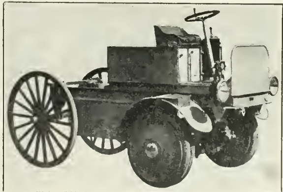
ELECTRIC TRACTOR used in Springfield, Mass., for motorizing apparatus which has heretofore been horse-drawn. Tractor manufactured by the Couple-Gear Freight Wheel Co., Grand Rapids, Mich.
