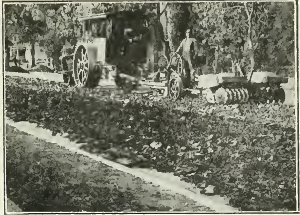
WEST ADAMS STREET, Los Angeles, Cal., pavement under construction. The city owns the outfit shown, which consists of a fifteen-ton Monarch roller, a petrolithic gang rooter, and a Hatch disc harrow.
