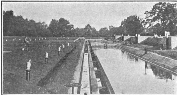
SETTLING BASINS FOR CONTACT EFFLUENT.
