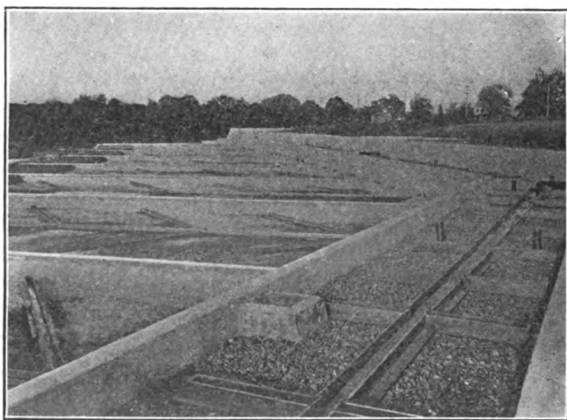
SECONDARY SAND BEDS.
