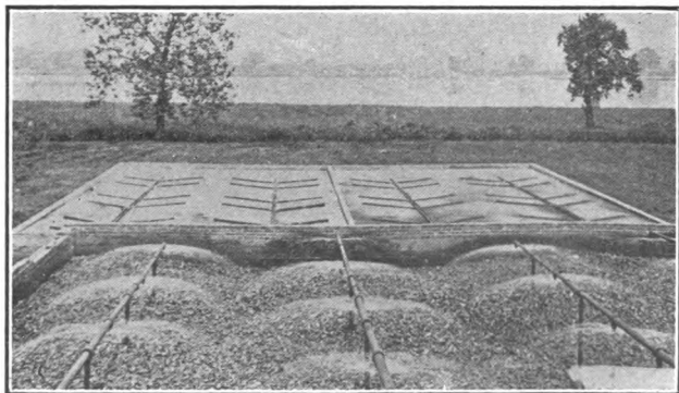
SPRINKLING FILTER WITH INVERTED NOZZLES.
