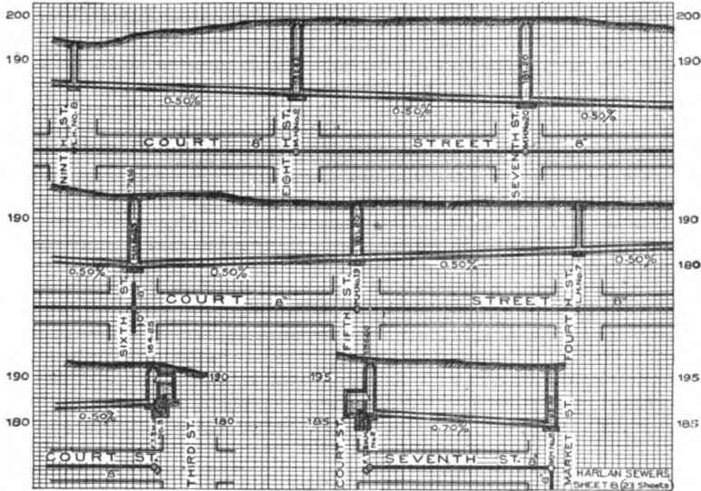
Fig. 39. Typical Sewer Profile Sheet.
