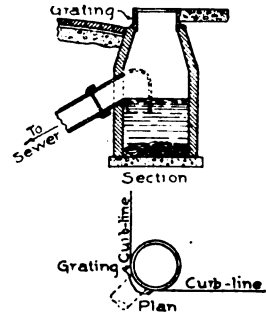
Fig. 14. Catch-Basin.
