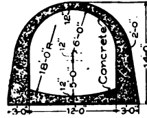
Fig. 23. Dry-Run Sewer, Waterloo, Iowa.
