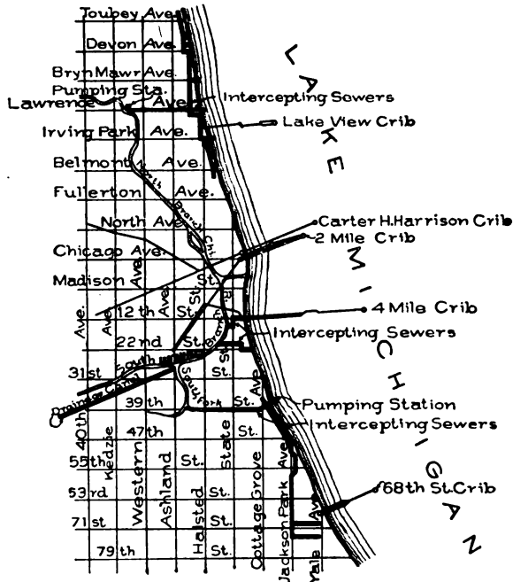
Fig. 5. Intercepting Sewers of the City of Chicago, Ill.
