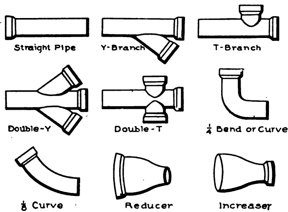
Fig. 16. Vitriified Sewer-Pipe and Specials.
