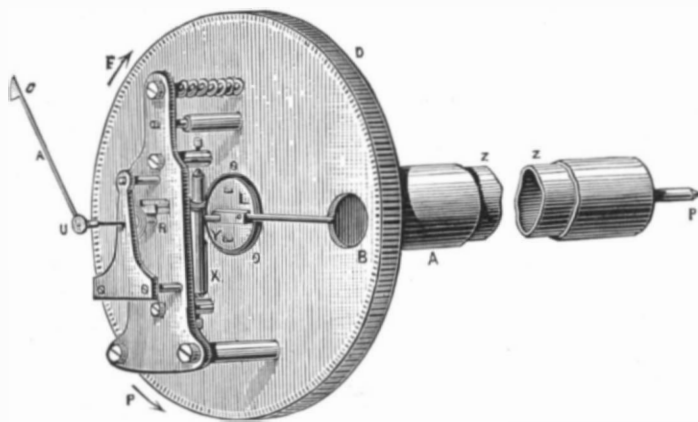
Fig. 1.—REGISTERING THERMOMETER.
