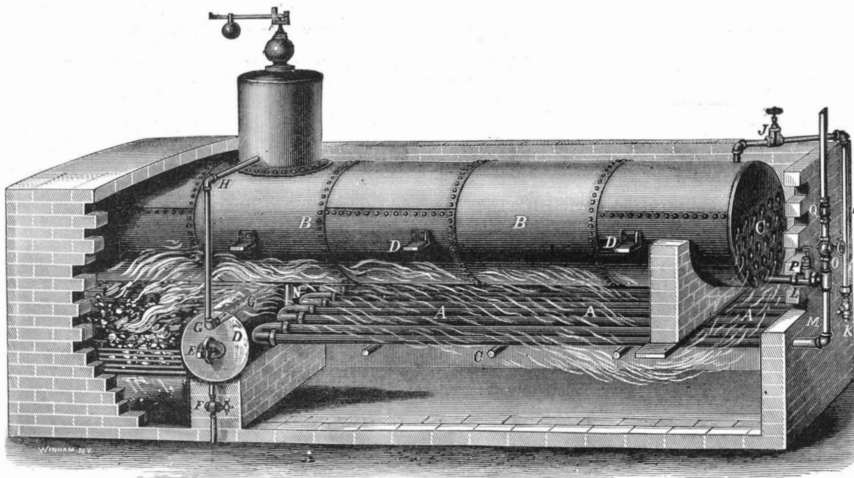
STEAD'S CIRCULATING GENERATOR FOR STEAM BOILERS.
