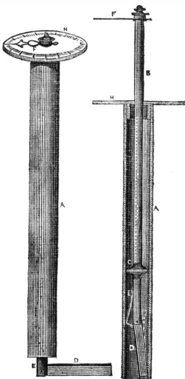
Wilders Leeway Indicator. FIG. 1. FIG. 2.
