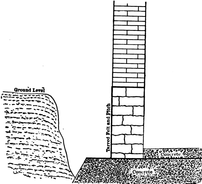
FIG. 1.—A Method of Constructing a Foundation.
