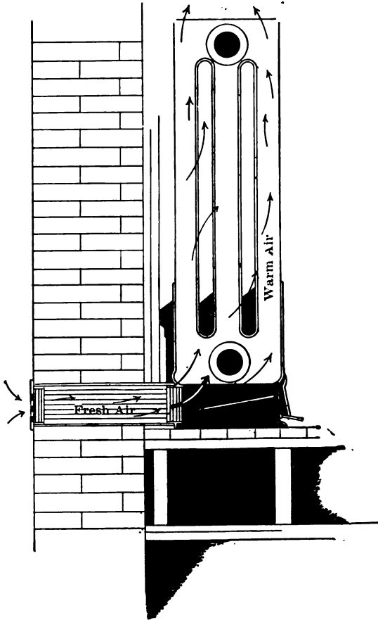
FIG. 6.—Heating by Direct-indirect Radiation.
