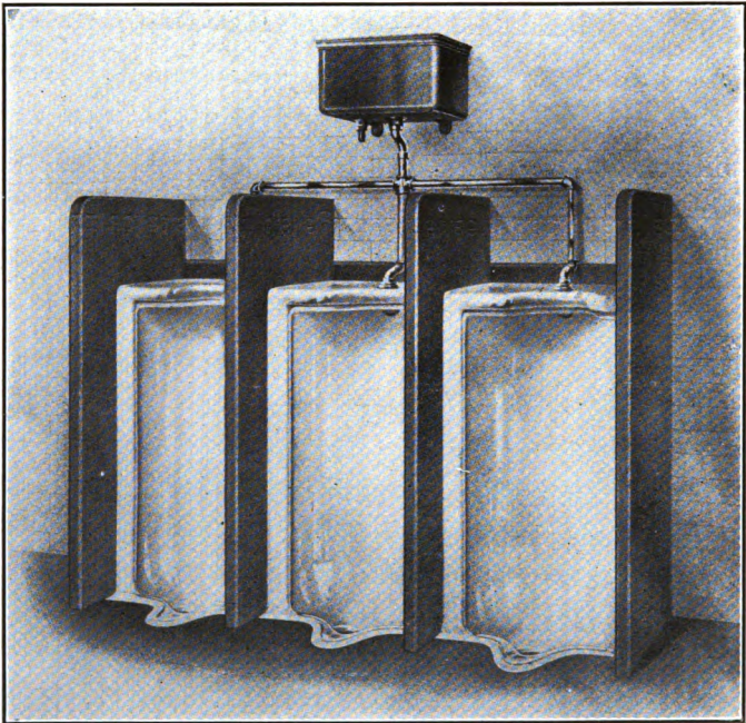
FIG. 9.—A Sanitary Urinal. (From a copyrighted photograph by the J. L. Mott Co.)
