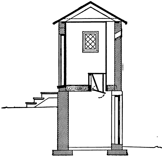
FIG. 28.—Dry Closet for Schools.
