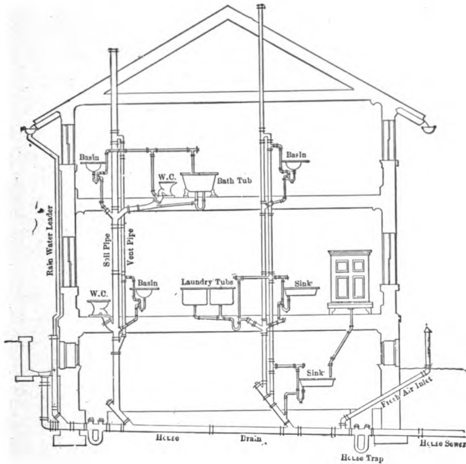
FIG. 2.—Section of a House, showing Plumbing System.
