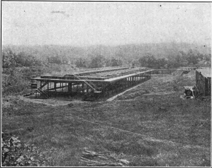
FIG. 19.—Sewage-filtration Plant, Reading.
