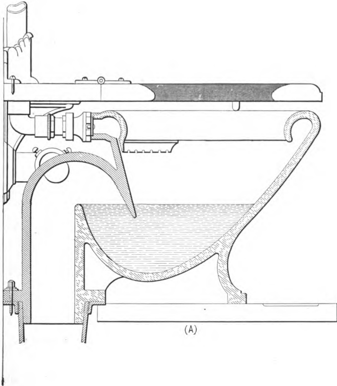
FIG. 5a.—Wash-down Closet.
