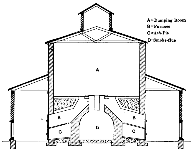
FIG. 20.—Section of Thackery Garbage-furnace.
