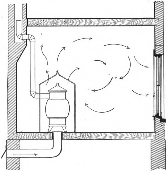
FIG. 26.—Diagram showing Circulation of Air in a Room heated by a Ventilating-stove.
