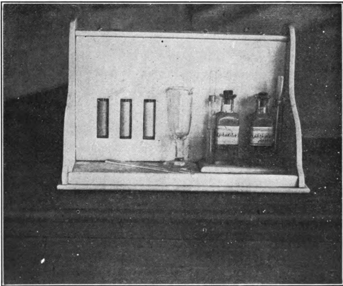
FIG. 16.—Apparatus for Water Analysis. (Photograph by the Author.)
