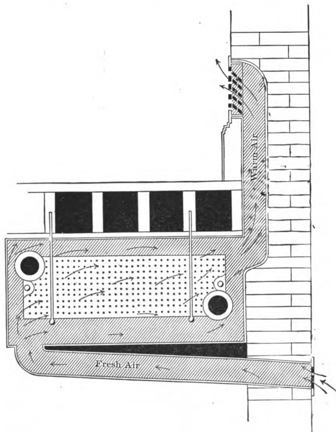
FIG. 7.—Heating by Indirect Radiation.
