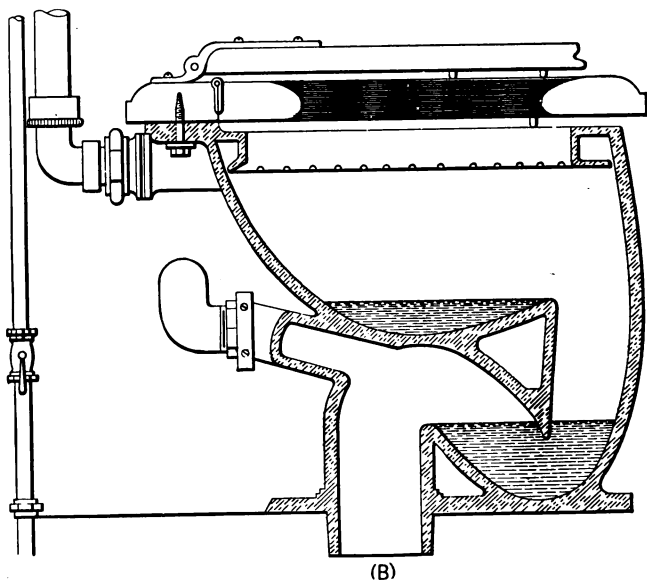
FIG. 5 b .—Wash-out Closet.
