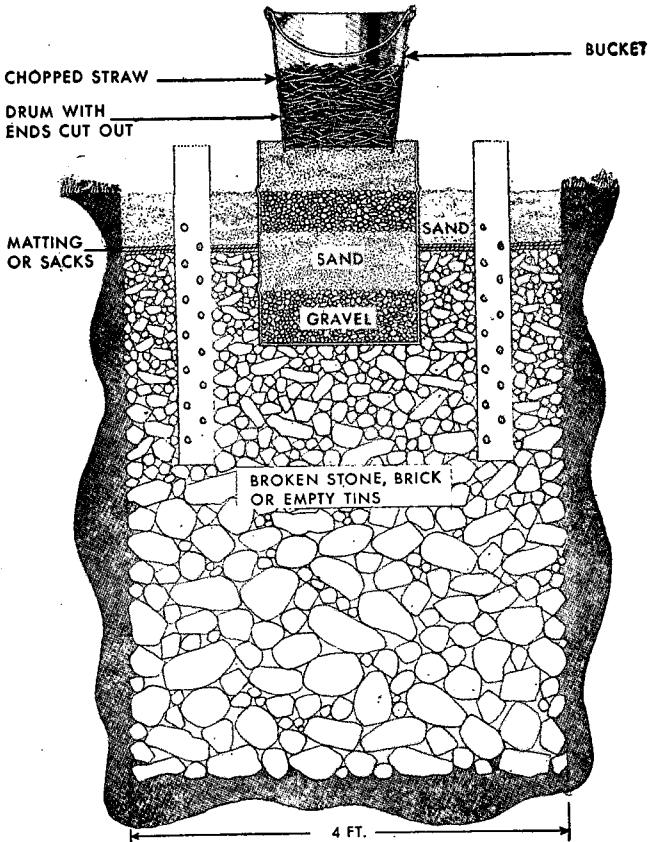
Figure 25. Kitchen soakage pits and baffle grease trap.
