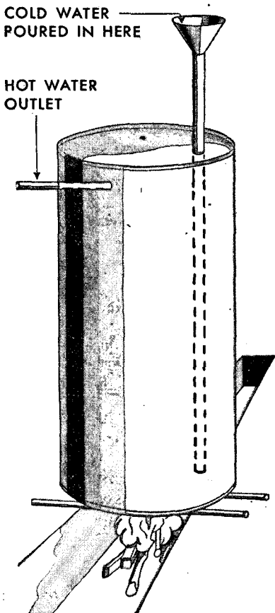
Figure 55. Heating shower water.
