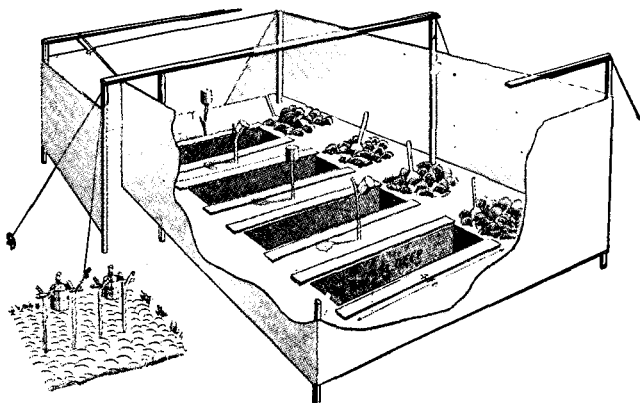
Figure 9. Hand-washing device.
