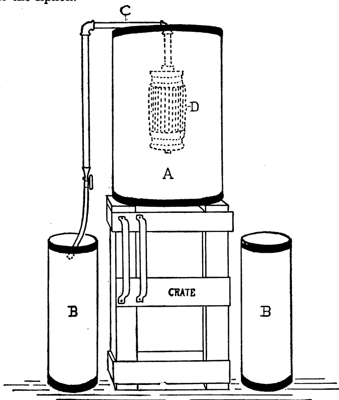
Fig. 17.—Darnall filter, showing method of operation.
