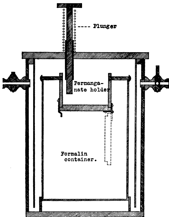
Fig. 32.—Gas generator, for disinfection in the field. Height, 8 inches; diameter, 6 inches; weight, 5 pounds (Munson).
