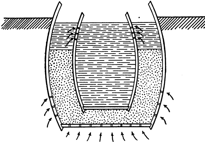
Fig. 18.—Barrel filter sunk in spring.
