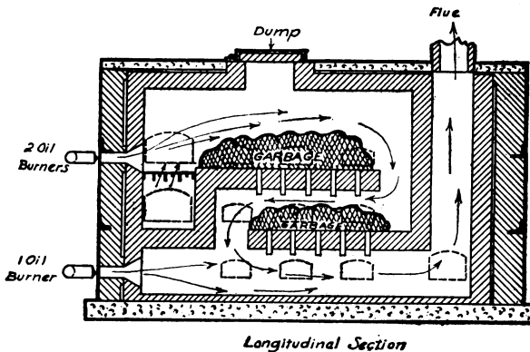
Fig. 37.—Morse-Boulger destructor, longitudinal section.
