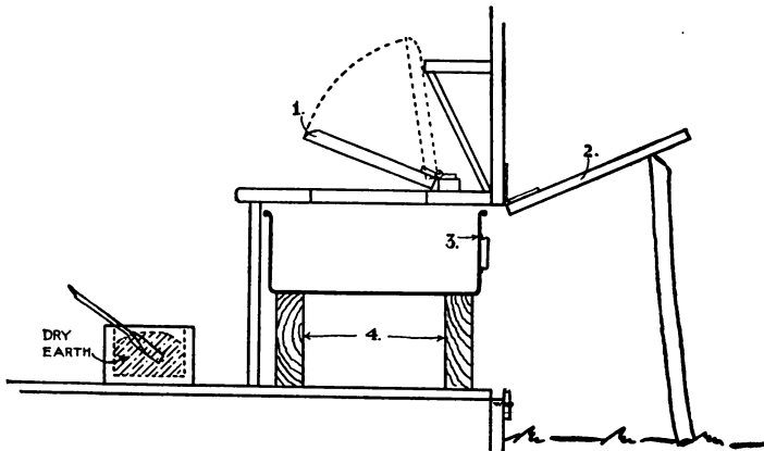
Fig. 34.—Dry earth closet: 1, Self-closing seat cover; 2, fly-tight trap-door; 3, pan; 4, supports for pan.
