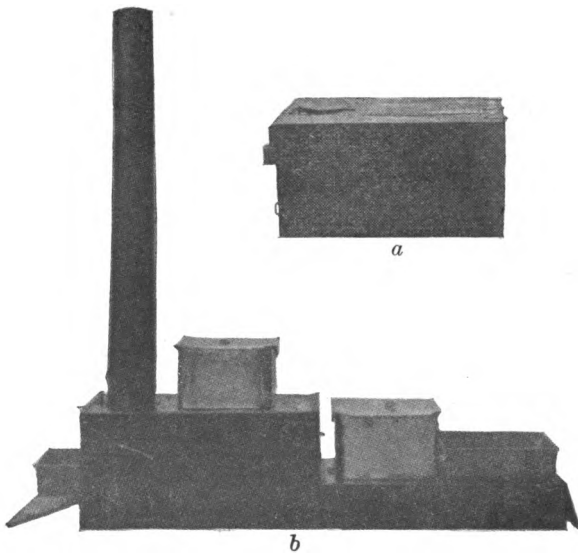
Fig. 20.—United States Army field range: a , Packed for transportation; b , set up ready for use.
