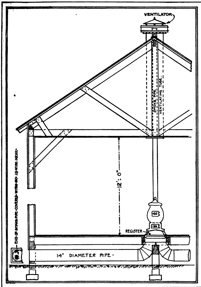
Fig. 24.—Ventilation system for temporary buildings by means of fresh-air ducts beneath floors, opening under stoves.
