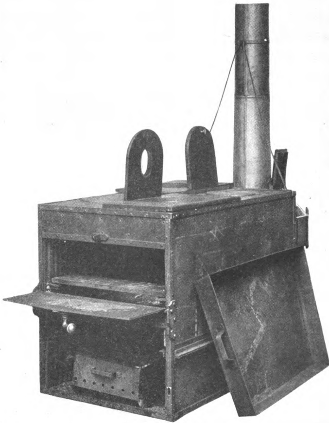
Fig. 40.—Incinerator for excreta, Quartermaster Corps type.
