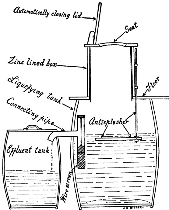
Fig. 35.—Closet devised by officers of the United States Public Health Service (Lumsden, Roberts, and Stiles).
