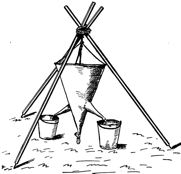
Fig. 16.—Ishiji filter (Japanese model).
