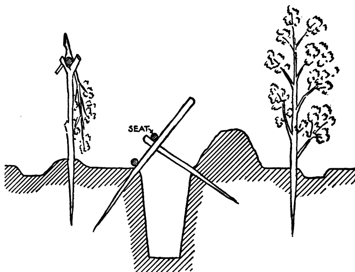
Fig. 43.—Company sink, cross-section, showing pole seat, brush screening, and ditching.
