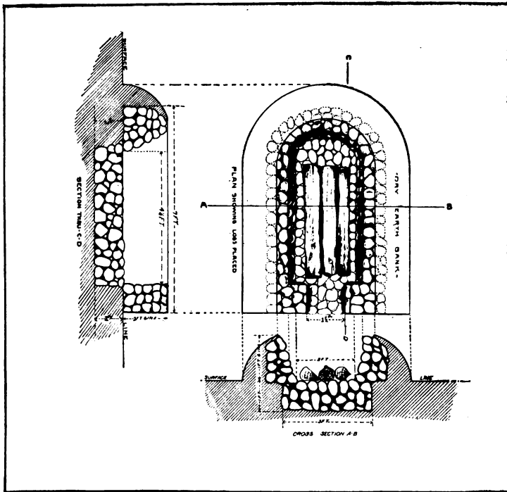
Fig. 45.—Company mess incinerator (Straub).
