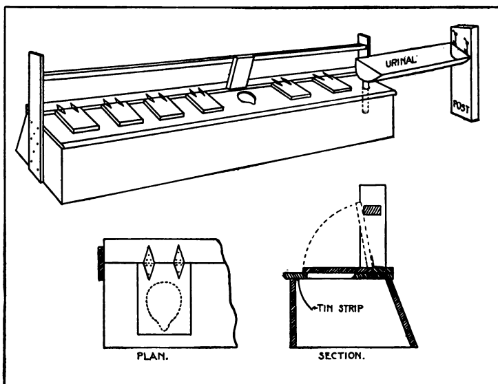
Fig. 42.—Box seat cover and urine trough for company sink. Note shape of seat, self-closing cover, slope of back, and tin strip. (After Straub and Miller.)
