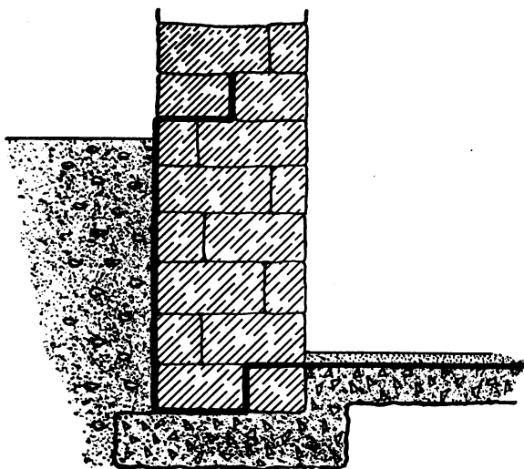
Fig. 22.—Damp-proof course for foundations of buildings (indicated by the heavy line).
