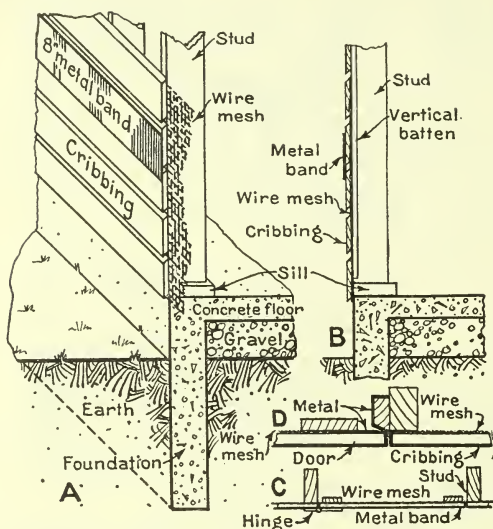
FIGURE 8.—Suggested construction for cornerrib: A, Section through wall; B, section through door, which is made of cribbing on vertical battens; the metal band on the wall extends across the door, but is cut and bent inward at the edges of the door; C, plan of door; D, enlarged detail of jamb at closing side of door
