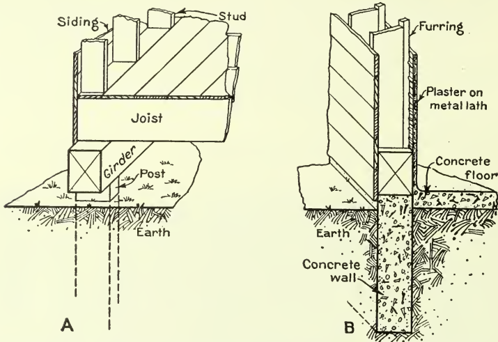
FIGURE 4.—A, Detail of old barn with floor supported a few inches above ground on girders and posts; B, same barn made rat proof with concrete foundation and floors and cement-plastered walls
