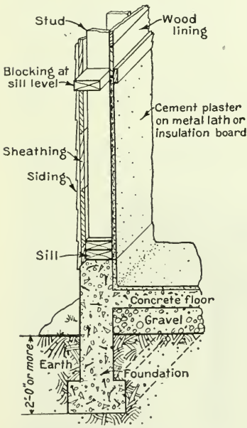
FIGURE 7.—Recommended construction of walls and floors of new frame barns. Cement plaster on metal lath or insulating board is applied to the inside of the studs at least to the level of the window sills as a better protection against rats and as being more easily kept clean than wooden lining
