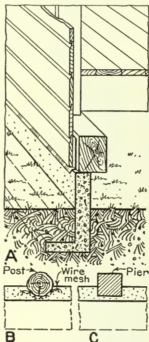
FIGURE 22.—A, Concrete curtain, or area wall, designed for rat-proofing purposes; it does not support the building. B, Plan of wall where supports are of wood; the concrete is bound to the posts with wire mesh. C, Plan of masonry support; concrete will adhere to the masonry if the surface is roughened
