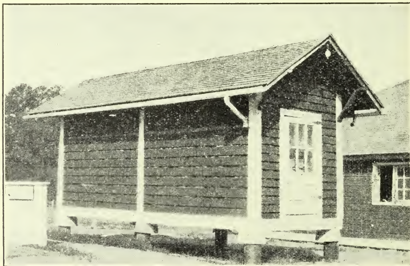
FIGURE 9.—An inexpensive method of rat proofing a cornerrib. It is supported by glazed tiles capped with galvanized washtubs, which, though not attractive in appearance, have successfully kept out rats
