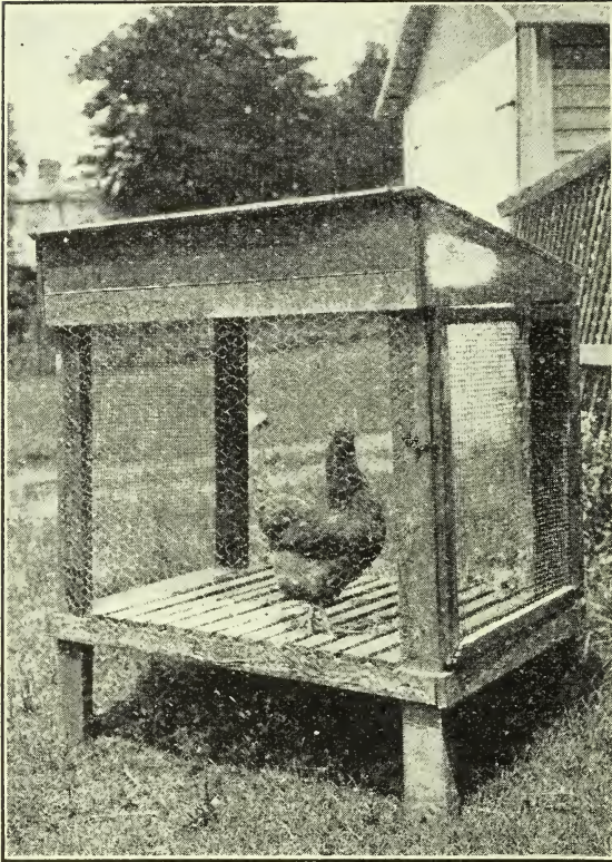
FIGURE 14.—Coop built up off the ground, rather than with the floor resting on the ground and thereby affording rats a desirable hiding place
