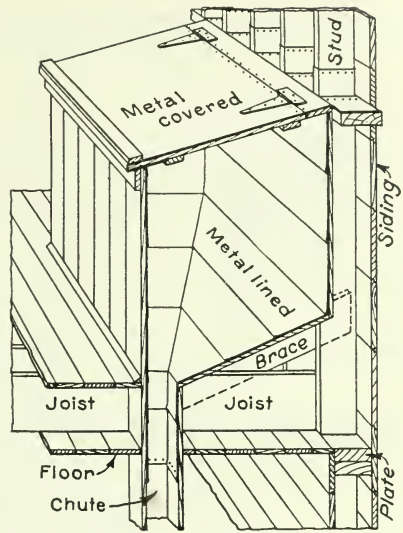
FIGURE 6.—A convenient upper-story rat-proof grain bin
