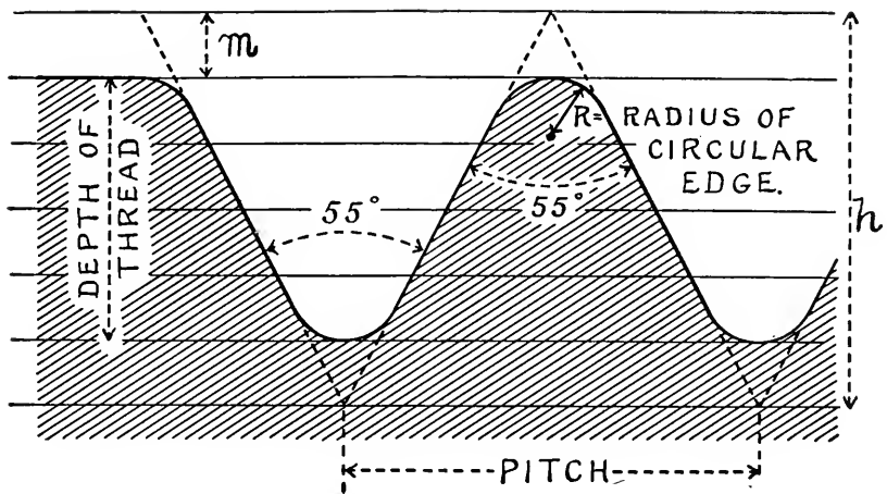
FIG. I. — THE WHITWORTH THREAD.
