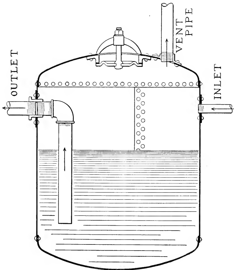
FIG. 1.—A CORRECT FORM OF BLOWOFF TANK.
