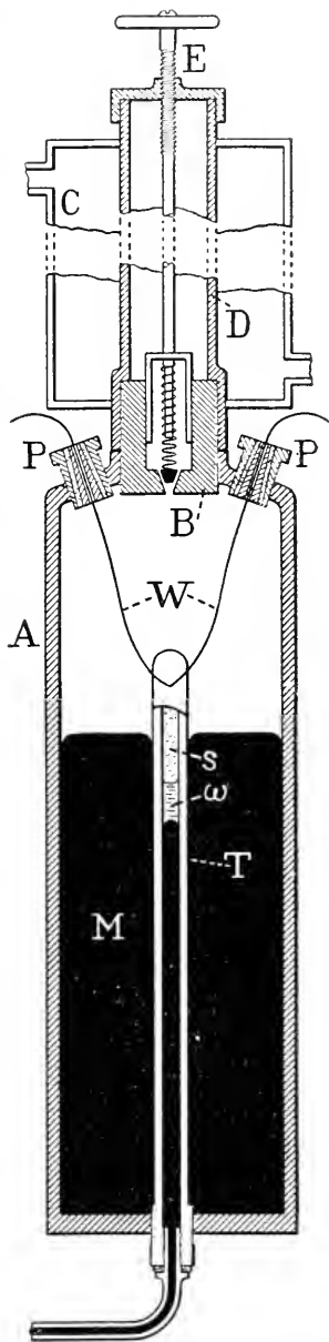
FIG. 1.—SHOWING CERTAIN DETAILS OF BATELLI'S APPARATUS.
