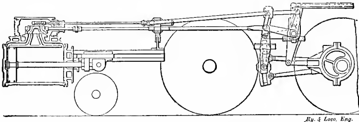
Fig. 229. David Clark's Valve Motion
