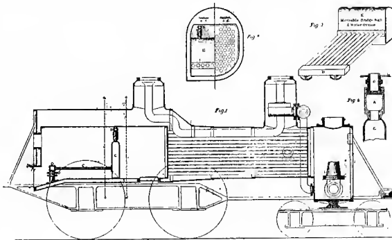
Fig. 183. Norris' Coal Burning Boiler
