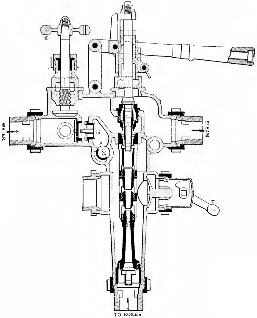
Nathan's Simplex
