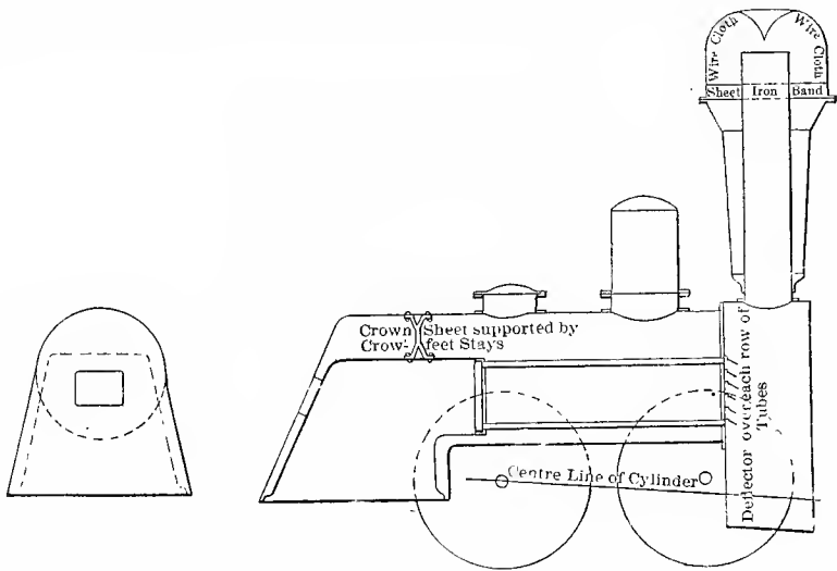
Fig. 168. Dripps Boiler, 1832
