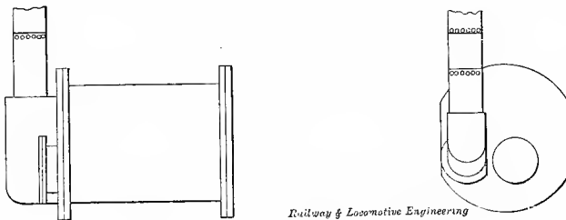
Fig. 162. Trevithick's Return Flue Boiler
