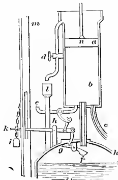
Fig. 197 Newcomen Engine, Showing Flat Admission Valve
