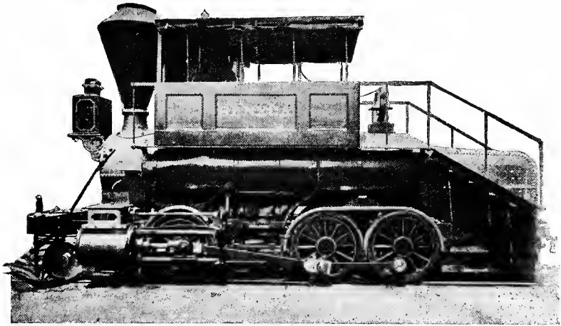
Fig. 154. Winans' Camel, Built 1856, Rebuilt 1863
