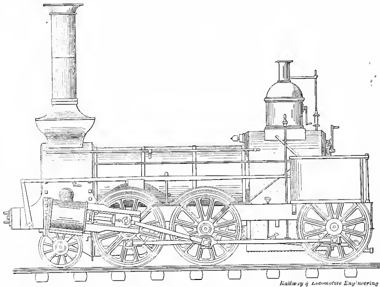
Fig. 76. First Mogul Ever Built. Made by Eastwick & Harrison, for Russia
