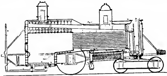
Fig. 181. Rogers' Coal Burning Boiler
