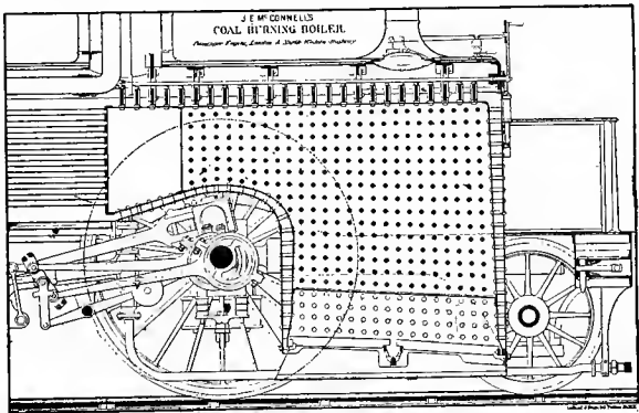
Fig. 171. McConnell's Coal Burning Fire Box
