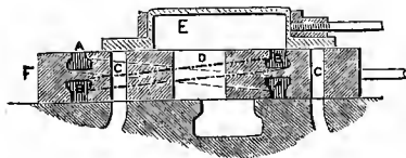
Fig. 209. Eastwick's Reversing Motion
