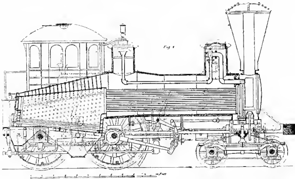
Fig. 125. Millholland's Anthracite Passenger Engine Hiawatha
