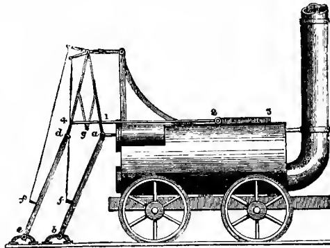
Fig. 239. Brunton's Traveller, 1813
