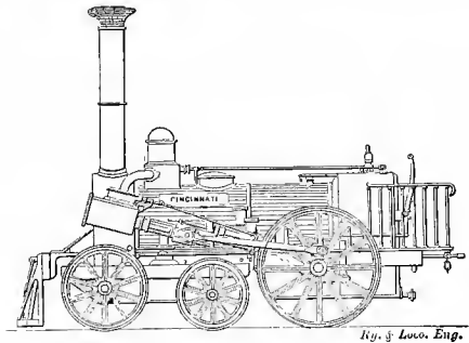
Early Niles Locomotive
