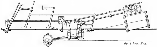
Fig. 231. Early Pennsylvania Railroad Valve Motion
