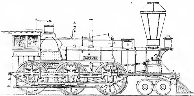
Fig. 129. Lackawanna's First Freight Engine, 1851
