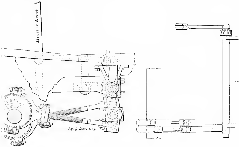
Fig. 233. Baldwin's First Link Motion in 1845
