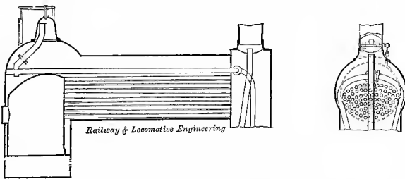
Fig. 167. Bury Boiler, 1840.
