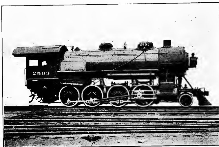
Fig. 49. Latest B. & O. Eight-Wheel Connected Engine
