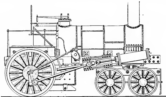
Fig. 115. "Orange," Built by Seth Boyden at Newark, 1837, for Morris & Essex Railroad
