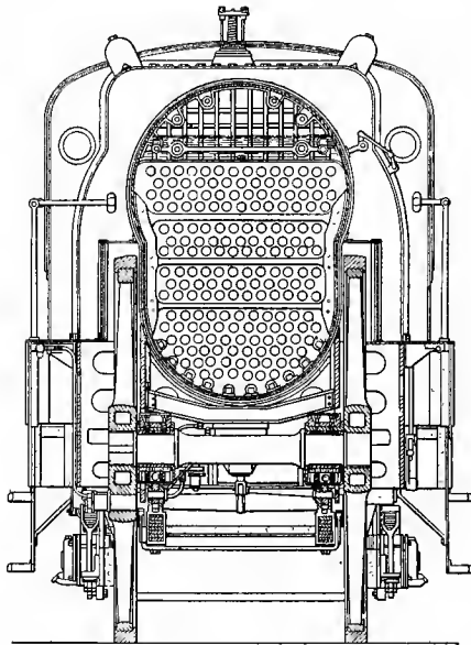
Fig. 260. Section of Boiler of the Thuille Locomotive
