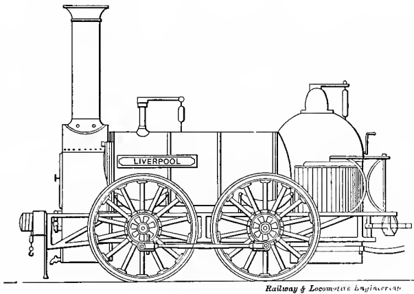
Fig. 16. Bury's Locomotive, 1834
