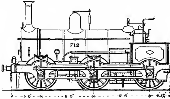
Fig. 23. Kirtley's Goods Engines
