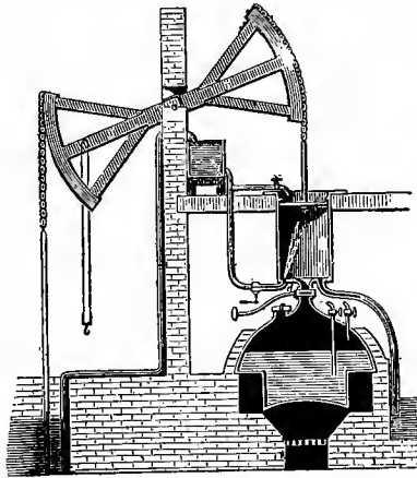
Fig. 4. Newcomen's Engine
