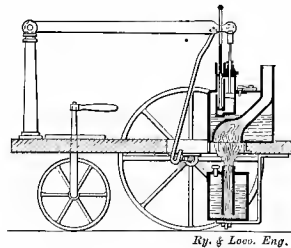
Fig. 8. Murdoch's Model
