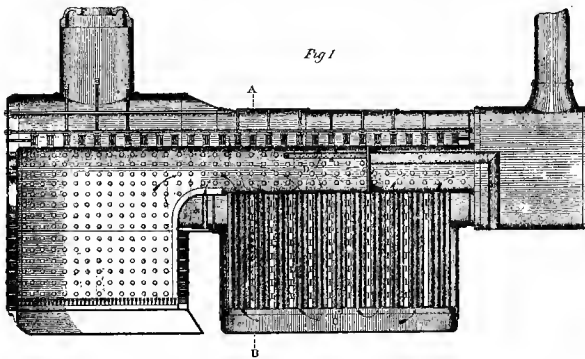
Fig. 185. Boardman's Boiler
