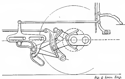
Fig. 206. Gray's Expansion Valve Gear
