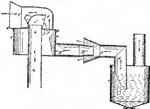
C. B. Keys—Patented June 19, 1866. Plate III.
