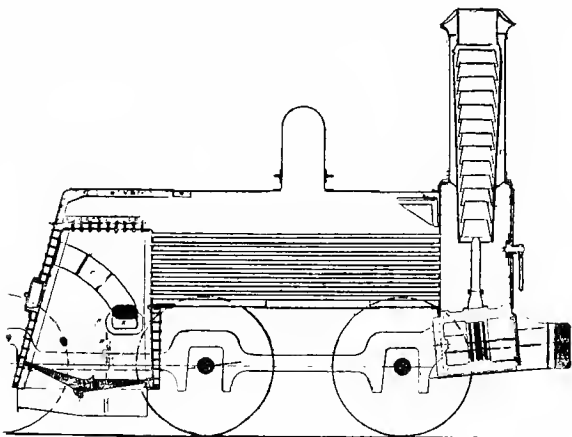
Fig. 180. Eaton's Smoke Consuming Boiler
