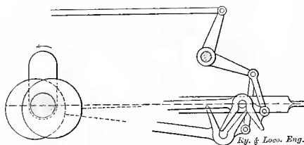
Fig. 204. Pauwel's Valve Gear
