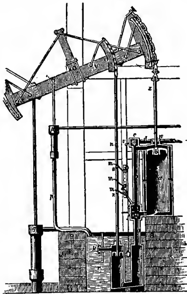
Fig. 5. Watt's Steam Engine
