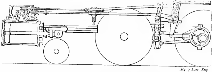
Fig. 141. Clark's Independent Cut-Off Motion
