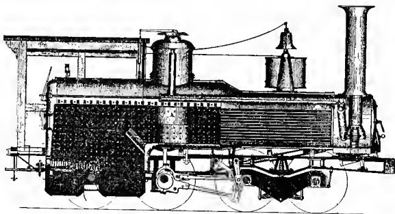
Fig. 182. Baldwin's Coal Burning Boiler
