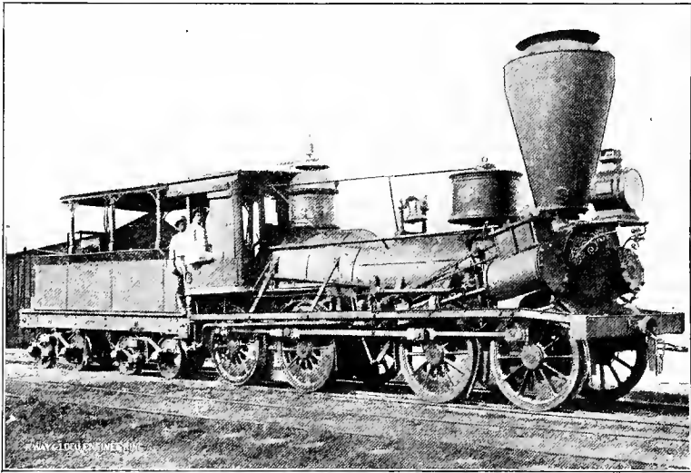
Fig. 71. Old Baldwin.
