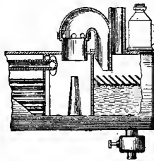
Fig. 194. To Drown Sparks
