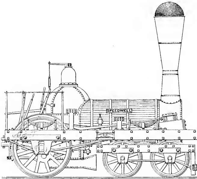
Fig. 128. Morris and Essex Third Engine, 1838
