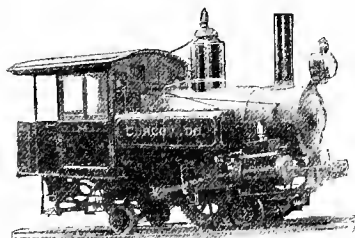
Fig. 265. Riggerbach Rack Rail Locomotive
