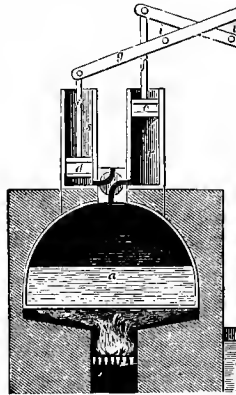
Fig. 6. Leupold's Plan of Steam Engine
