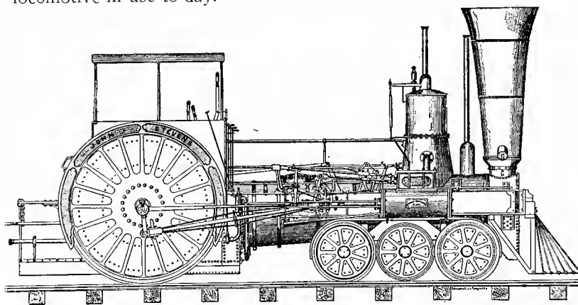
Fig. 55. The Stevens Crampton Locomotive
