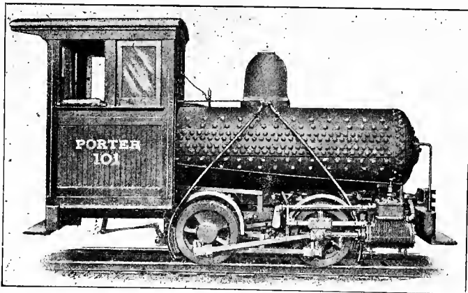
Fig. 273. Porter's Compressed Air Locomotive
