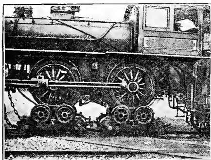
Fig. 249. Holman Locomotive
