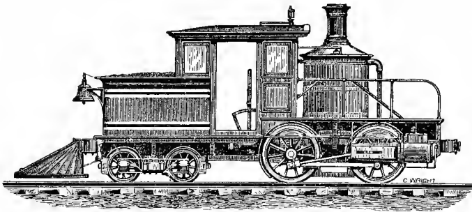
Fig. 263. First Forney Locomotive
