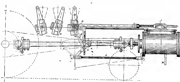
Fig. 225. Joy's Valve Motion
