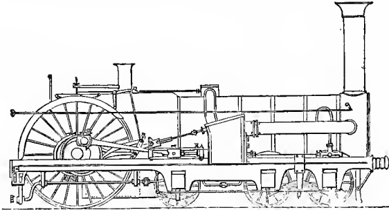
Fig. 254. Crampton's "Liverpool"
