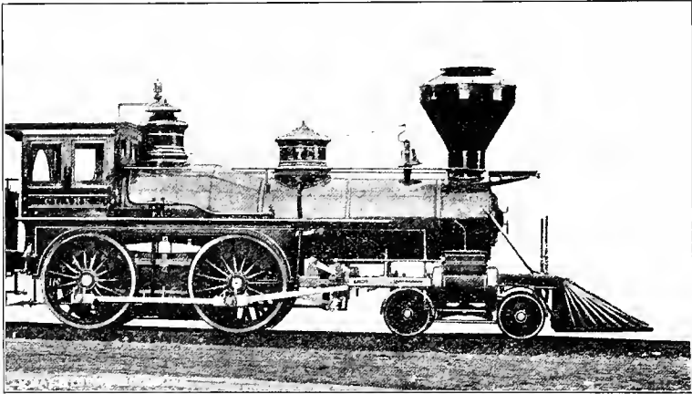
Cooke Locomotive, 1868
