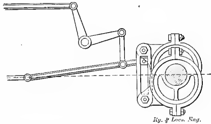
Fig. 210. Pretended Williams' Link Motion
