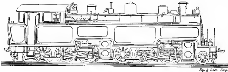
Fig. 96. Mallet Articulated Double-End Locomotive
