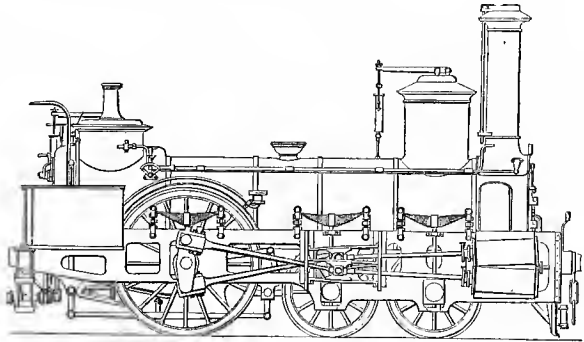
Fig. 250. "Duplex," Austria, 1861
