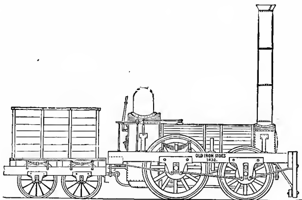
Fig 65 "Old Ironsides"
