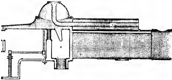
Fig. 186 Phleger's Boiler
