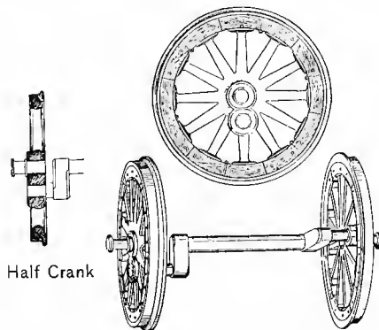
Fig. 67. Baldwin's Improved Driving Wheels
