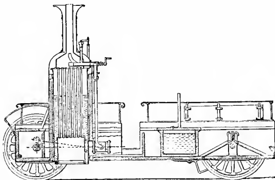
Fig. 257. Adams' Light Express Locomotive
