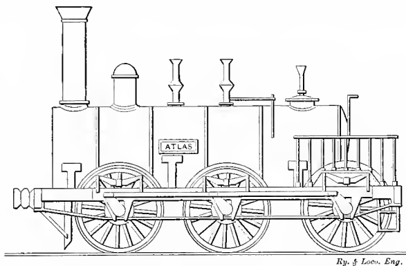
Fig. 22. Stephenson's Established Form of Goods Engine
