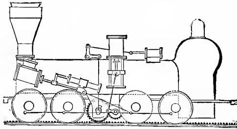
Fig. 68 Geared Locomotive
