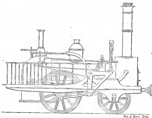
Fig. 242. Roberts' Experiment, 1833
