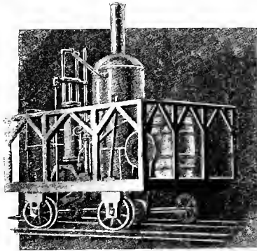
Fig. 36. Cooper's Tom Thumb
