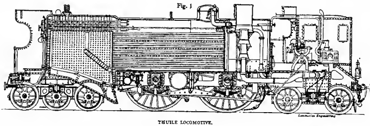
Fig. 259. Thuile Locomotive
