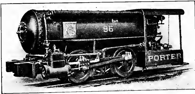
Fig. 272. Porter's Single Truck Compressed Air Locomotive
