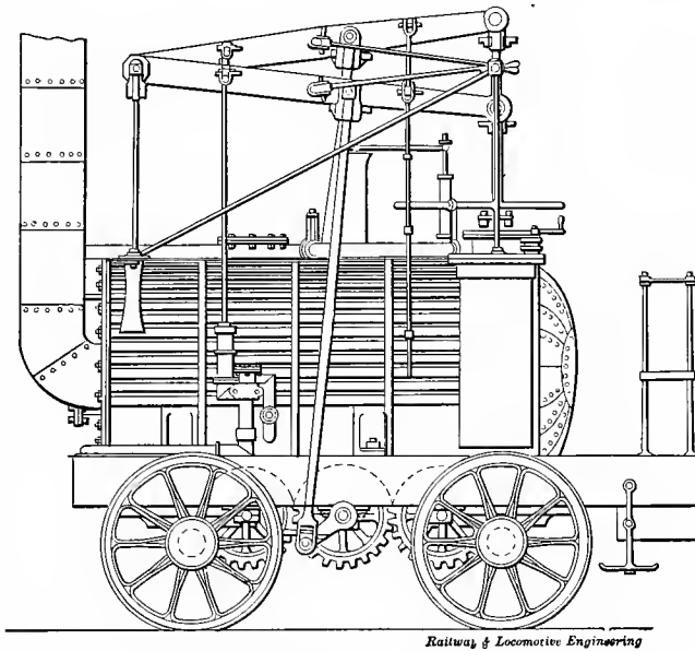
Fig. 12. Hedley's "Puffing Billy," 1813. First Locomotive Used Commercially in Hauling Cars
