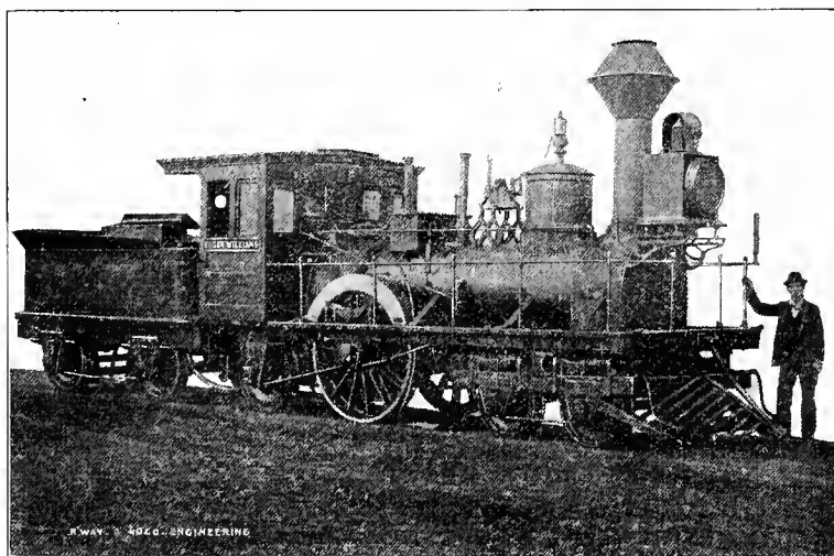
Fig. 86. Lowell Engine, Built About 1837, Rebuilt 1846, Belonged to Stonington Railroad. James M. Anderson, Master Mechanic of Road, in Front
