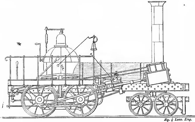
Fig. 73. Garrett & Eastwick's Locomotive Hercules
