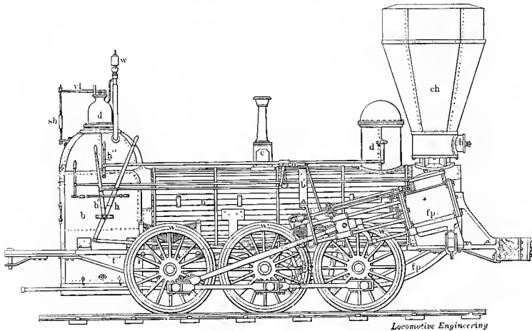
Fig. 122. Millholland's Philadelphia
