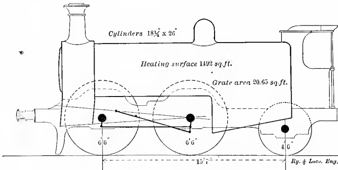
Fig. 24. Strondley's Gladstone Class
