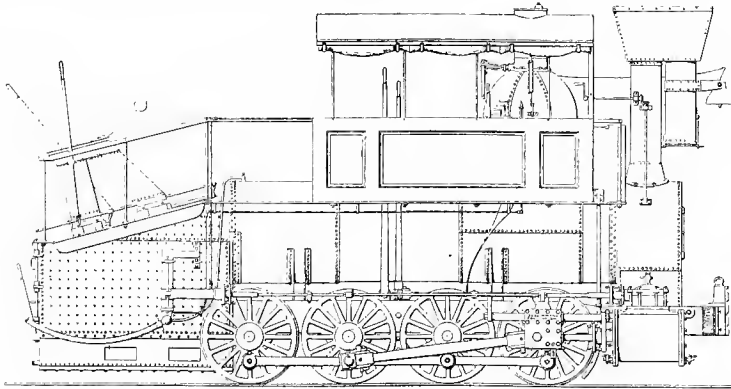
Fig. 131. Ross Winans Carbon for Lackawanna, 1854
