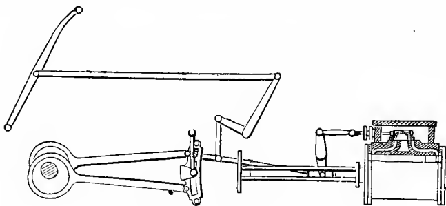
Fig. 222. Rogers' Suspended Link Motion
