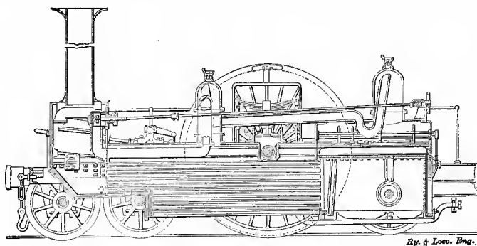
Fig. 253. Trevithick's "Cornwall," 1847
