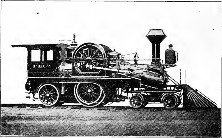
Fig. 248. Fontaine Locomotive
