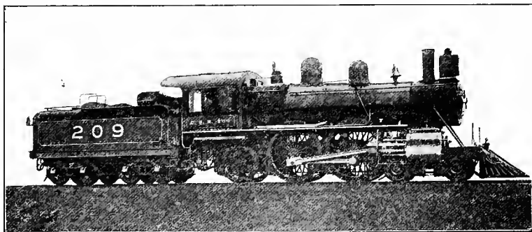
Modern Vaucrain 4-Cylinder Compound Passenger 4-4-2 Engine, Built at Canadian Pacific Shops, Montreal, in 1898. Cylinders, 13½ and 23 x 26 Inches; Drivers 84 Inches; Weight of Engine, 170,250 Pounds
