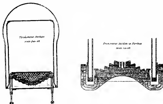
Fig. 177. Jeffrey's Coal Burning Step Gate
