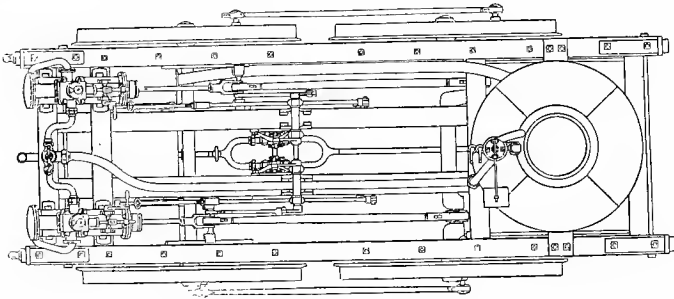
Fig. 31. Plan of the "Best Friend"
