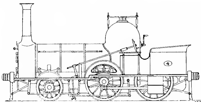
Fig. 259. Rebuilt Bury Locomotive
