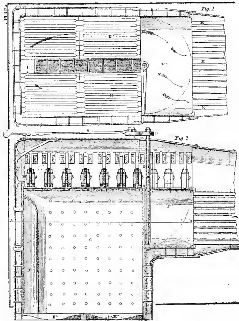
Fig. 179. Head's Fire Box
