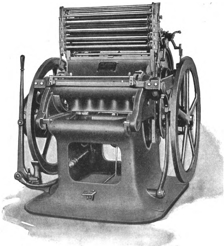
FIG. 136.—John Thomson Press, Model J.
