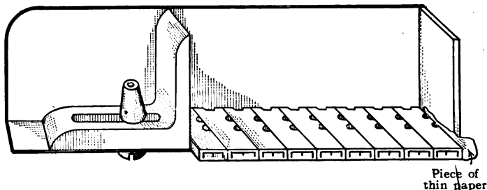
FIG. 9.—Proper Method of Making up a Non-graduated Composing-stick.
