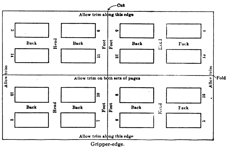
FIG. 105.—Diagram Showing Various Parts of a Form.
