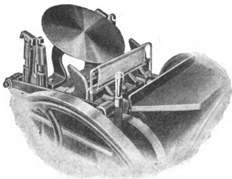
FIG. 148.—Sylvester Safety Device for Job Presses.
