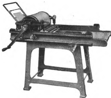
FIG. 23.—The Vandercook Proof-press.
