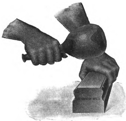
FIG. 18.—Method of Holding and Tapping a Form-planer.
