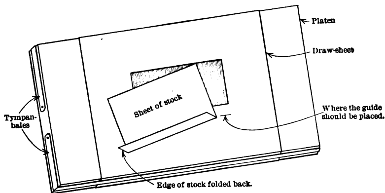
FIG. 138.—Setting Guides.
