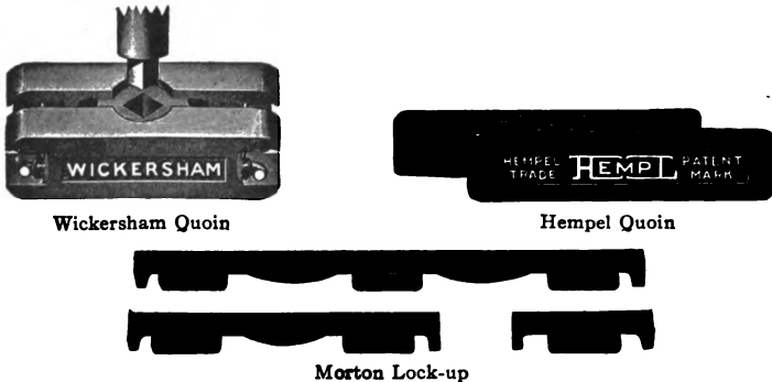
FIG. 95.—Some Standard Forms of Iron Quoins.
