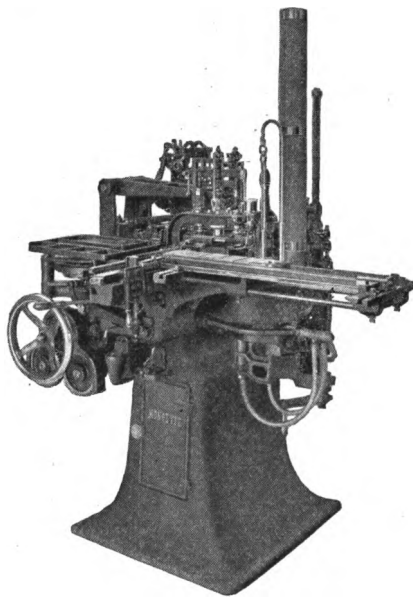
FIG. 129.—Monotype Casting-machine.
