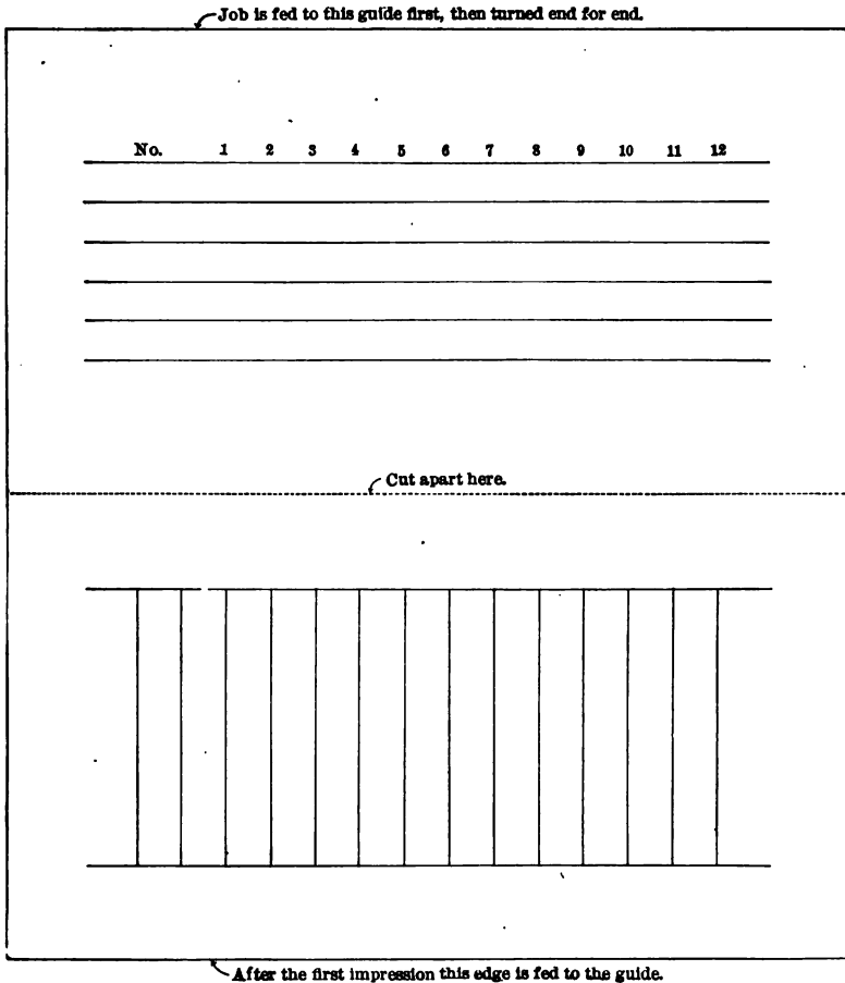
FIG. 98.—Showing Lock-up of a Rule Form in Two Sections, to be Printed at One Time. When the sheet is turned end for end the two sections will overlap, thus producing two copies.
