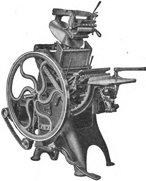
FIG. 134.—Golding Jobber.
