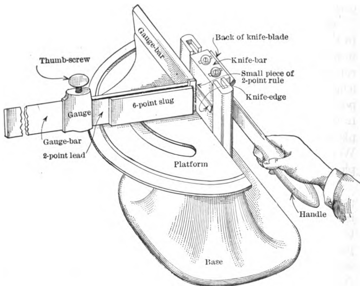
FIG. 124.—Dressing up a Small Piece of Rule on a Mitering-Machine.
