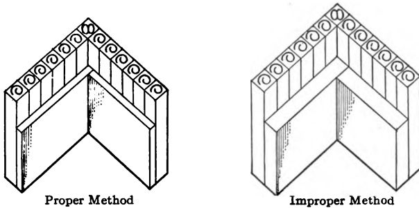
FIG. 53.—Proper and Improper Method of Placing Slugs inside of Border Units.
