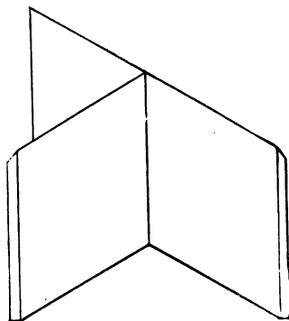
FIG. 47.—Showing How Three-point Side-face Rule Should be Butted to Make a Perfect Joint.
