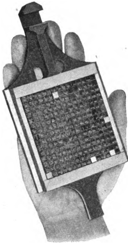
FIG. 130.—Monotype Matrix-case.
