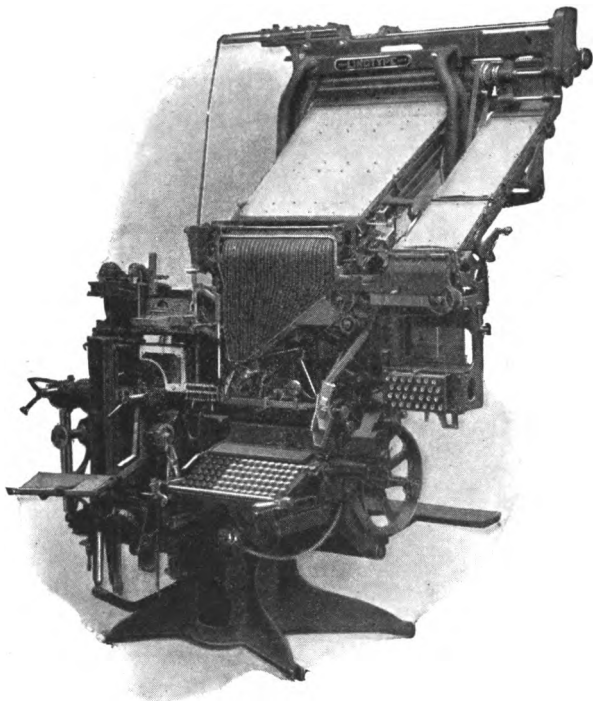
FIG. 127.—Linotype No. 17.
