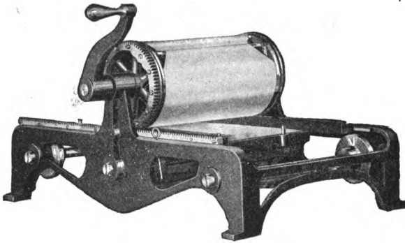
FIG. 21.—The Poco Proof-press.
