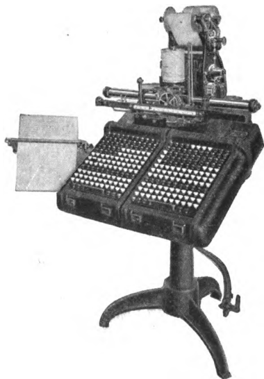
FIG. 128.—Monotype Keyboard.
