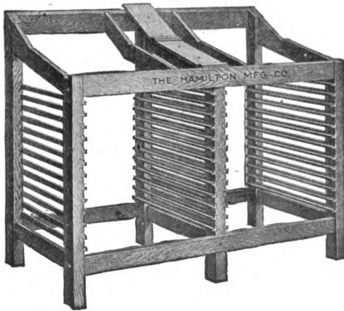
Old Style of Composing-frame.
