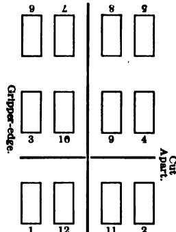
FIG. 111.—Twelve Pages Worked as an Eight and a Four, the Eight to Inset the Four.
