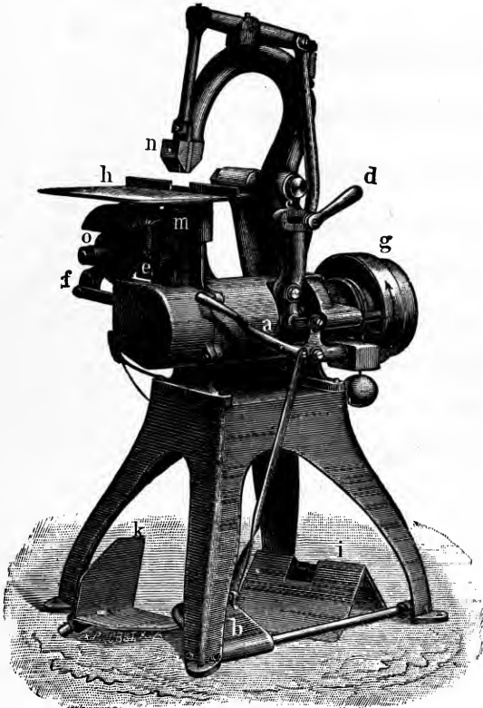
THE SUCCESS—NO. 7½—FOR STEAM POWER.
