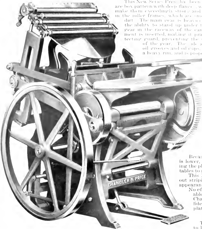
Three Quarter View of 11 1 / 2 x22 New Series Chandler & Price Press
