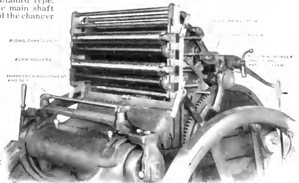
Laureate Models J and T Detailed view from the front and right-hand side. This shows the carriage when provided with the two riding changers, and also the lath for causing all the form rollers to pass during the up-movement, free of the form. The inking apparatus is the same in both models.
