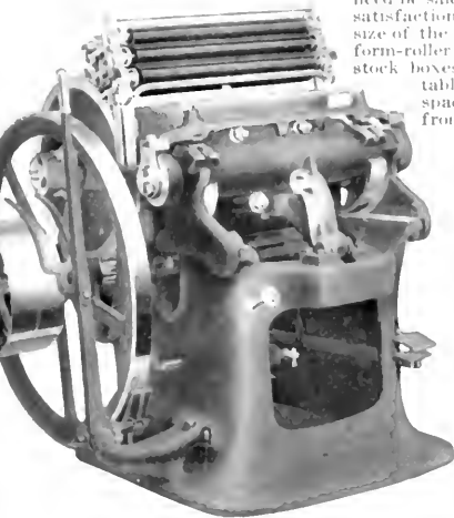
Colt's Armory, Style 2-A. Made in two sizes: Half Medium, 13x19 inches, and Half Super Royal, 14x22 inches (inside chase measurements).
