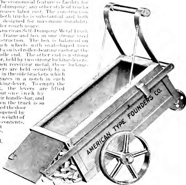
American Self-Dumping Metal Truck No. 551
