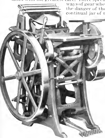
Three Quarter View of an 8x12 New Series Chandler & Price Press
