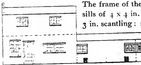
Fig. 12. Elevation of Front of Two Story Building and Part of Long Building in Fig. 11.
