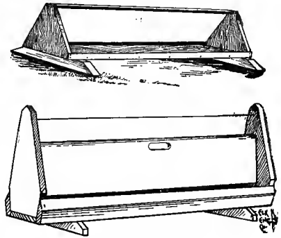
Fig. 41. Feed Troughs.
