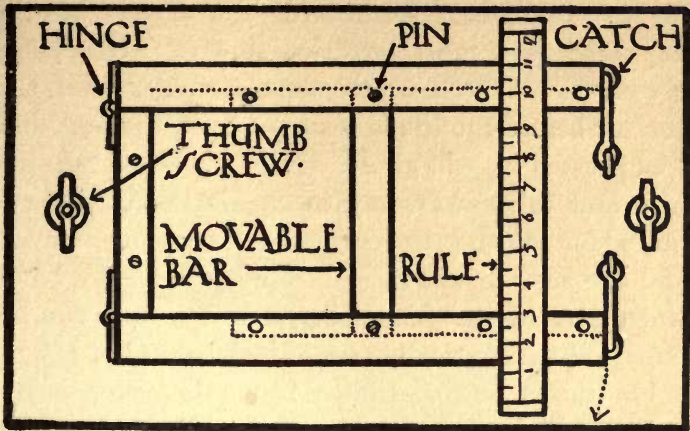
TILE FRAME - 6\frac{1}{2} \times 13 -
