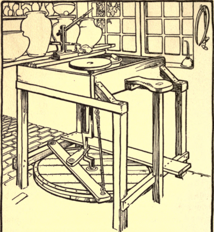
THE KICK WHEEL.
