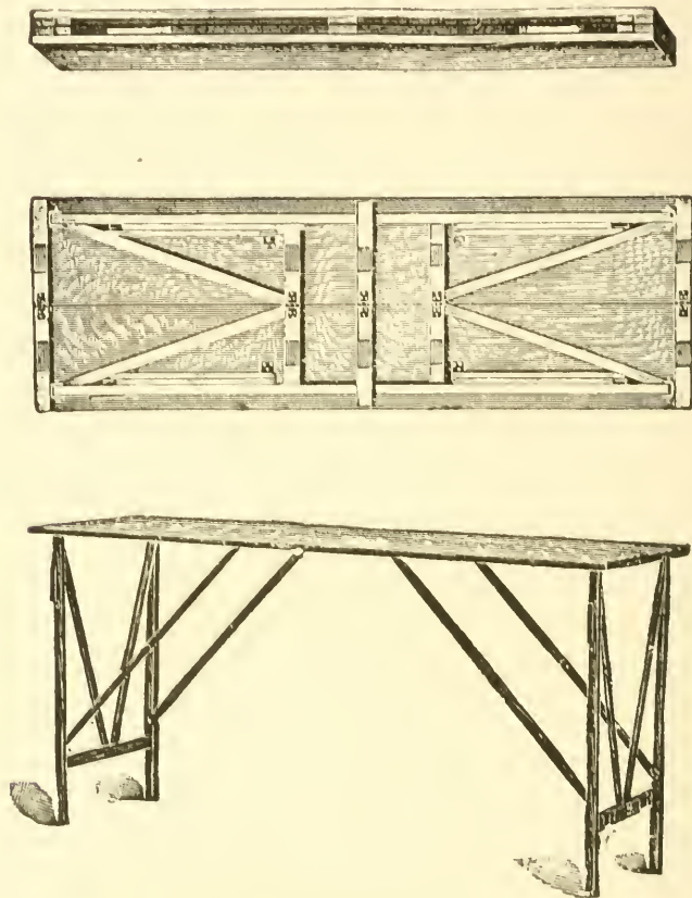
Fig. 48. Paperhanger's Table.
