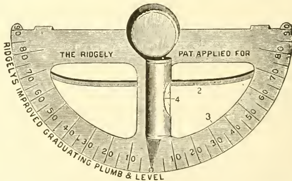
Fig. 46. Graduating Plumb and Level.
