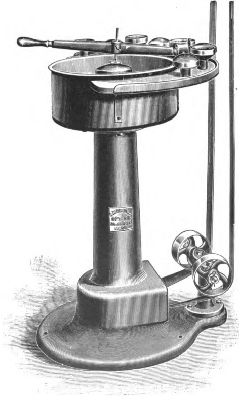
OPTICIAN'S LATHE FOR GRINDING SPHERICAL LENSES.
