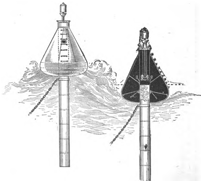
COURTENAY'S WHISTLING-BUOY.
