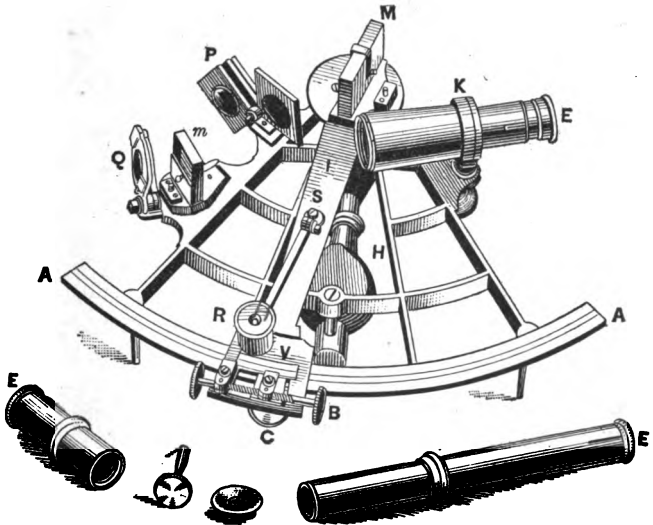
THE SEXTANT.
