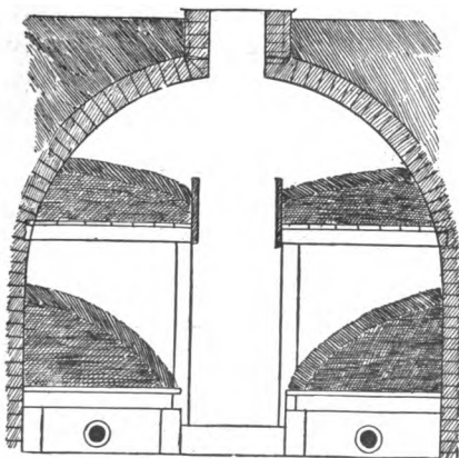
FIG. 3. CROSS-SECTION OF THE DOSORIS MUSHROOM CELLAR.
