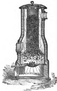
FIG. 6. VERTICAL SECTION.
