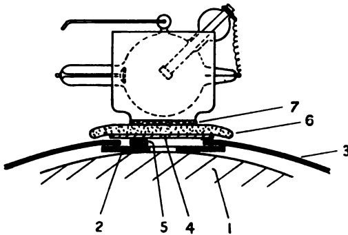
FIG. 361.—Arrangement of the tube and filters.
