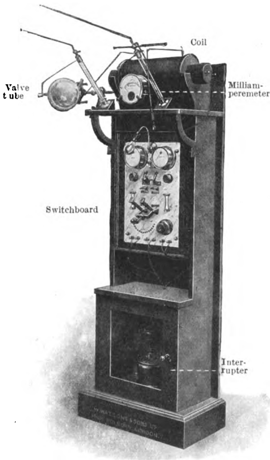
FIG. 339.—Apparatus arranged on an upright cabinet. (Watson & Sons.)
