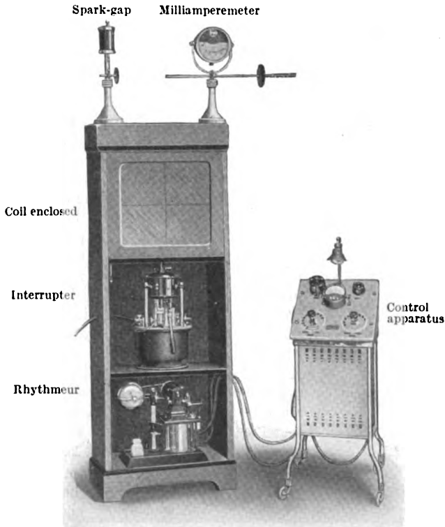
FIG. 326.—Therapeutic outfit suitable for deep therapy. (Schall.)
