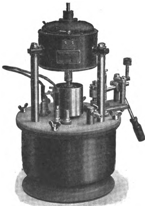
FIG. 327.—Mercury interrupter with gas di-electric. (Schall.)
