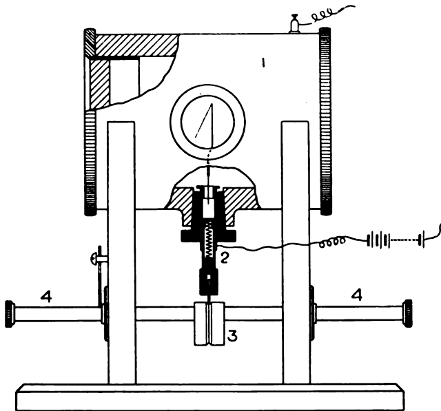
FIG. 362.—Special form of gold leaf electroscope. (For description see p. 493.)
