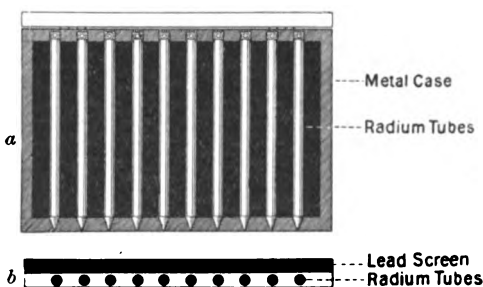
FIG. 374.—A flat applicator for radium. a , Front view. b , Sectional view.
