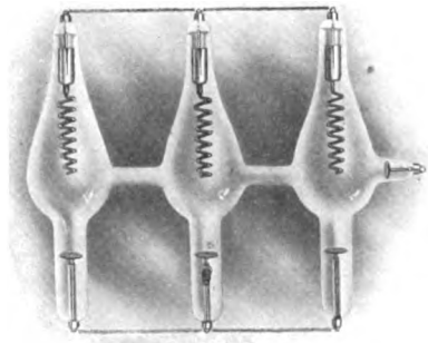
FIG. 332.—Triple valve tube. (C. Andrews.)
