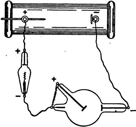
FIG. 333.—Method of connecting coil to valve tube and X-ray tube. Valve tube on positive pole. (Siemens.)
