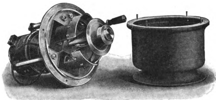
FIG. 328.—Mercury interrupter, showing details.
