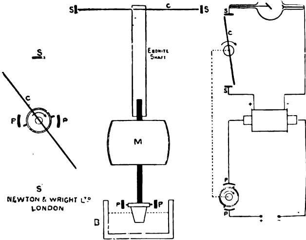
FIG. 331.—Diagram of connections for Morton rectifier.
