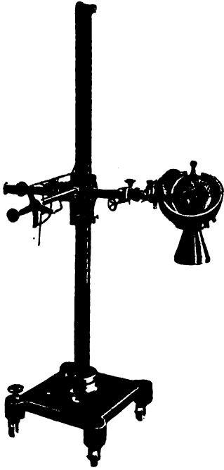
FIG. 336.—Pillar tube stand suitable for therapeutic work. (A. Gaiffé.)
