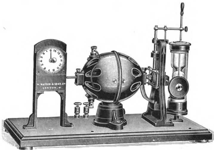
FIG. 329.—Dipping interrupter, with revolution counter, or tachymeter.
