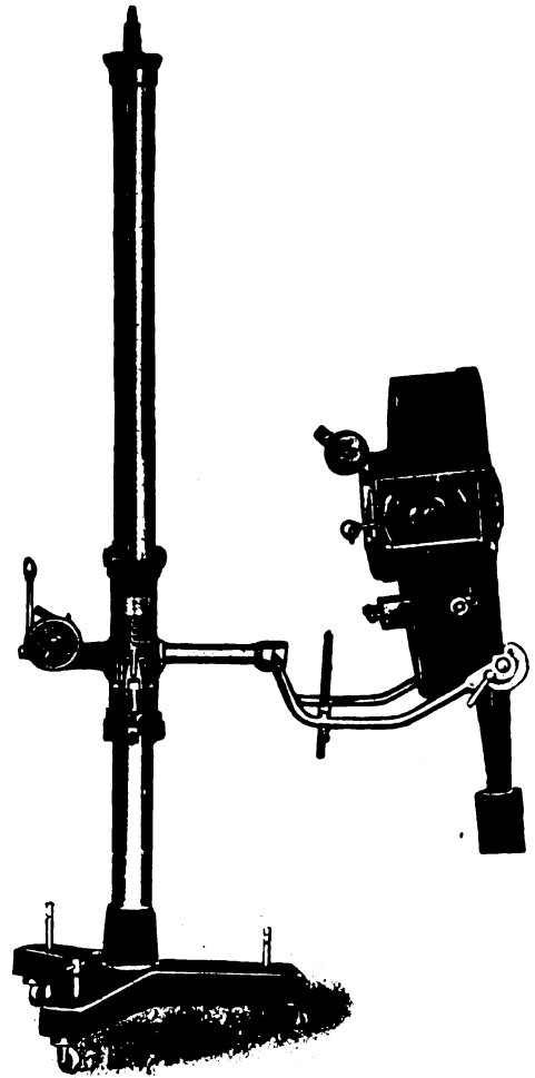
FIG. 335.—Tube stand for deep therapeutic work. (Schall.)
