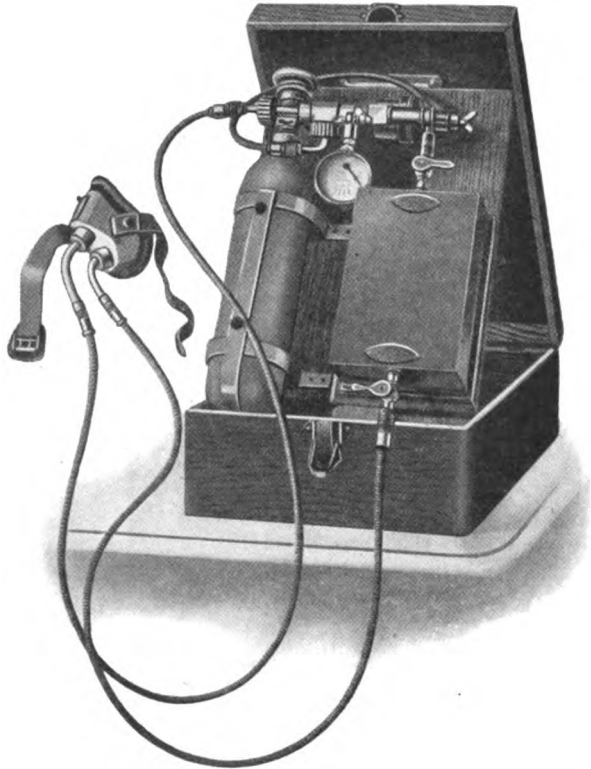
FIG. 370.—Apparatus for inhalation of radium emanation and oxygen. (Radium, Limited.)
