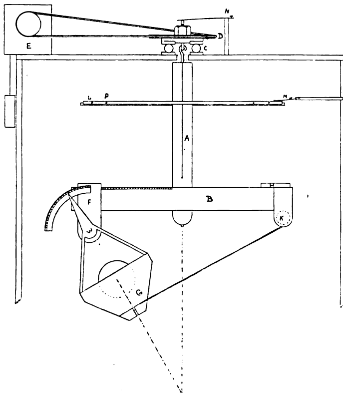
FIG. 337.—Rotating tube stand.
