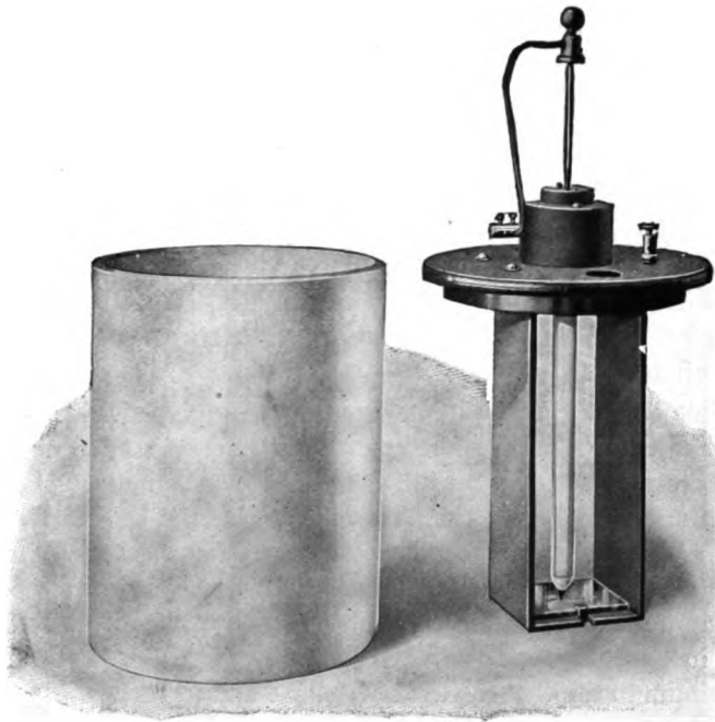
Fig. 79. Self-adjusting electrolytic interrupter.
