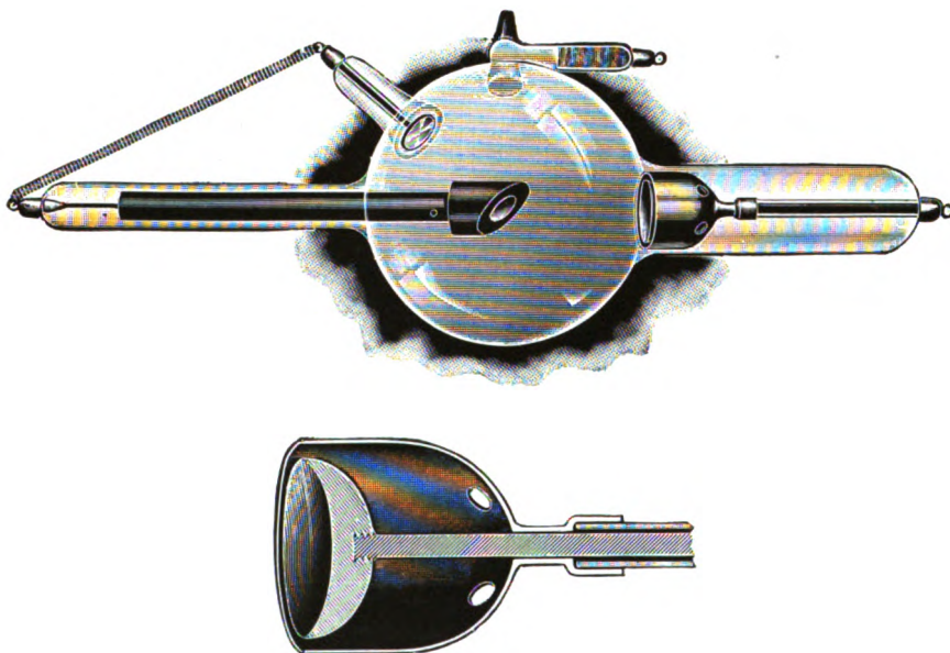
Figure 368.—X-ray tube with protection cathode collar.
