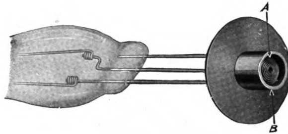
Figure 365.—Cathode of Coolidge tube.
