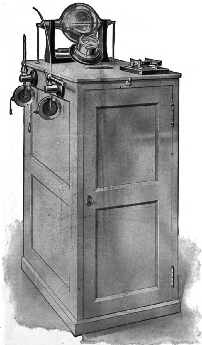
Figure 357.—Special dental X-ray machine. Induction coil type. Size: 15 inches wide, 28 inches deep, 36 inches high.
