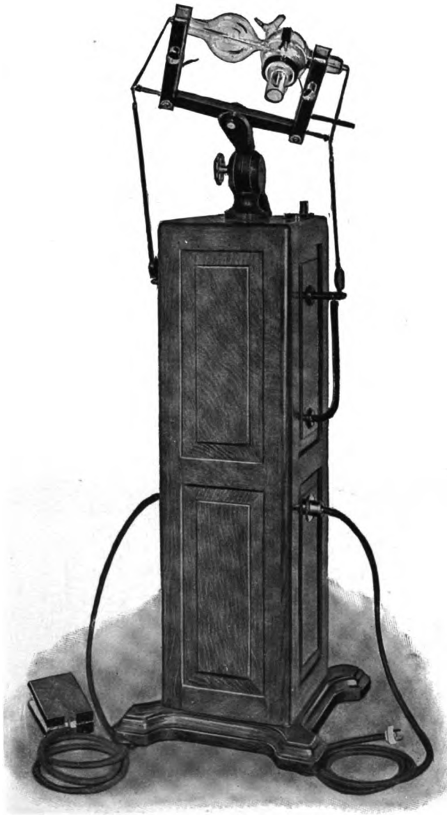
Figure 363.—Dental X-ray "Unit." Size: 18 inches wide, 18 inches deep, 46 inches high.
