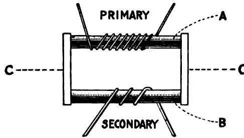
Fig. 10. Diagram of a step-down transformer.
