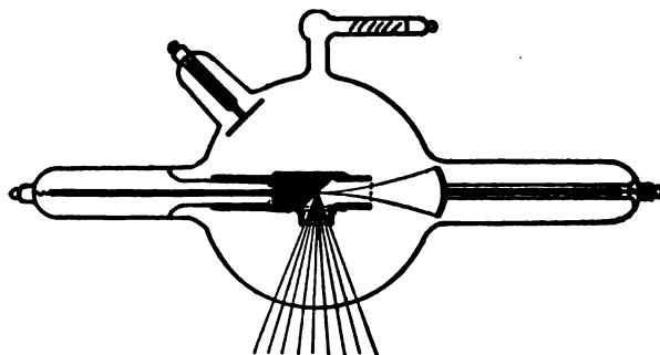
Fig. 319. Protection or safety, X-ray tube.
