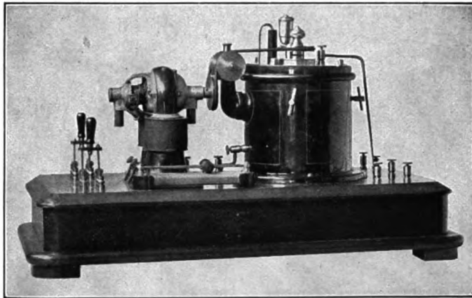
Fig. 21. Mercury turbine interrupter.
