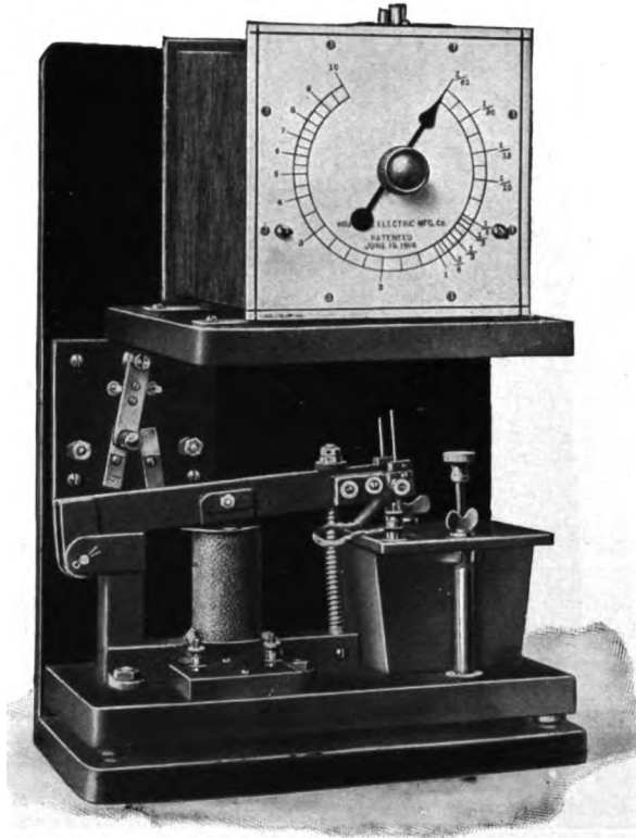
Fig. 116. Automatic time switch or "timer," by means of which seconds may be split.
