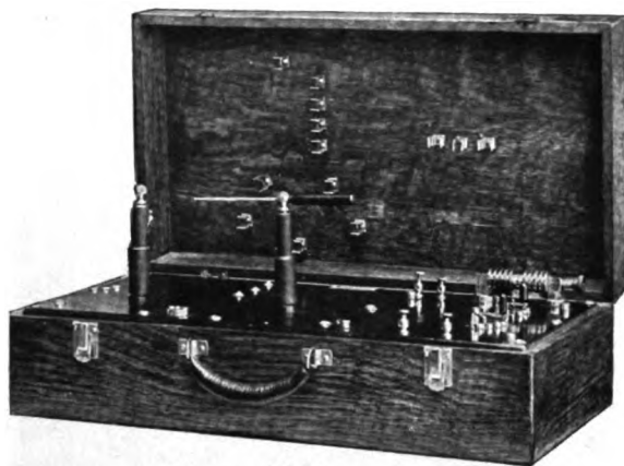
Fig. 14. High-frequency coil.
