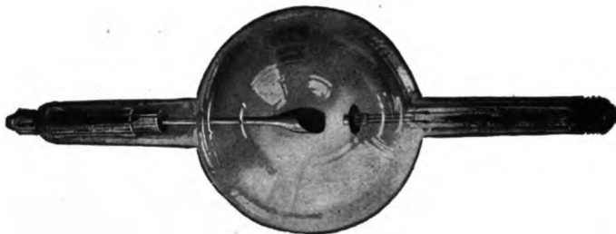
Figure 364.—Coolidge X-ray tube.
