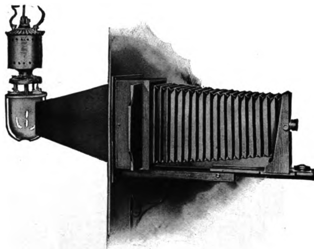
Fig. 471. Enlarging apparatus.
