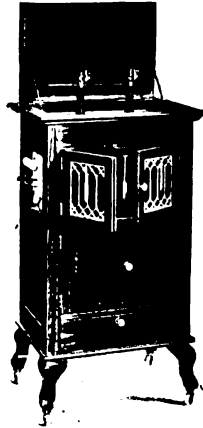
Figure 360.—X-ray and electrotherapeutic machine. High-frequency type. Size: 24 inches wide, 18 inches deep, 48 inches high.
