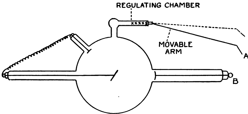
Fig. 44. X-ray tube with vacuum regulator.
