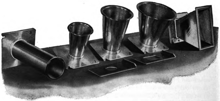
Fig. 328. Compression cones, cylinder and square, and diaphragms for same.
