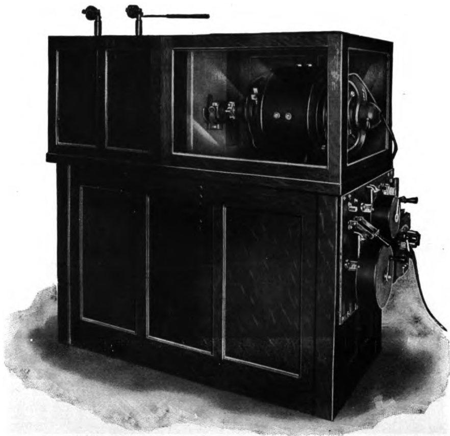
Fig. 15. Interrupterless coil.
