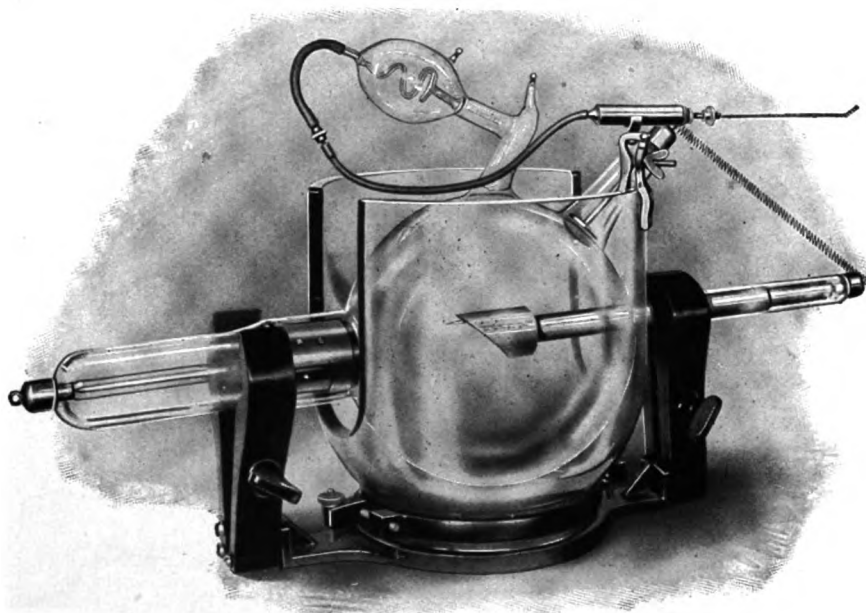
Figure 371.—Hydrogen X-ray tube.
