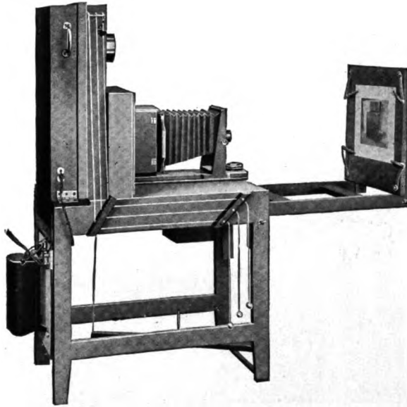
Fig. 472. Enlarging apparatus.
