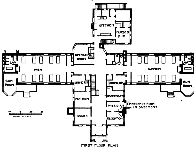
FIRST FLOOR PLAN Arnot-Ogden Memorial Hospital, Elmira, N. Y.
