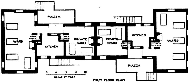
Contagious Disease Ward, Cambridge Hospital.
