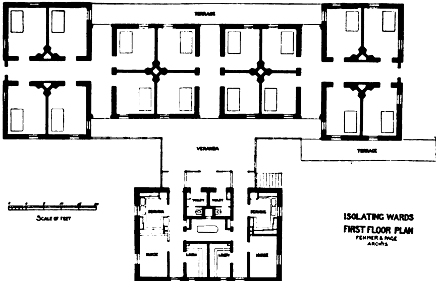
Isolation Ward, Massachusetts General Hospital.
