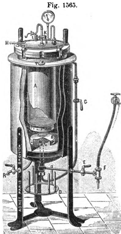
Sorel's Sterilizer for Dressings.
