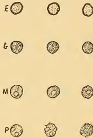
FIG. 48.—PUS-CORPUSCLES SHOWING DIFFERENT CONSTITUTIONS ( \times 500 ). E , Excellent; G , good; M , medium; P , poor.
