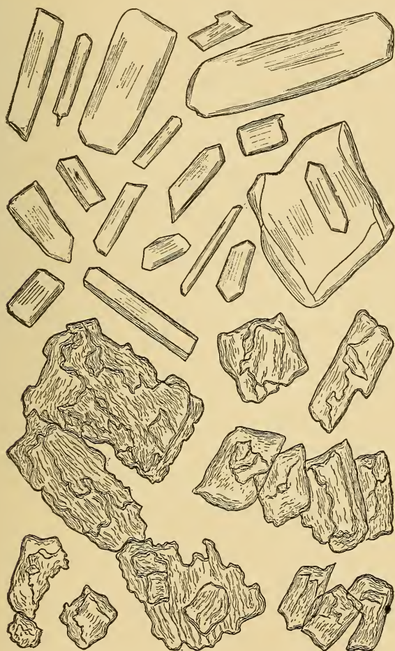
FIG. 8.—CRYSTALS OF UREA (UPPER HALF) AND NITRATE OF UREA (LOWER HALF) ( \times 200 ).
