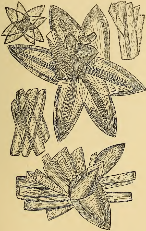
FIG. 20.—CRYSTALS OF URIC ACID, COMMON FORM ( \times 400 ).
