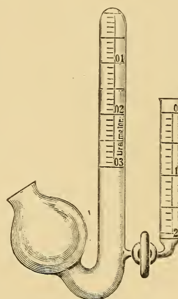
FIG. 10.—HINDS' MODIFICATION OF DOREMUS' UREOMETER.
