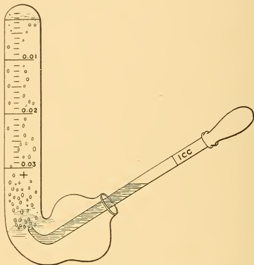
FIG. 9.—DOREMUS' UREOMETER.
