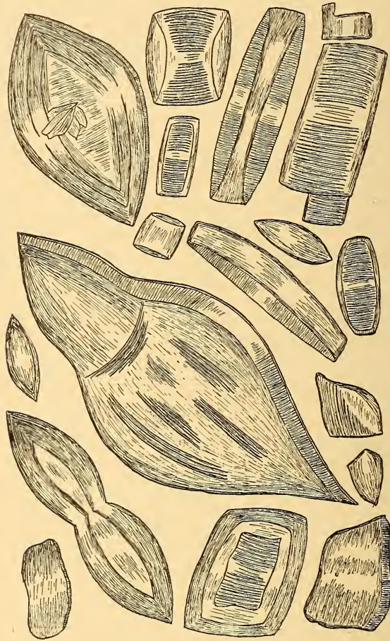
FIG. 19.—CRYSTALS OF URIC ACID, COMMON FORM ( \times 400 ).
