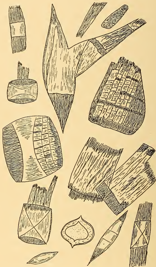
FIG. 21.—CRYSTALS OF URIC ACID, FROM HIGHLY ACID URINE ( \times 450 ).
